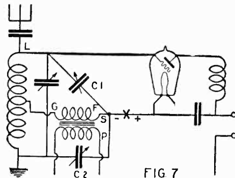
FIG. 7 Another type of reflex circuit is shown in Fig. 7. The Wheatstone Bridge principle is used here.
