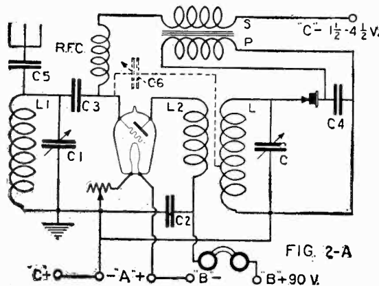
FIG. 2A shows a 1-tube reflex, the outstanding feature of which lies in the shunt feeding of the audio frequency energy into the radio frequency amplifying tube. If it is desired to use a tube detector in preference to a crystal, then connections should be made as in Fig. 2B.
