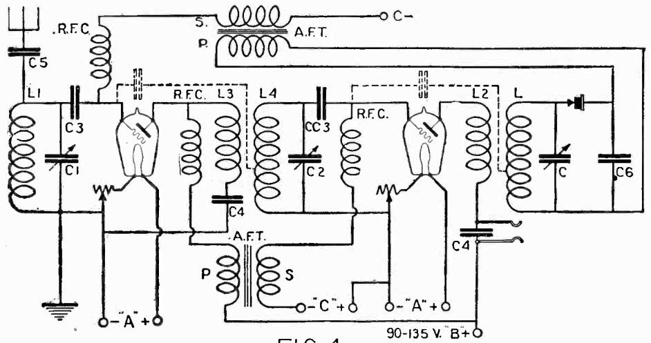
FIG. 4 This circuit, while more complicated than the one shown in Fig. 2A, gives an amplification equivalent to four tubes, the crystal acting as a detector. There are two stages of R.F. and two stages of A.F. If neutralized, the hook-up becomes equivalent to a five tube Neutrodyne.
