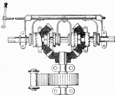
Above is a diagrammatic view of gears and clutch mechanisms of the device at the right.
