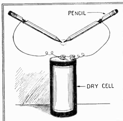
A simple arc lamp; pencil leads are the electrodes and the pencils can be held in the hand as the wood cuts off the heat.
