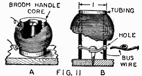
FIG. 11 The R.F. chokes are jumble-wound to minimize distributed capacity. Two winding forms are shown.
