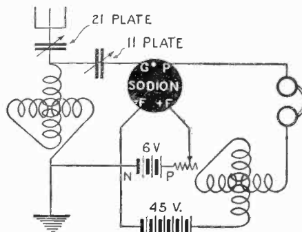
An experimental hook-up using the sodion detector.
