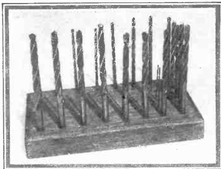
Drills may be kept handy if held in a drill stand. This may be easily made out of a block of wood 7/8"x3"x5", using each drill to make its own hole. Beside each hole stamp into the wood the number of the drill. Shellac or varnish the stand.
