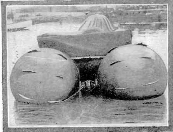
↑ The picture above shows rear view of the three-balled water velocipede, the differential gear of a small automobile driving the two rubber covered rear spheres, the surface of these spheres being provided with vanes in order to afford propulsion. The balls may be made from metal or wood framework covered with heavy rubberized cloth.
