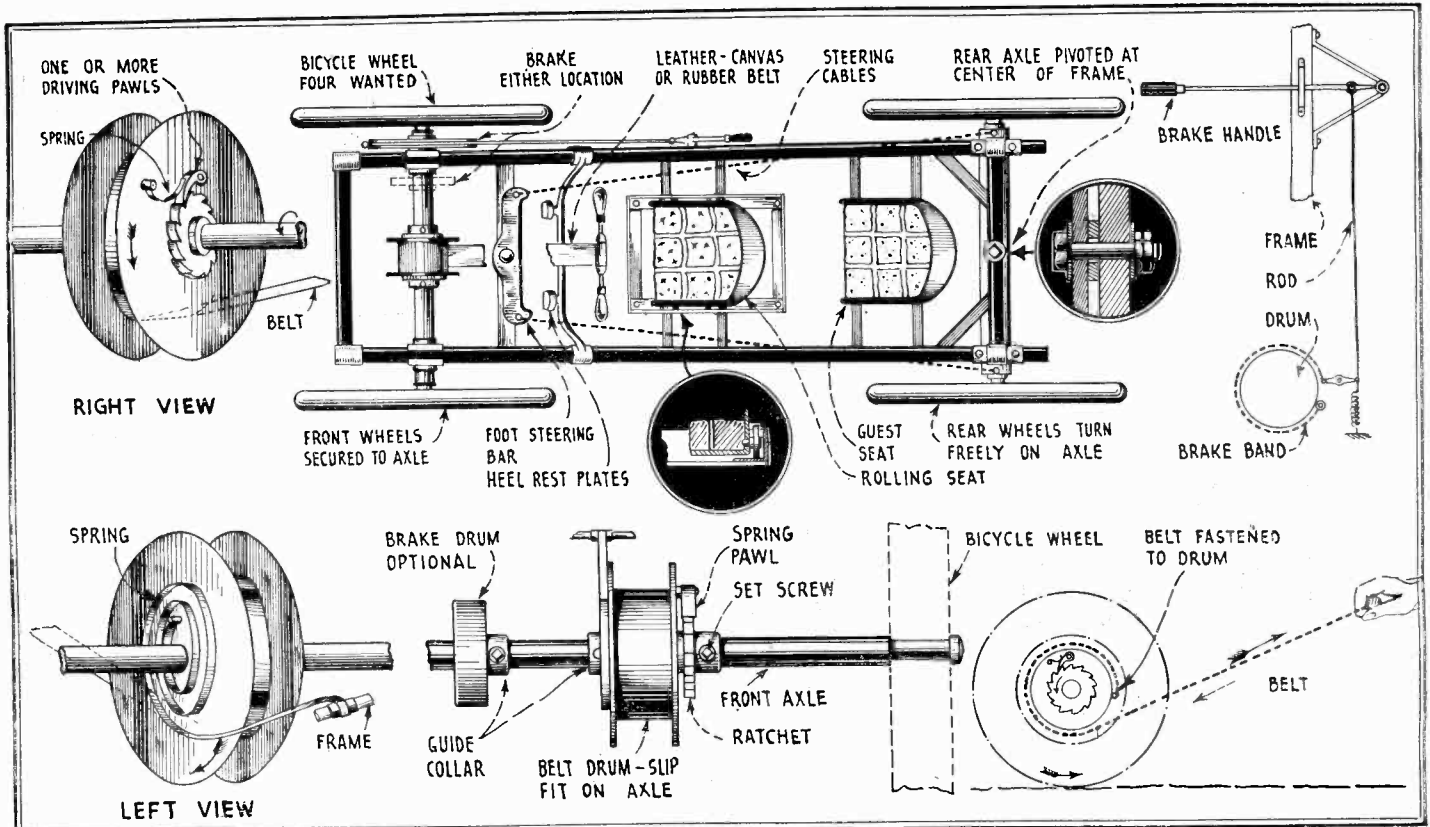
pawls rotate the ratchet, which is rigidly secured to the front driving axle. Then the spiral spring retracts the belt, and the pawls slip over the teeth of the ratchet wheel freely, without exerting power on the axle.
