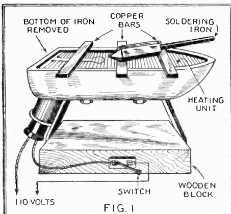
A flat iron, inverted, with the coil exposed, is a convenient heater for a soldering iron or for light cooking, heating glue and similar purposes.
