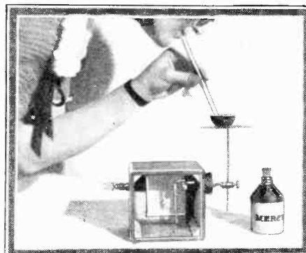
No, this is not a soda fountain but a little electrical generator. Blowing the breath through mercury agitates it, thus creating an electrical potential as indicated by the electroscope.
