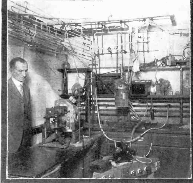
X-ray and other apparatus in laboratory where illinium was first produced.
