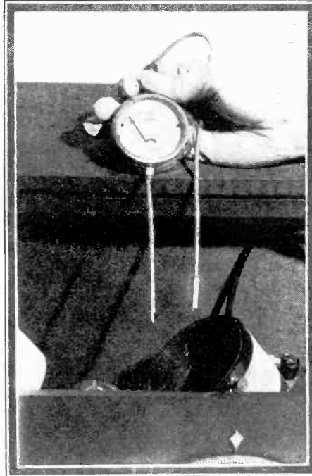
Convenient extension leads for the pocket voltmeter are made by soldering two pieces of bus bar, one to the meter case and one to the end of the flexible terminal. The bus bar is covered with spaghetti almost to the extreme tip.
