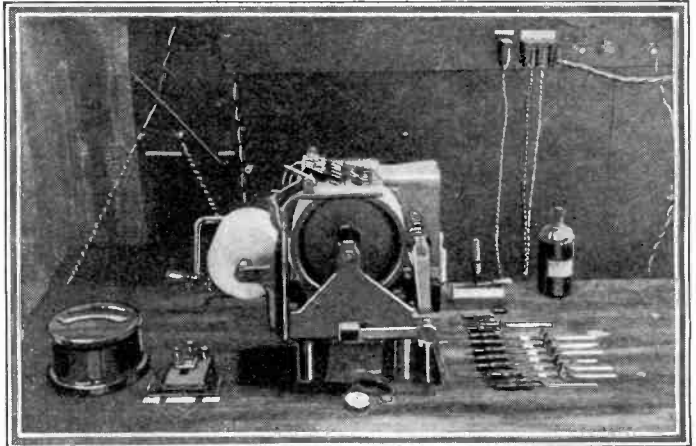
Photo above shows electric chronograph apparatus which records the time elapsing between dropping the bomb and the moment of explosion.
