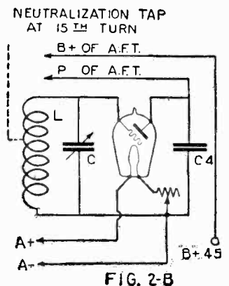
FIG. 2A shows a 1-tube reflex, the outstanding feature of which lies in the shunt feeding of the audio frequency energy into the radio frequency amplifying tube. If it is desired to use a tube detector in preference to a crystal, then connections should be made as in Fig. 2B.
