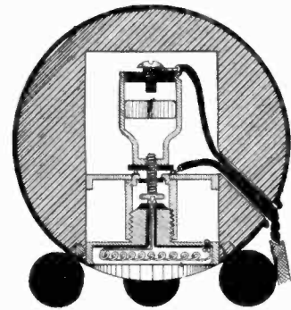
This electric cigar lighter turns on automatically when inverted. A small weight slides down, making contact with a screw. The jams. Courtesy Aldredge Company
