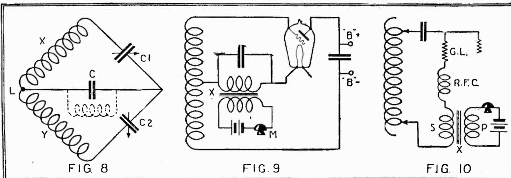
FIG. 8 FIG. 9 FIG. 10 The hook-up shown in Fig. 7 is indicated in its equivalent ideographic form in Fig. 8. C1 and C2 are midget condensers forming the arms of a Wheatstone Bridge and are used for balancing the radio frequency currents out of the audio frequency transformer, the distributed capacity of which is represented by the condenser C (the secondary winding being indicated by the dotted inductance across C.) This method effectively prevents undesirable feed-back. Figs. 8 and 9 show the equivalent transmitting circuits which tend to introduce distortion in a reflex set because of the occurrence of modulation. The similarity between these circuits and the normal reflex arrangement is immediately obvious.
