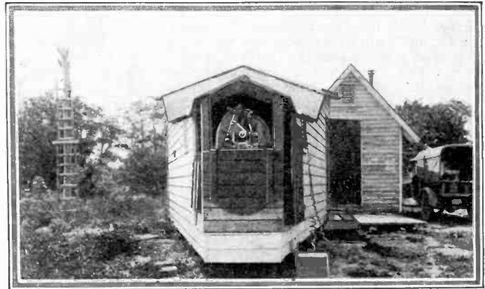
Photo above shows end view of camera house in which specially devised cameras photograph both horizontal and vertical views of bombing plane and bomb. That data is used in studying fall of bombs.
