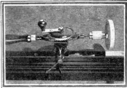
A strip of sandpaper glued or tacked on the periphery of a wooden disk held in the chuck of a hand drill makes a good sand wheel.
