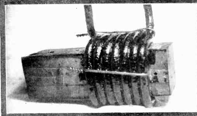
The upper left-hand illustration shows a coil of the welding transformer with four terminals to give two steps of transformation. The lower left hand cut shows the use of a wooden form for winding the coils. The other illustration on the right shows the transformer fully mounted.
