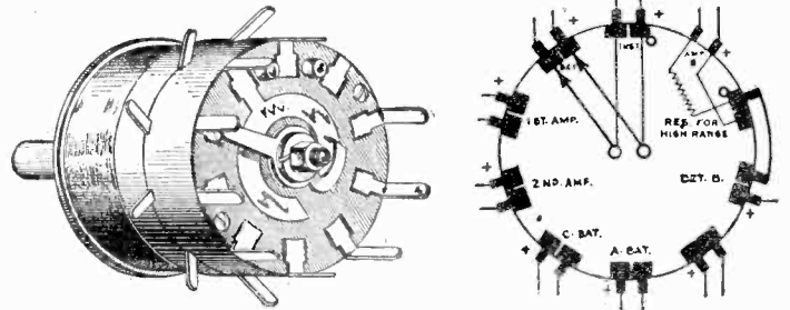
A rear view of the controlling switch showing the soldering tabs.
