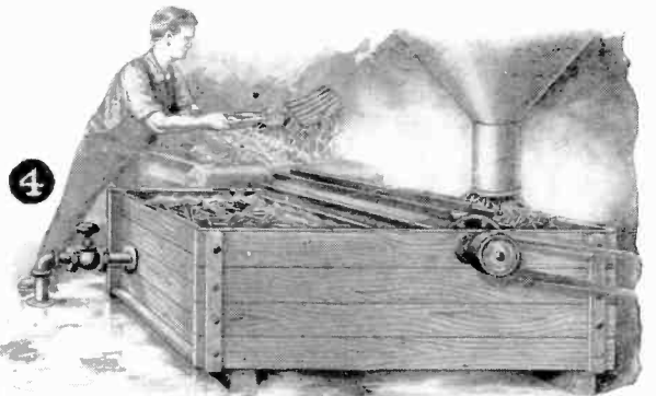
In illustration 3 the veneer is being shaved by a guillotine-like knife. The eighty or more pieces of veneer six inches wide, are cut into 240 or more individual match sticks. These fall into a hopper and by means of air are blown upstairs into an impregnating solution shown in illustration 4.
