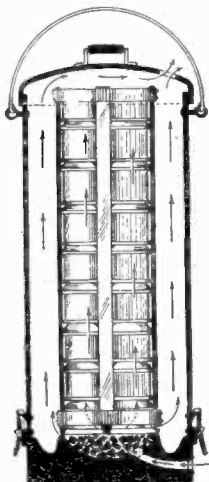
This is a diagrammatic view through the food carrier; note that the air enters through a vent, passes through charcoal and escapes at the top.
