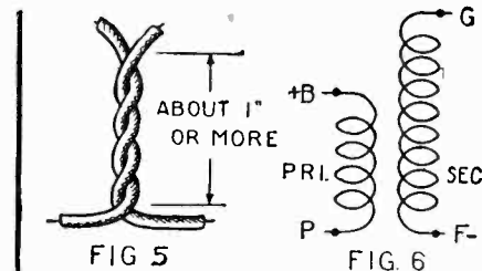
FIG. 5 FIG. 6 If the windings of the R.F. transformers are put on in the same direction, then the connections should be made as in Fig. 6.
