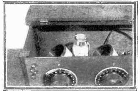
A bottle of calcium chloride or slaked lime inside the set keeps the air free from moisture and thus improves reception.
