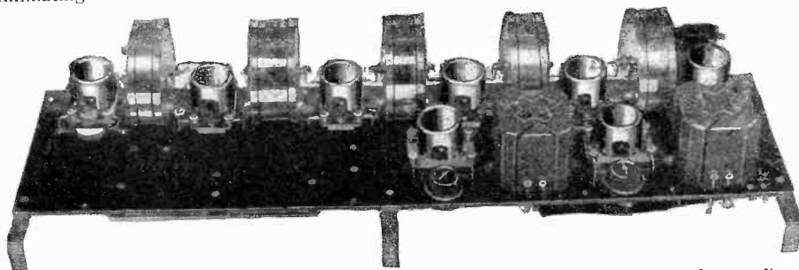
Front view of Super-heterodyne showing eight sockets, heteroformers and the two extra large audio frequency transformers employed. Under most conditions one such stage of audio is sufficient.
