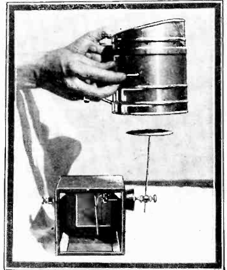
Every kitchen a power-plant. Flour sifted upon the receiving plate instantly causes the leaf to move, due to the electrical charge produced upon the flour particles when agitated.
