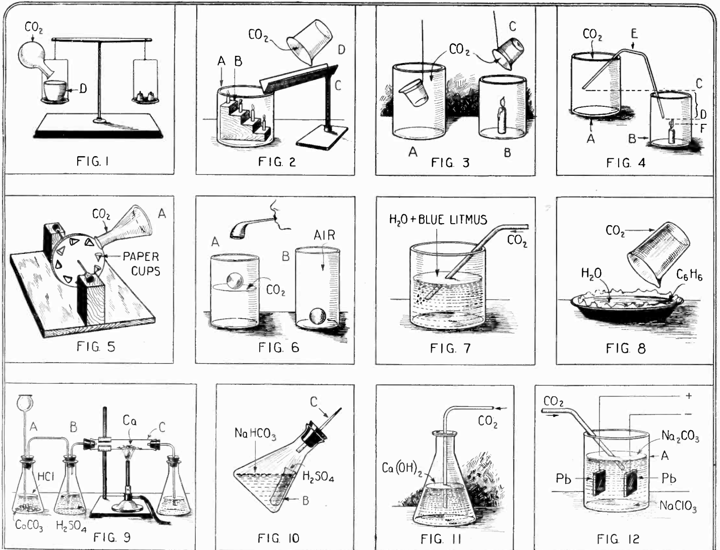
Fig. 1, Weighing a vessel full of carbon dioxide. Fig. 2, the carbonic acid stairway, putting out candles. Fig. 3, dipping the gas out of one vessel and pouring it into another so as to put out the candle. Fig. 4, siphoning the gas as if it was water. Fig. 5, turning a mill with the gas. Fig. 6, floating a soap bubble upon the gas. Fig. 7, blue litmus solution is turned red by carbonic acid gas bubbles. Fig. 8, putting out a flame of benzene with the
