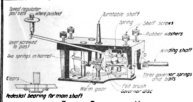
TYPICAL PHONOGRAPH MOTOR -1-
