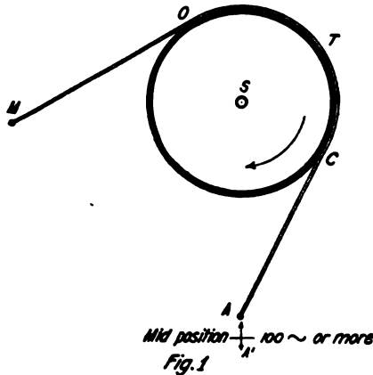
Fig. 1—The "Vibro Whip," Described by Mr. Roos, is Based on the Principle of the Old "Whip-Top," Which We Used to Spin in Our Boyhood Days, and the Action of Which is Partly Shown in the Above Figure—the Band Around the Drum "S" Being Pulled and Released Alternately in the Direction A-A'.
