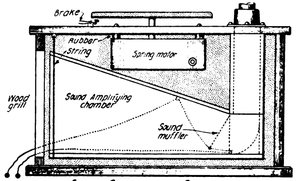
SOUND CHAMBER IN CABINET -7-
