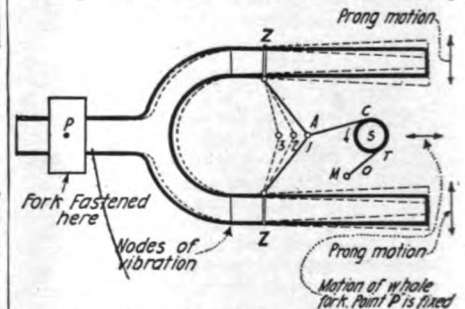
Z-Z —Movable points of attachment of driving belt which moves point A from 1-3 as fork vibrates.
