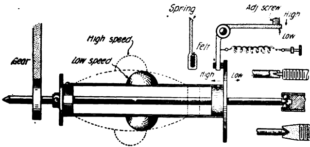
DETAIL OF PHONOGRAPH GOVERNOR -2-
