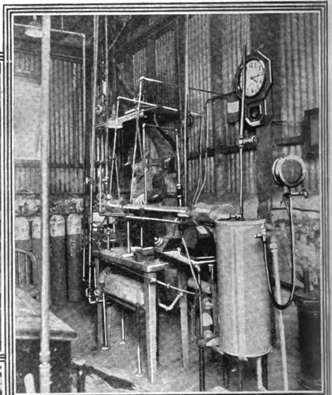
Above:—First Step in the Lamp Factory. Here the Approximate 30 Per Cent of Oxygen in Commercial Argon Shipped in the Cylinder at the Left Is Burned Out in a Hydrogen Flame, Leaving Argon and Nitrogen.
