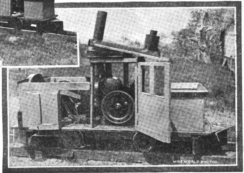
Who Wouldn't Like to Have a Model Railway Running Around Their Backyard Just Like This—and You Can Have One at Small Expense. If You Just Want to Have a Small Locomotive, Either a 1/4- or 1/2-H.P. Engine Will Do. The Engine Here Shown, Pulling a Trailer Car and All, Is Provided with a 4-H.P. Gasoline Engine.
