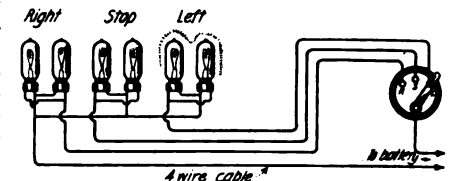
A Simple Yet Positive Electric Signal For the Rear of Your Automobile. It Is Operated From the Seat.
