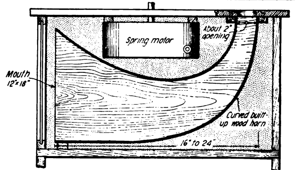
BEST SHAPE FOR WOODEN HORN -8-
