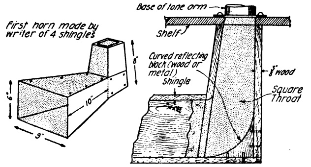
THE SHINGLE SOUND CHAMBER -6-
