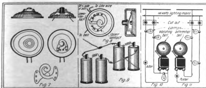
Fig. 7—Shows Plan, Section, Elevation and Metal Contacts of a "Push-Button." Fig. 8—Shows Plan and Section of Double Contact Push. Fig. 9—Battery Cells Connected in Series-Parallel. Figs. 10 and 11—Bells Being Operated From Lighting Mains.
