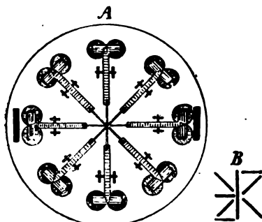
A—Plan view of type arms. B—Face of type magnified. Fig. 4—How the Eight Pairs of Electro-magnets and Type Bars Are Arranged on the Rogers Printing Telegraph. Also Close-Up View of Type Components.
