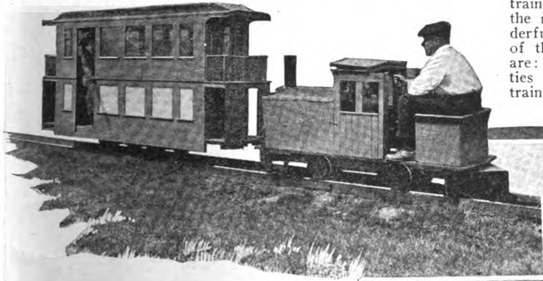
Who Wouldn't Like to Have a Model Railway Running Around Their Backyard Just Like This—and You Can Have One at Small Expense. If You Just Want to Have a Small Locomotive, Either a 1/4- or 1/2-H.P. Engine Will Do. The Engine Here Shown, Pulling a Trailer Car and All, Is Provided with a 4-H.P. Gasoline Engine.
