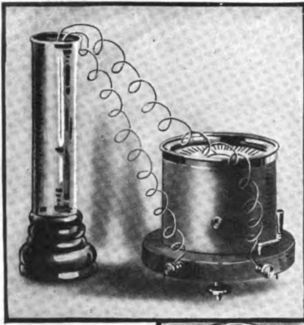
Above: A Coil of Special Wire Is in Circuit With a Current Meter; the Coil Is Immersed in the Liquid Air. The Current Increases As the Temperature is Lowered, and the Reading Gives the Temperature.
