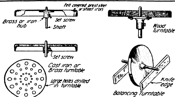
VARIOUS STYLES OF TURNTABLES -5-
