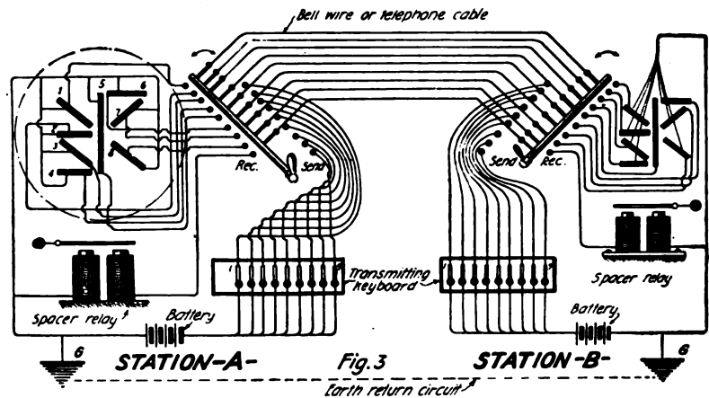
Fig. 3—Simplified Circuit For Printing Telegraph of the Rogers Type. Each Part of the Letter is Formed by Pressing the Proper Strap Keys at the Transmitting Station, the "Receiver" Being Switched Into Circuit, of Course.
