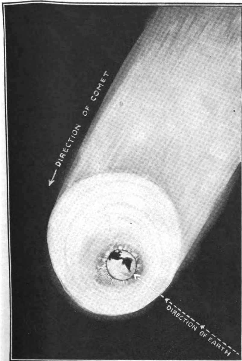
A Distant View Taken From Space Shows How the Earth Would Plow Thru the Head of a Comet. Note That the Head of the Comet Measures About 100,000 miles. It Would Take About 40 Minutes for the Earth to Traverse Thru the Nucleus of the Comet for the Reason That the Two Bodies Move at the Rate of 40 Miles per Second.
