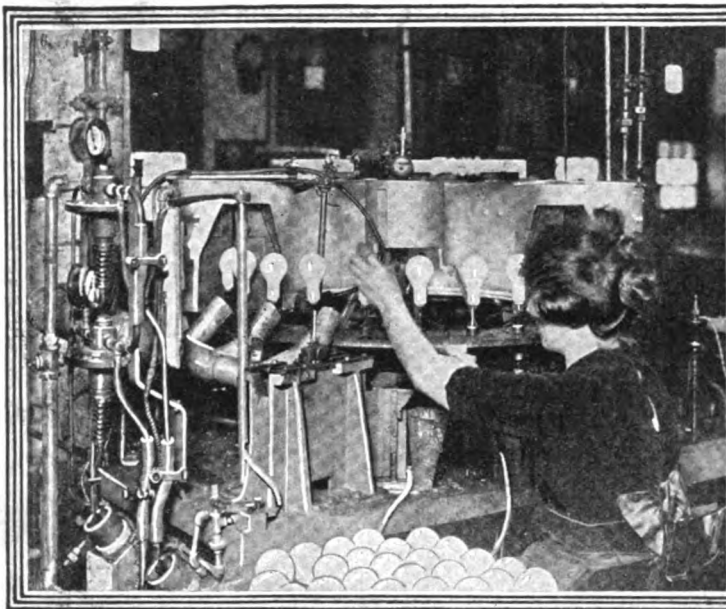
Above:—Here the Lamps Are Thoroughly Exhausted on the Turn-table Which Carries Them Thru the Oven. As They Come Out (Left) They Are Cooled by Three Blasts of Air. The Argon Is Injected From Beneath When the Lamp Reaches the Position at the Operator's Left Hand. The Bulb Is Sealed and Ready for Use—an "Argon Filled" Lamp.
