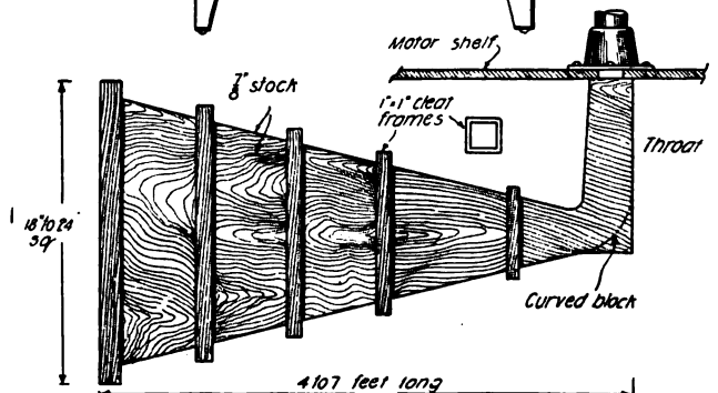
LARGE EXHIBITION STYLE HORN BUILT OF WOOD -10-
