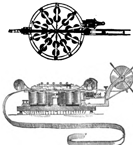
Fig. 5—A Rogers Type Printing Telegraph Having 10 Characters Instead of 8, Together with 10 Pairs of Operating Electromagnets, "Spacing" Relay Magnets, Paper Reel For Tape, Etc.
