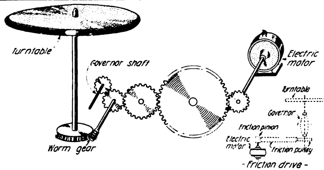
ELECTRIC PHONOGRAPH MOTOR -4-
