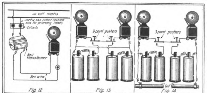
Fig. 12—Shows Connections of Step-Down Bell-Ringing Transformer. Fig. 13—Two-Line "Return Call" Bell System with Two Sets of Batteries. Fig. 14—Illustrating a "Grounded" Return Call System; Separate Batteries For Each Circuit.
