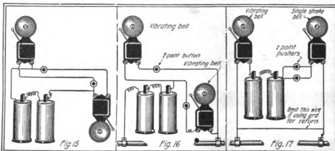
Fig. 15. Three-Line "Return Call" Bell System, — One Battery Ringing Either Bell. Fig. 16. Two-Line Grounded Return Call System With Common Battery. Fig. 17. Three-Line Return Call System, Common Battery.
