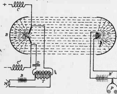
RUHMER'S PHOTOPHONIC TRANSMITTER AND RECEIVER
