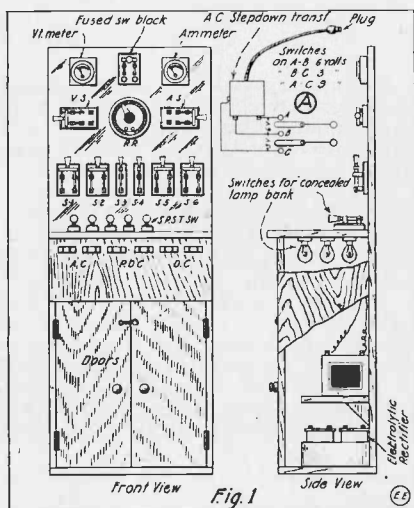
Front and Side View of 110 Volt Switch-board.
