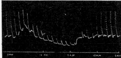
RECORD FOR 24 HOURS SHOWING DIURNAL VARIATION OF EXCITABILITY
