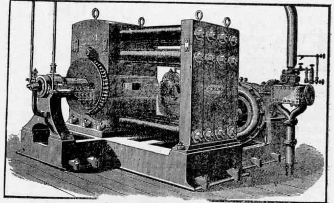
One of First Dynamos.
