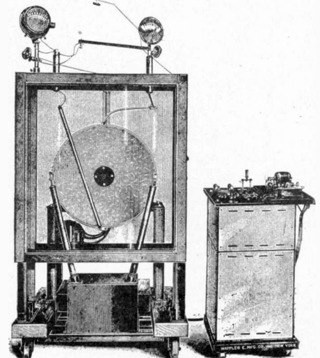
Fig. 5. Heavy Current Interrupterless X-Ray Generator. Micanite Disc Is Seen Enclosed In Glass Cabinet. 100,000 Volt Transformer at Base.
