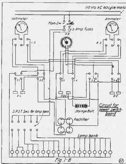
Circuits for 110 Volt A.C. Switch-board.
