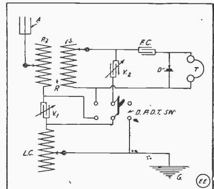
Throw-over Switch for Short and Long Wave Tuning.
