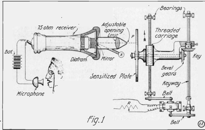
Scheme for recording the voice photographically.
