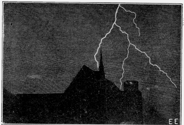
Showing a Single Stroke of Lightning From Cloud to Earth. A Return Stroke From Earth to Cloud Often Occurs. Hence the Fallacy of Staying in a Cellar.
