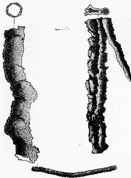
Showing the Very Peculiar and Striking Forms Produced in Sand When Lightning Strikes It. Sometimes Called Lightning Tubes.
