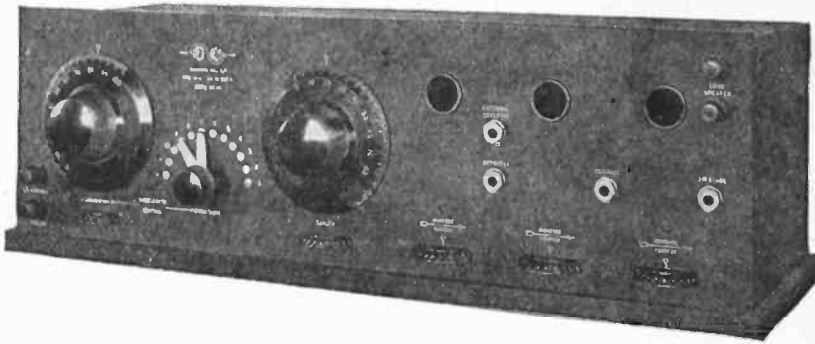
THE CELEBRATED GREBE CR-9 RECEIVER
