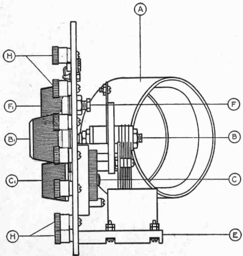
FIGURE 5: In this drawing is shown the method of mounting the coupler, the condenser, the rheostat, the socket and the binding posts. The knobs and dials are fastened to the shafts of the instruments (where they protrude through the face of the panel) by set-screws.
