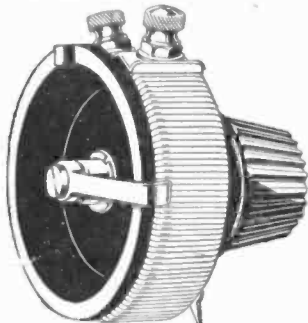
No. 650—FROST-RADIO Bakelite Rheostat
