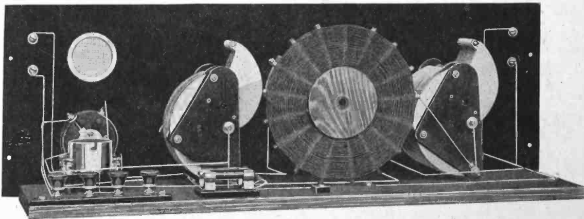
Receiver, by courtesy Radio Specialty Shop, Chicago, Ill.
