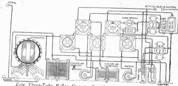
Erla Three-Tube Reflex Circuit—Complete Blue Prints. 50c each.
