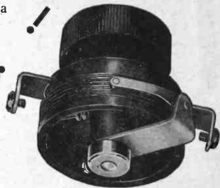
Unity Vernier Rheostat (Successor to the Jenkins Rheostat)
