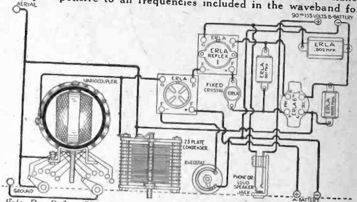
Erla Duo-Reflex Circuit, Using One Tube—Complete Blue Prints, 25c Each.
