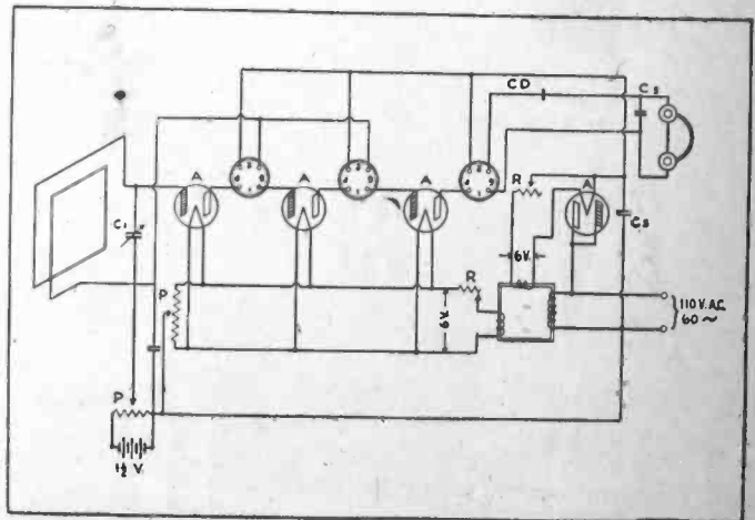
Loop Receiver using 60 cycle AC to operate filaments and plate voltages.
