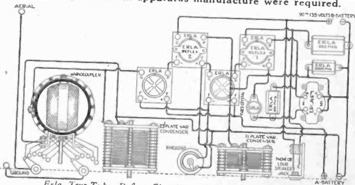
Erla Two-Tube Reflex Circuit—Complete Blue Prints. 35c each.
