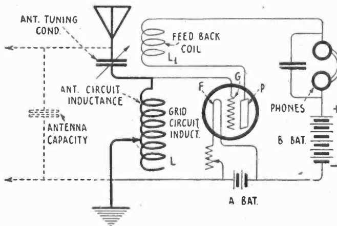
FIG. 1 A typical single-circuit arrangement, with the tube connected directly to the antenna circuit
