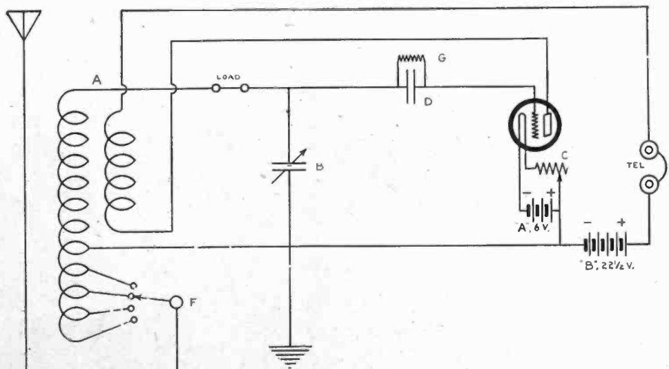
THE ELECTRICAL CONNECTIONS FOR THE PARTS USED IN THE CIRCUIT
