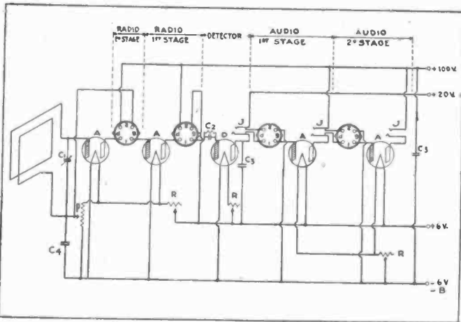
Loop receiver with two stages radio, detector and two stages audio frequency amplification.
