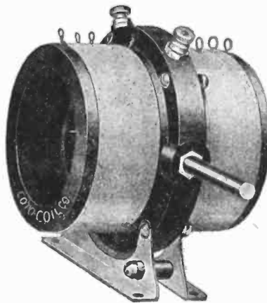
Coto Compact Moulded Bakelite Variocoupler
