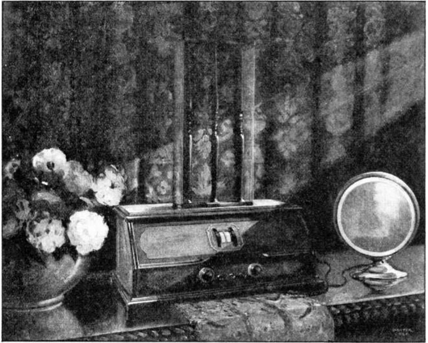
Radiola 25, (picture above with Loudspeaker Model 100), a six-tube uni-control Super-Heterodyne, that uses the new power tube. It has space in the cabinet for dry batteries, but can be adapted for use with Loudspeaker Model 104, for complete operation on 50 or 60 cycle, 110 volt A.C. lighting circuit. With 6 Radiotrons. List . . . $165
