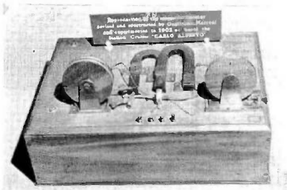
Early model of Marconi magnetic detector.
