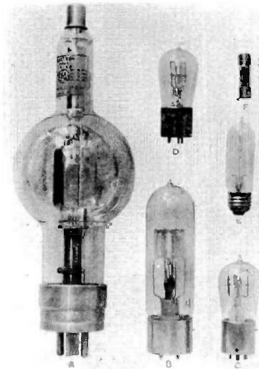
Receiving and transmitting tubes up to 5 watts, 1918.
