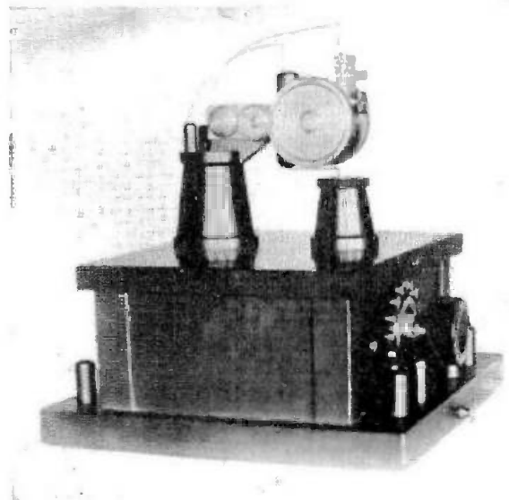
First Fessenden Barretter or electrolytic detector, 1905.
