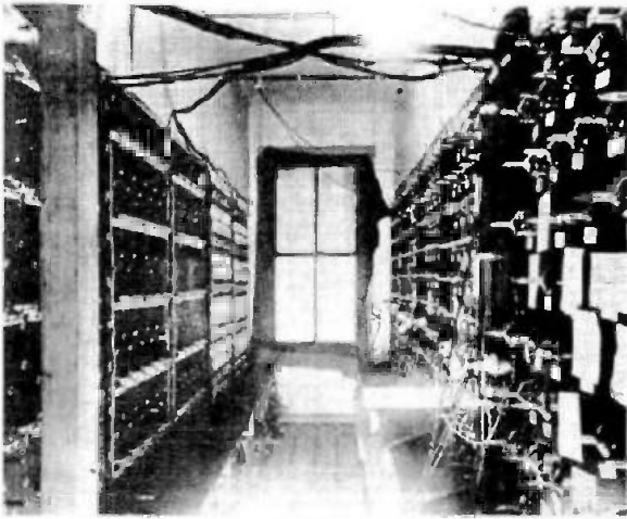
Racks of tubes arranged in parallel as used during the first radiotelephone conversation across the Atlantic in 1915, from Navy station NAA.
