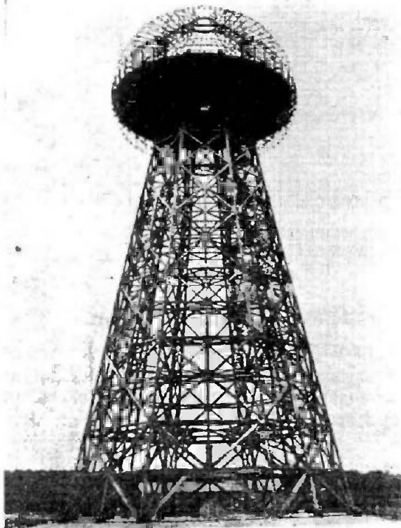
FIG. 2.—TESLA CENTRAL POWER PLANT AND TRANSMITTING TOWER FOR WORLD TELEGRAPHY, VARDENCLIFFES, LONG ISLAND, N. Y.
