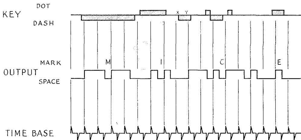
Fig. 1—Some possible key-level positions during the sending of the word "MICE" illustrate how the "Ultimatic" key corrects for operator timing errors.
