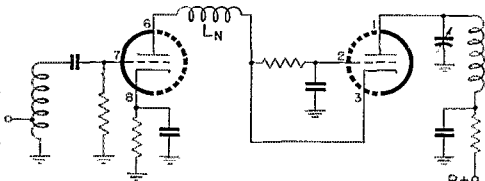
Fig. 2—Modification of the cascode circuit suitable for 2-meter r.f. amplifier service. The coil L_N is resonant at the middle of the band with the input capacitance of the second triode section. Its adjustment is not critical. Suitable tubes are the 6BQ7A, 6BK7 or 6BZ7.
