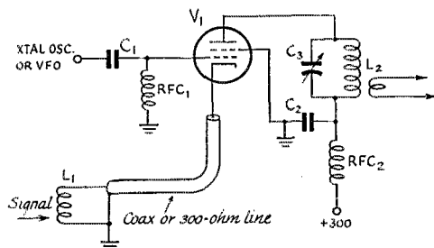
Fig. 2 — This simple high-level mixer/amplifier has been used by W6EDD and others. The heterodyning signal is present at the grid in either amplifier or mixer service — the tuning of the output circuit, L_2C_3 , determines the function.
