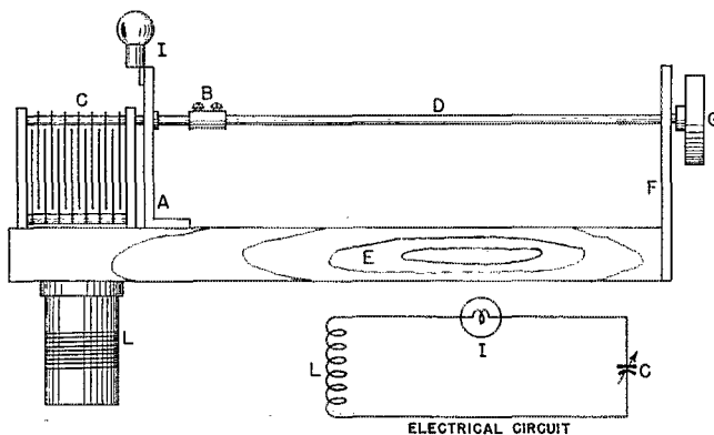
Fig. 3— An absorption-wavemeter layout that protects the operator from accidental high-voltage shock. (A) Right-angle bracket. (B) Shaft coupling. (C) Tuning capacitor. (D) Insulated shaft. (E) 12-inch length of 1-by-2-inch board. (F) Shaft-support plate. (G) Control knob. (I) Dial-lamp assembly. (L) Tank coil.
