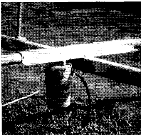
A plastic fruit-juice container makes a good weather protector for the variable condenser.
