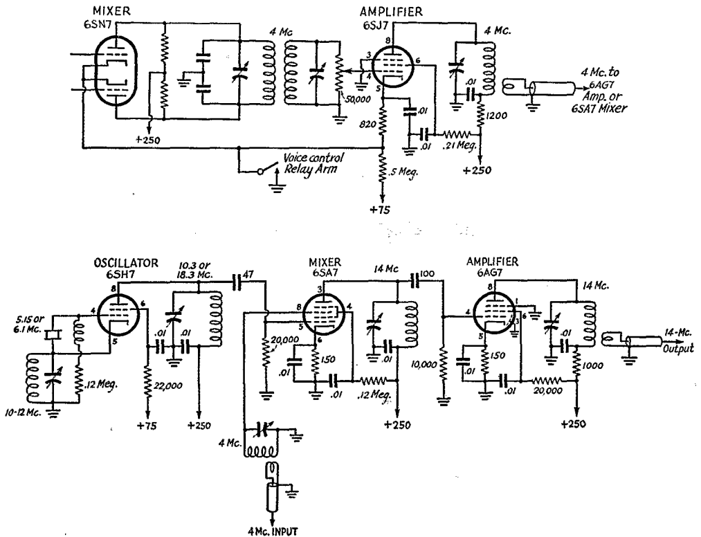
Fig. 1— Here is the way W2FGV converts the 4-Mc. output from his Edmunds (W1JEO) exciter to 14 Mc. The top circuit shows the only modification in the original circuit, the addition of the 6SJ7 amplifier, and the bottom circuit shows the 6SA7 mixer and a 6AG7 amplifier working on 20. John has the whole thing built on a 13 × 17 × 3-inch chassis and uses it to drive a pair of 807s running 125 watts on either 75 or 20.
