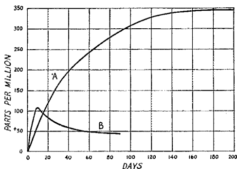
Fig. 3 — Aging curves of Type KV3 crystals in the FS135C 100-kc. oscillator. Curve A, crystal No. 2 in oscillator No. 2; curve B, crystal No. 1 in oscillator No. 2.
