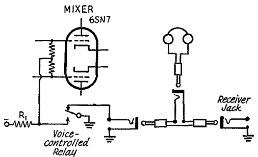
Fig. 2— W5BDX uses this simple circuit with his voice-controlled relay to open the headphone circuit and to bias back the mixer (and other stages) with one arm of the relay. R_1 is a current-limiting resistor, to avoid a dead short on the negative supply.
