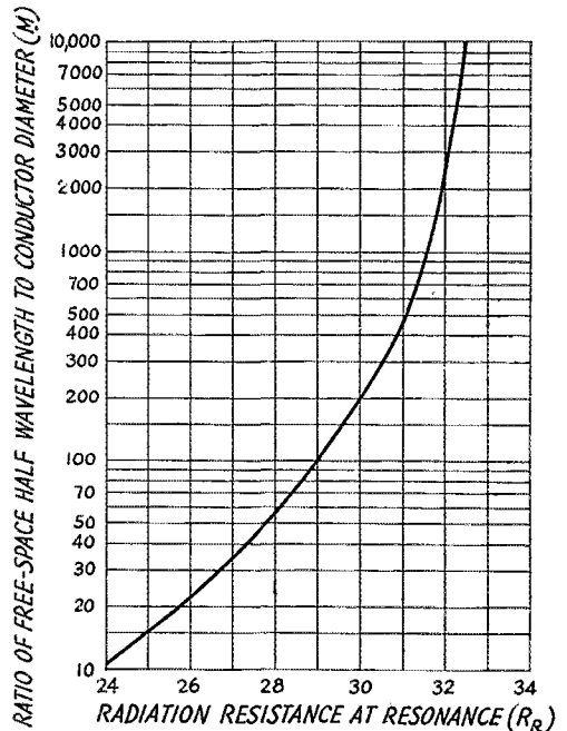
Fig. 4—Radiation resistance of a quarter-wave antenna (with ground plane or grounded) as a function of M . The values apply only when the antenna is of the resonant length. Multiply resistance values by 2 for half-wave antennas.
