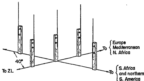
Fig. 4 — Two extra elements pivoted on the same driven element will provide two additional directions of optimum radiation. The arrangement shown above has been used at W5DF to cover the compass points indicated. By using a total of seven elements, with the parasitic elements spaced 60 degrees around the driven element, there is a choice of six directions giving complete coverage.
