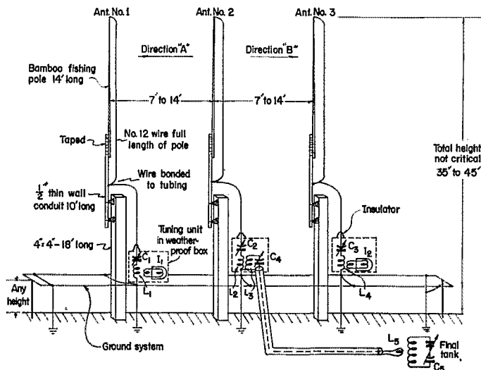
Fig. 1—The 7-Mc. 3-element beam at W5DF. This drawing (not to scale) shows the essential electrical and mechanical features. The same antenna can be used on 14 Mc., but the separation between elements should not exceed 10 feet if that band is to be used. W5DF has also used it on 80 meters to work ZL with a 25-watt transmitter.
