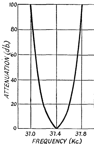
Fig. 2 — Selectivity characteristic of the 37-ke. i.f. amplifier.
