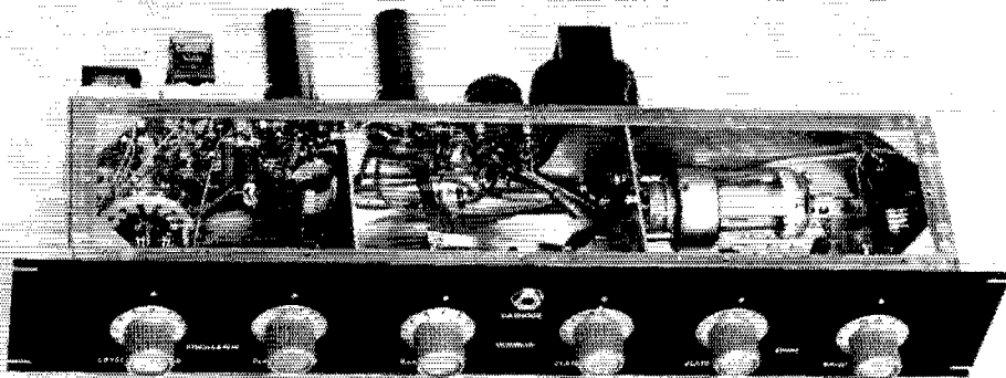
Looking into the handswitching exciter-transmitter from the top front. Oscillator components are in the left compartment, the doubler and power connector in the center, and the output stage at the right. Note that the 6146 socket is mounted inside the output stage compartment.
