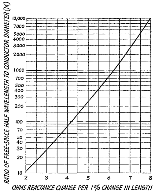
Fig. 3—Reactance change with antenna length as a function of M , for quarter-wave ground-plane (or grounded) antennas. If the antenna is longer than the resonant length the reactance is inductive; if shorter, the reactance is capacitive. The curve is accurate for lengths within 10 per cent of the resonant length. Multiply reactance values by 2 for half-wave antennas.
