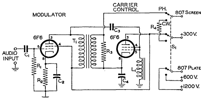
Fig. 1—Circuit diagram of the controlled-carrier system.
