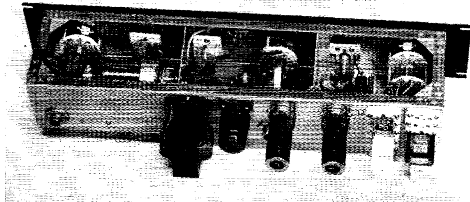
Rear view of the exciter. On the rear wall at the right are 10 crystal sockets of various types. Then come the two 5763s, the power plug, the filament transformer, and the output coaxial fitting. Components on the inside front wall are, in the same order, the crystal switch, oscillator tuning, doubler bandswitch, doubler tuning, and final bandswitch.
