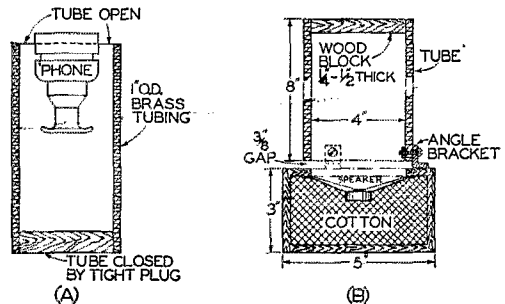
Fig. 1—Two methods of adding further audio selectivity are shown here. Both are extensions of the same principles involved in adding selectivity by means of the Q5-er and other sharp i. f. systems, but attack the problem from the mechanical side.
