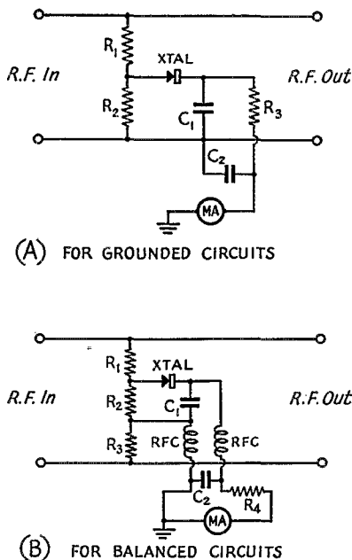
Fig. 1 — R.f. voltmeter circuits. In the upper circuit, A, R_1R_2 is a voltage divider for reducing the peak voltage applied to the crystal; R_1R_2R_3 serves the same purpose in the lower circuit. To a first approximation, these dividers can be calculated on a d.c. basis, although the ratios at r.f. are likely to differ considerably, depending on the frequency, the shunt capacitances of the resistors and stray pick-up in the crystal rectifier circuit. C_1 and C_2 are r.f. by-passes; 0.005 \mu fd. is a satisfactory value. Design considerations are discussed in the text.
