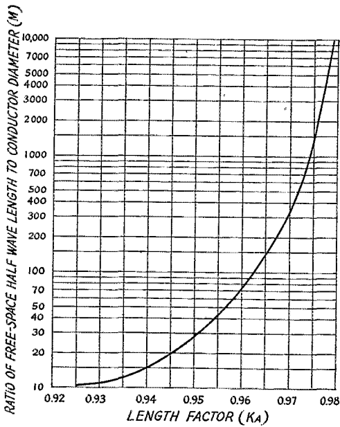
Fig. 2—The antenna-length factor as a function of the ratio of a free-space half wavelength to the conductor diameter. The length factor multiplied by a free-space quarter wavelength is the length of a quarter-wave radiator resonant at the selected frequency.
