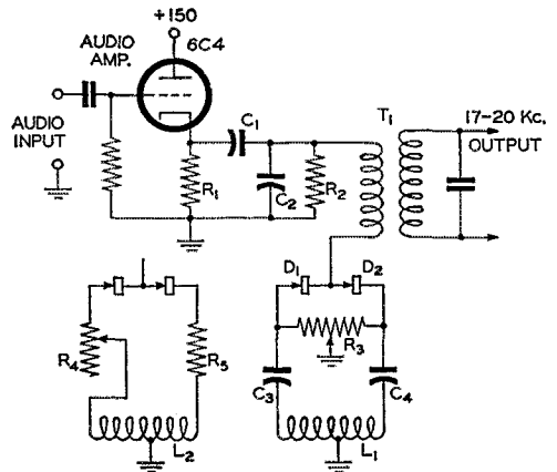
Fig. 2 — The series balanced-modulator circuit for generating double sidebands and suppressed carrier. An alternative oscillator connection is shown at the lower left.
