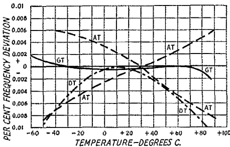
Fig. 1 — Typical frequency-temperature characteristics of three types of crystal cuts used in frequency standards.
