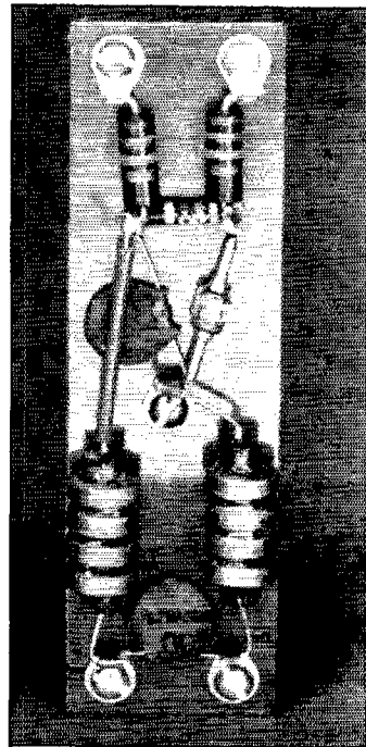
Voltmeter assembly for a balanced circuit. Except for R_4 and the milliammeter, all the parts shown in the lower circuit of Fig. 1 are mounted on a piece of thin bakelite, and arranged so that when the bakelite base is mounted with its flat side at right angles to the direction of the transmission line the coupling between the line and voltmeter circuit will be minimum. The leads to R_4 and the meter may be any length since they carry only a very small direct current.
