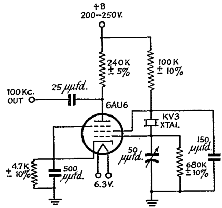
Fig. 2 — Oscillator circuit for a simple 100-kc. crystal standard.
