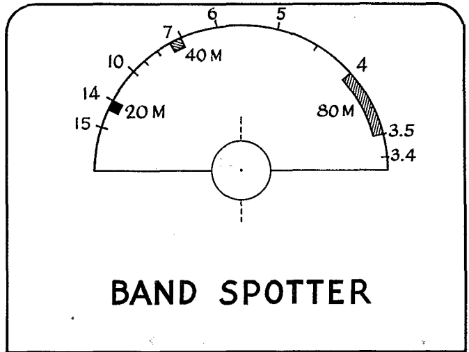
◆ Fig. 2 — Actual calibration of the wavemeter. This drawing may be cut out or traced and pasted to the face of the aluminum bracket provided the parts listed below Fig. 1 are used in the construction. ◆
