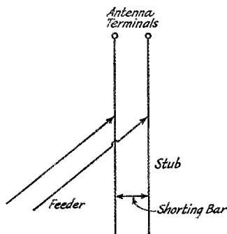
Fig. 1—The shorted stub, with feeders tapped on for matching. If the antenna impedance is higher than the line characteristic impedance, the stub should be approximately one-quarter wavelength long; if the antenna impedance is lower than the line impedance the stub should be one-half wavelength long.
