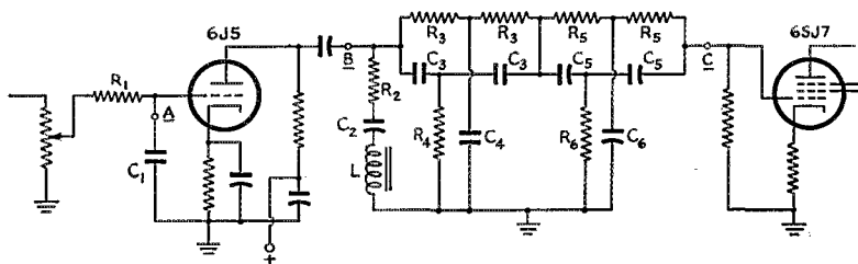
Fig. 6—Circuit diagram of voice-frequency filter. Note: the circuit designations should not be confused with those of the main diagram.
