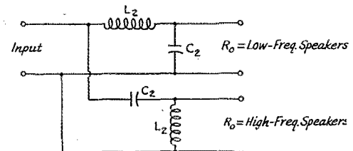
Fig. 2 — Cross-over networks.
