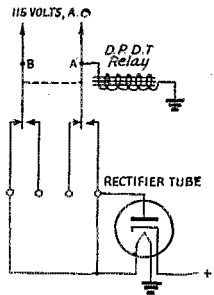
Fig. 4 — Using a d.p.d.t. 115-volt relay as an automatic circuit polarizer to assure correct line-plug connections in a transformerless power supply.
