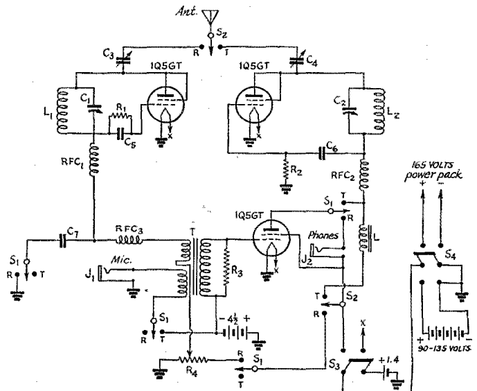
Fig. 1. — Wiring diagram of the WERS "walkie-talkie."
