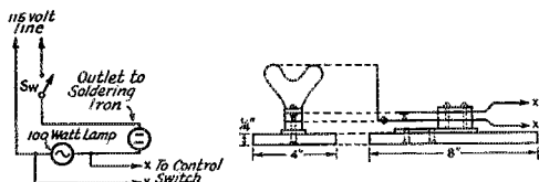
Fig. 8 — Soldering-iron rest and heat control.
