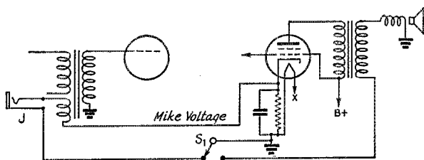
Fig. 6 — Simplified transmit-receive switching circuit for the Alleghany County WERS transmitter-receiver in August QST .
