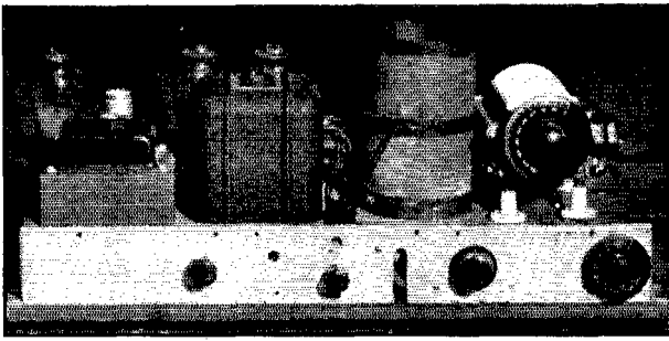
Transmitter, modulator and power supply are built on one chassis and arranged for remote control from the operating position. The final tank coil and variable tuning condenser are at right.
