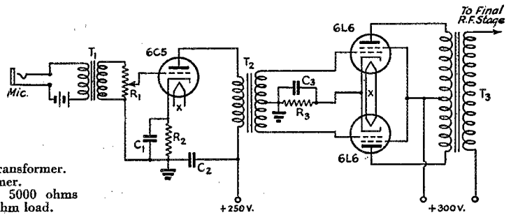
Fig. 2 — Modulator circuit diagram.
