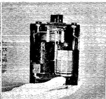
The QRP rig and "beer-can" antenna with which W9GGI once worked all states; as well as K5, K6 and K7, on 7Mc. The rig consists of a simple 6V6 crystal oscillator. The quarter-wave vertical antenna is made up of one-quart oil cans soldered end-to-end. W9GGI built a power supply for the rig in the same size box to match the transmitter.
