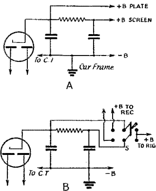
Fig. 2 — Switching arrangement for using the power supply from a car h.c. receiver for the mobile unit. A shows the original power circuit, while B shows the altered circuit. S is a d.p.d.t. toggle switch.
