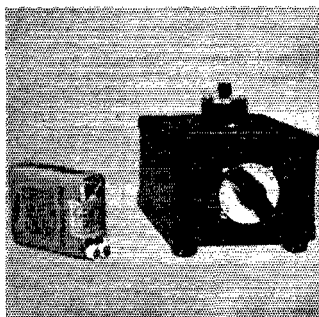
The QRP rig and "beer-can" antenna with which W9GGI once worked all states; as well as K5, K6 and K7, on 7Mc. The rig consists of a simple 6V6 crystal oscillator. The quarter-wave vertical antenna is made up of one-quart oil cans soldered end-to-end. W9GGI built a power supply for the rig in the same size box to match the transmitter.
