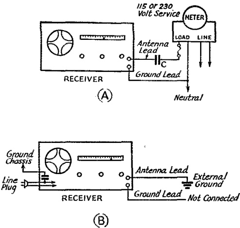
Fig. 5 — Methods of coupling receiver to the line.
