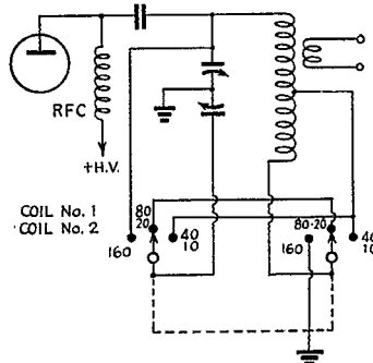
Fig. 3—W9IXE's arrangement for covering five bands with two coils.
