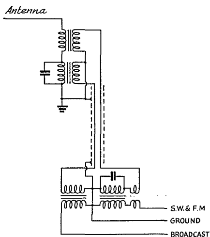
Fig. 2 — Modern all-wave antenna system covering range from 400 to 22,000 kc., with shielded transmission line and two-channel double-transformer couplers at antenna and receiver.
