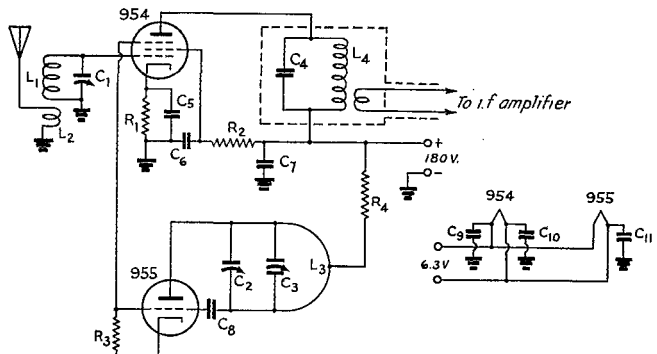
Fig. 1 — Wiring diagram of the 225-Mc. converter.
