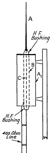
Fig. 1—W8SR's scheme for feeding a coaxial antenna with an open-wire line. A and A 1 are halves of the half-wave dipole, while B and C form a quarter-wave matching section.
