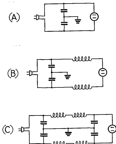
Fig. 3 — Representative types of power-line filters.
