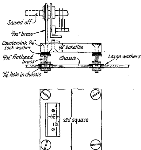
Fig. 2 — Adjustable condenser mounting for oscillator section of condenser gang. Only this mounting has four legs; the other two mountings have three legs each.
