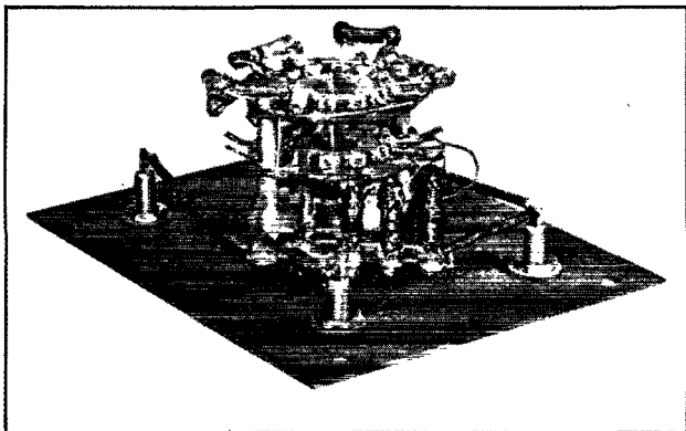
This view shows the series resistors mounted on the switch and the parallel shunts supported by a lug strip.
