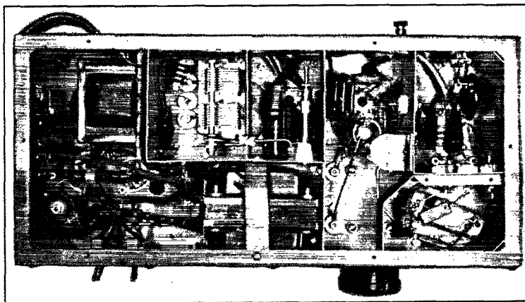
Bottom view with dust cover off. The oscillator coil compartment, in the lower right-hand corner, has a separate cover so that bending of the chassis cover cannot cause a frequency change.
