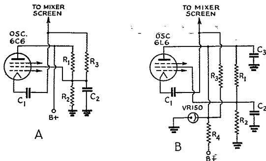
Fig. 2—HRO receiver circuit changes suggested by W3JVJ for improving voltage-frequency stability. A—Original circuit. B—The modified circuit. C_1, C_2, C_3 —0.1 \mu\text{fd} . R_1 —50,000 ohms. R_2, R_3 —100,000 ohms. R_4 —3000 ohms, 5-watt.
