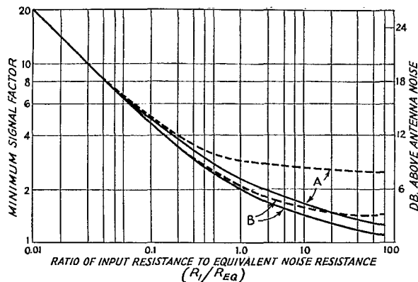
Fig. 2 — Minimum signal factor vs. R_1/R_{eq} . Dashed lines, antenna coupling adjusted for maximum gain; solid lines, adjusted for maximum signal-to-noise ratio. A, all electronic loading; B, no electronic loading.
