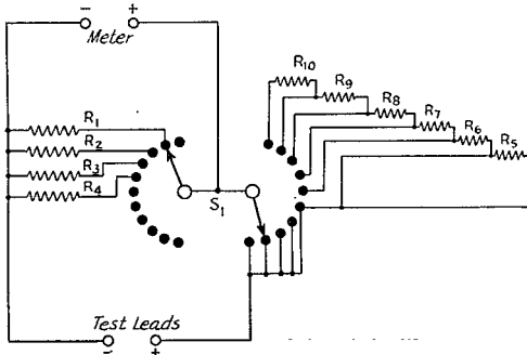
Fig. 1 — Wiring diagram of the multi-range volt-milliammeter-adapter.
