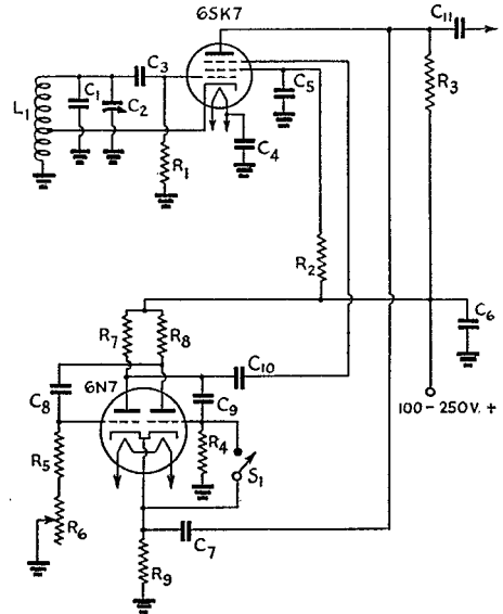
Fig. 4 — Circuit of simplified frequency standard.
