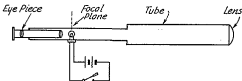
Fig. 1 — Light source in place in telescope used in simple light-beam communication experiments.
