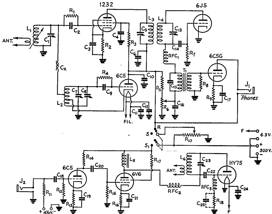
Fig. 1 — Circuit diagram of the 112-Mc. transmitter-receiver. Both shields of the 1232 should be grounded.
