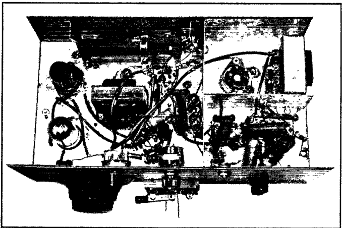
The various sections of the unit are boxed off by baffle shields as shown in this bottom view. The modulation choke is in the upper right-hand compartment. Other components are readily identifiable.
