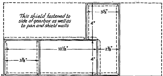
Shield compartment depth 5\frac{1}{2} "
