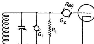
Fig. 1 — Simplified equivalent circuit for analyzing effect of various contributions to total noise.
