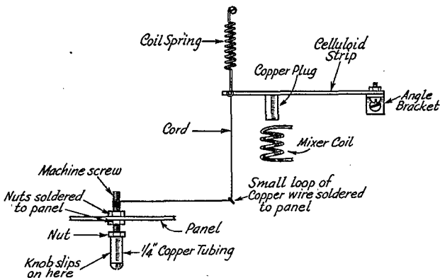
Fig. 2 — Mechanical system for varying the inductance of the mixer grid coil. The cord (thin fishline) winds up on the machine screw when the control knob is turned. The coil spring keeps the cord tight and pulls the copper plug away from the coil when the cord unwinds.
