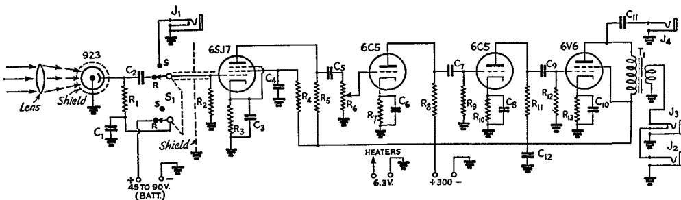
Fig. 1 — Modulator-amplifier circuit for light-beam communication.
