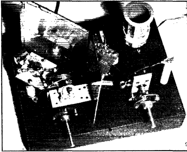
A top view of the 225-Mc. converter with the panel removed. The oscillator portion is at the left and the mixer section is at the right. The coil form at the upper right is the i.f. output transformer.
