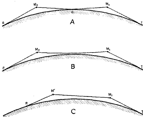
Fig. 8 — Three possible types of double skip. Type A involves direct reflection from the earth; type B upward refraction in the troposphere; type C a direct upper-atmosphere path between two sporadic masses.
