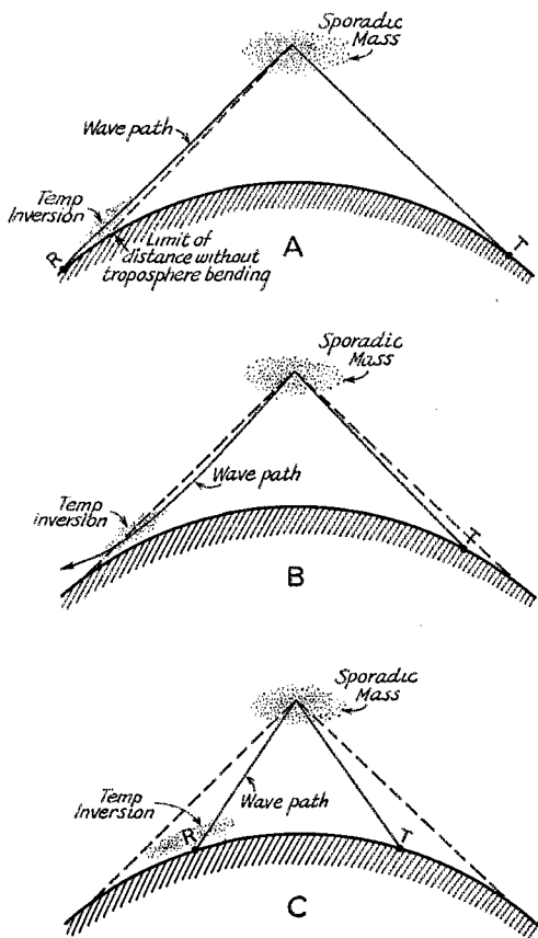
Fig. 7 — Effect of troposphere bending at the end of a skip path. At A the downcoming wave penetrates the region of the temperature inversion at practically horizontal incidence and is bent downward just as in the case of a wave originating on the earth's surface. In B , the wave arrives "on top" of the inversion, which from this viewpoint looks the same as it does from earth (i.e., the wave is travelling from a region of cooler air into warmer air), hence the wave bends away from the warmer air and away from the earth. In C the angle of incidence is still greater and the wave travels through the temperature inversion region because the bending is negligible.
