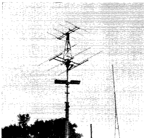
The 28- and 56-Mc. rotary arrays at W5DNN, Austin, Texas. The top section, recently added, is a 4-element array of the W6QLZ variety.
