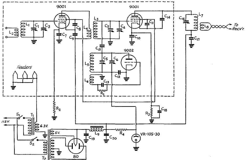
Fig. 1 — Circuit diagram of the 56-112-Mc. converter.
