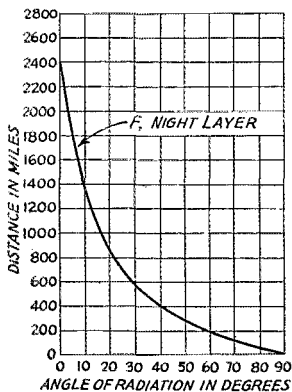
Fig. 3—A chart showing the distances from the transmitter at which waves at various vertical angles will be returned to earth from the night F layer under average conditions.
