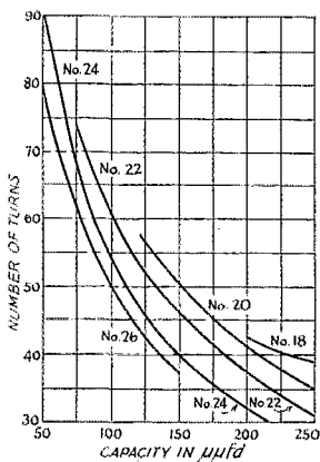
Fig. 1 — Turns required for various tuning capacities to resonate at 1700 kc. Sizes of enameled wire are indicated on the curves. Coils close-wound on 1½-inch forms.
