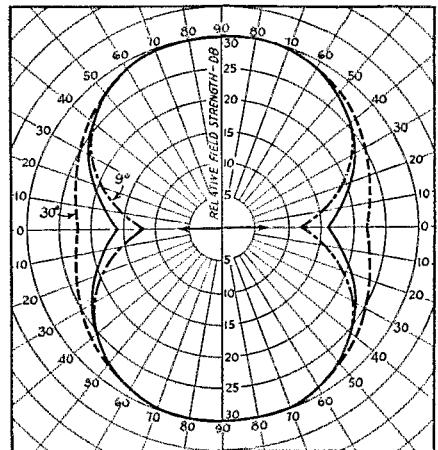
Fig. 6—Directive patterns of a horizontal half-wave antenna at three vertical angles, 9, 15 (solid line) and 30 degrees. The direction of the antenna is indicated by the arrow. These patterns are plotted to a 30-db. scale, which is about proportional to signal strength as determined by ear. If 30 db. represents an S9 signal, 0 on the scale will be about S1. All three patterns are plotted to the same maximum, but actual amplitudes at the various angles will depend upon the antenna height. The patterns show only the shape of the directive pattern as the angle is varied.
