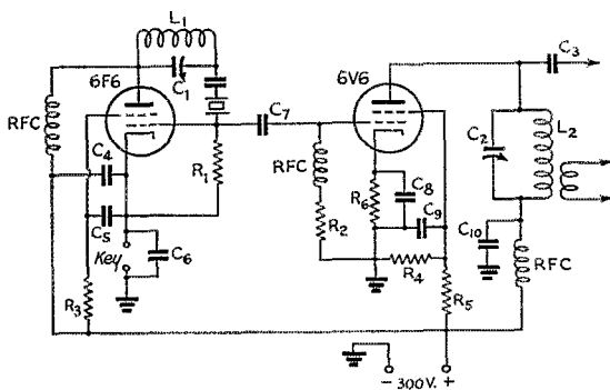
Fig. 2 — Circuit diagram of the 160-meter exciter using an 80-meter crystal.
