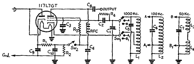
Fig. 1 — Wiring diagram of the 50-, 100- and 1000-kc. oscillator.
