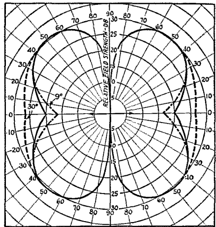
Fig. 7 — Horizontal pattern for a full-wave antenna, for vertical angles of 9, 15 and 30 degrees. Qualifications which are given under Fig. 6 apply to this pattern also.
