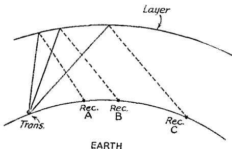
Fig. 1 — Signal paths from transmitter to various receiving points via ionospheric reflections. Signals received at A must be radiated at high angles, while radiations at lower angles are required for the more-distant points B and C.
