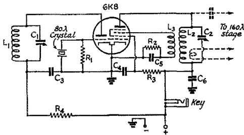
Fig. 1 — A "frequency halver," using a 6K8. Using an 80-meter crystal, 160-meter output is obtained from L 2 -C 2 .
