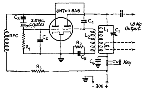
Fig. 3 — The simplified version of Fig. 2, using a Pierce crystal oscillator circuit, and the most practical of the "frequency halvers."
