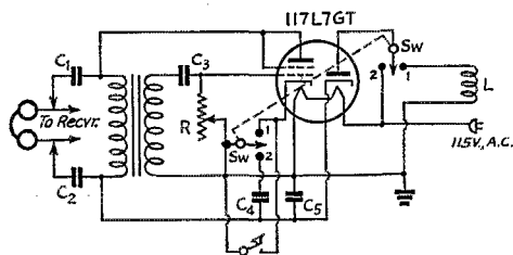
Fig. 5 — Circuit for combination code-practice oscillator and keying monitor.
