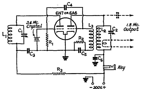
Fig. 2 — Another version of the "frequency halver," using a twin triode.
