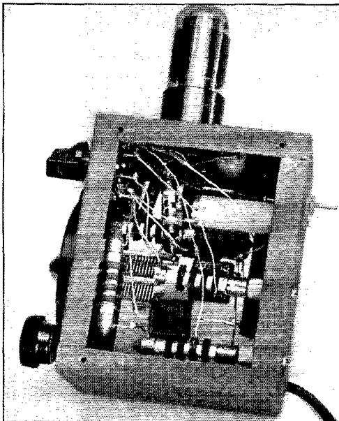
A shot of one side shows the arrangement of the inductances for the three tuning ranges. The long cathode leads running from the inductances are tied down at convenient points by drops of Duco cement. The 1000-kc. coil is at the top and the 100-kc. coil is in the center. Note that the 50-kc. inductance consists of two r.f. chokes at right angles.
