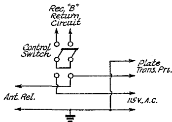
Fig. 4 — W8FAZ's single-switch control system
