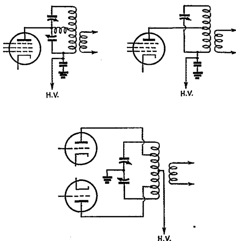
Fig. 4 — Tapping down on the plate tank to increase Q . The neutralizing condensers in the push-pull circuit should connect directly to the plates of the tubes rather than to the stator plates of the tank condenser sections.
