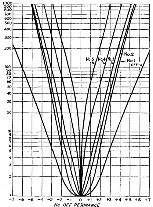
FIG. 3—OVERALL RESONANCE CURVES (CRYSTAL FILTER PLUS I.F. AMPLIFIER) WITH PHASING CONDENSER SET TO NEUTRALIZE THE CRYSTAL-HOLDER CAPACITY
