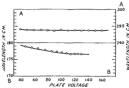
FIG. 5—WAVELENGTH CHARACTERISTICS OF THE TWO LOOP TRANSMITTERS Model A above
