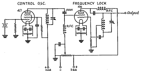
FIG. 1—FREQUENCY LOCK CIRCUIT
