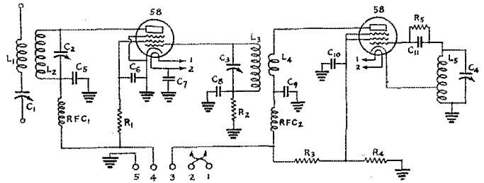
FIG. 2—CIRCUIT DIAGRAM OF THE OSCILLATOR-AMPLIFIER TRANSMITTER
