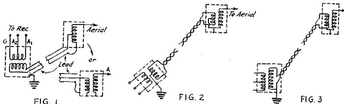
ARRANGEMENTS FOR IMPEDANCE MATCHING TO SIMPLE ANTENNAS, WITH SHIELDED AND TWISTED-PAIR LINES, ARE SHOWN IN FIGS. 1, 2 AND 3
