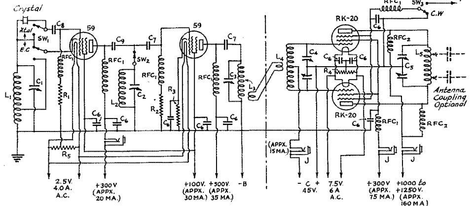
FIG. 1—THE TRANSMITTER R.F. CIRCUIT
