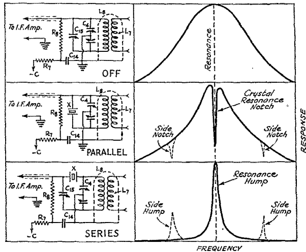
FIG. 4—THE SELECTIVITY CHARACTERISTIC OBTAINED WITH FILTER SWITCHING
