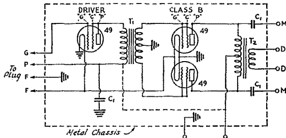
FIG. 4—SUBSTITUTION OF 5-PRONG SOCKETS IS THE MAJOR CHANGE TO BE MADE IN USING THE NEW TYPE 49 CLASS B TUBES
