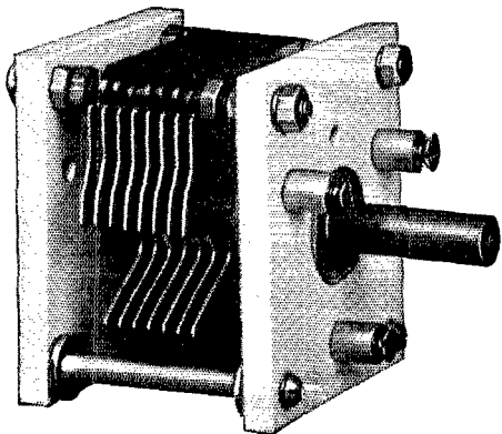
TYPE 568-D, 175 \mu\text{f} maximum, SLC Plates
