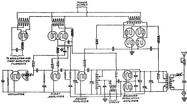
FIG. 1—SCHEMATIC DIAGRAM OF THE 100-WATT WESTERN-ELECTRIC TRANSMITTER USING GRID-BIAS MODULATION
