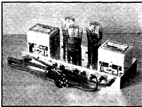
THE CLASS B AMPLIFIER WITH THE NEW TYPE 49 TWO-VOLT TUBES AND SILVER-MARSHALL TRANSFORMERS
