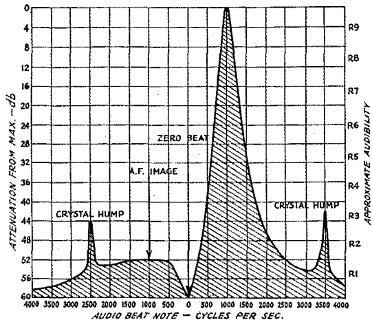
FIG. 5 — THE PICTURE OF SINGLE-SIGNAL C.W. SELECTIVITY
