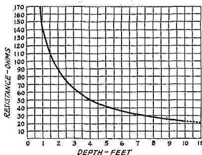
FIG. 2—CALCULATED EFFECT OF DEPTH ON THE RESISTANCE OF A GROUND CONNECTION perature at which the device operates can be varied within quite wide limits simply by moving the thermometer. The oven itself can be made to any design the builder may like.
