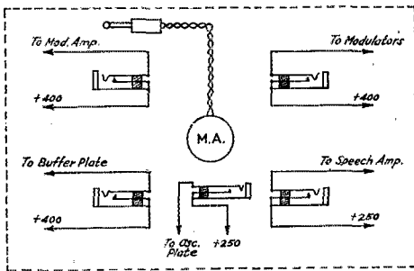
FIG. 2 — METER PANEL CONNECTIONS
