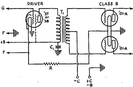
FIG. 2 — FOR USE WITH 6.3-VOLT TUBE RECEIVERS
