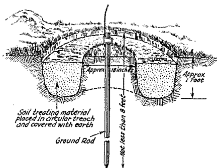
FIG. 5 — TRENCH METHOD OF SOIL TREATMENT Probably the most effective scheme of utilizing chemicals to lower soil resistance.
