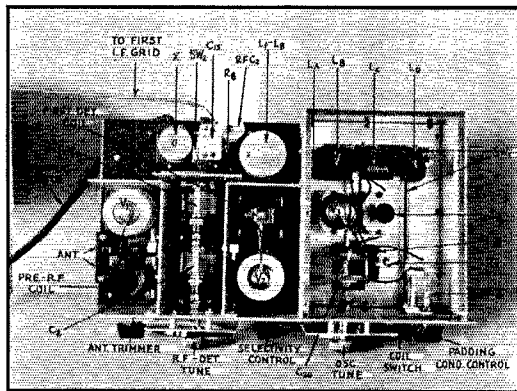
THE TOP PLAN, SHOWING THE ABOVE-DECK ARRANGEMENT IN DETAIL
