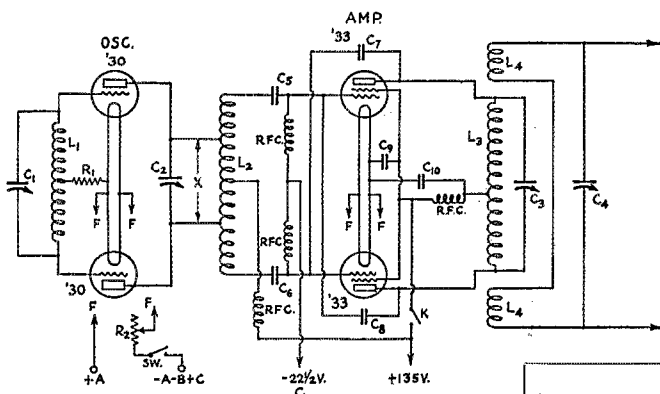
CIRCUIT OF THE PUSH-PULL BATTERY- OPERATED TRANSMITTER
