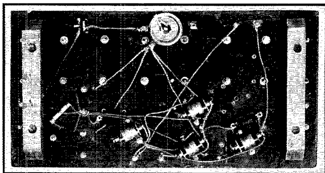
THE PLAN VIEW SHOWS THE RADIO-FREQUENCY WIRING. NOTHING COULD BE SIMPLER
