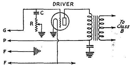
FIG. 3 — TONE CONTROL MAY BE ADDED TO THE AMPLIFIER, IF THE RECEIVER WITH WHICH IT IS USED DOES NOT HAVE THIS FEATURE
