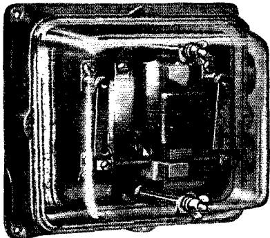
Phantom view of Keying relay (glass cover used only to obtain this effect)
