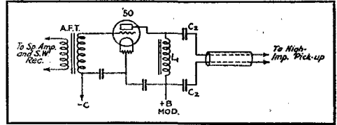
FIG. 4—THE MODULATOR OF A 'PHONE TRANSMITTER CAN BE USED AS THE RECORDING POWER AMPLIFIER
