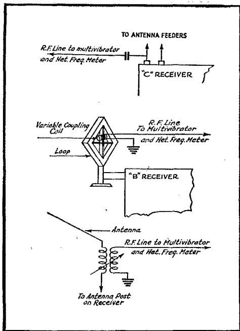
FIG. 2—THREE METHODS OF COUPLING FOR HETERODYNING A STATION SIGNAL BY A SIGNAL FROM THE FREQUENCY MEASURING EQUIPMENT
