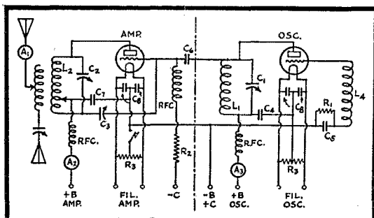
FIG. 4 — IN THIS CIRCUIT THE OSCILLATOR IS THE FIXED GRID COIL ARRANGEMENT OF THE T.P.T.G.
