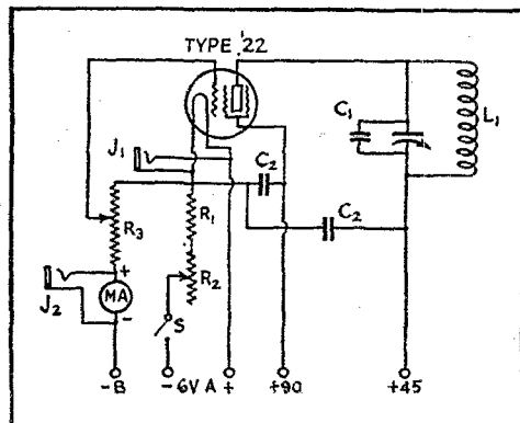
FIG. 1 — SCHEMATIC CIRCUIT OF THE FREQUENCY METER
