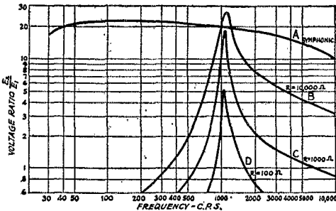
FIG. 3 — FREQUENCY-RESPONSE CHARACTERISTICS OF THE AMPLIFIER
