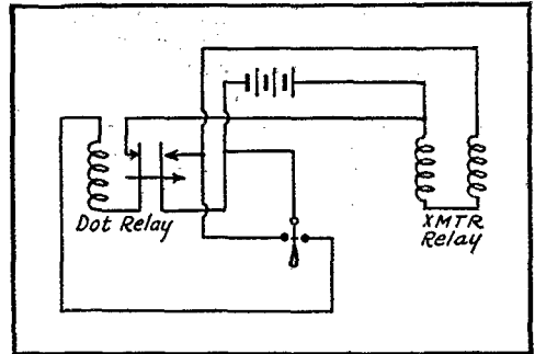
FIG. 3 — AN ARRANGEMENT WHICH ALLOWS KEYING AT SPEEDS BETWEEN TEN AND FORTY-FIVE WORDS PER MINUTE
