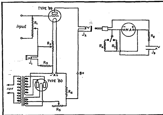
FIG. 1.—THE V. T. VOLTMETER CIRCUIT
