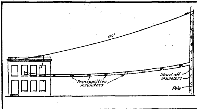
FIG. 1 — THE OUTDOOR RECEIVING ANTENNAS The 150-foot antenna is used mostly with the "B" receiver. The vertical Conrad antenna is designed particularly for high-frequency reception with the "C" receiver.
