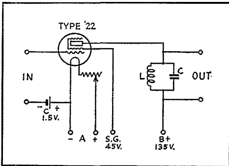
FIG. 1—THE USUAL SCREEN-GRID PEAK-AMPLIFIER CIRCUIT
