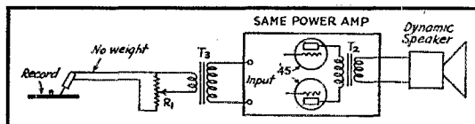
FIG. 2 — THE SAME POWER AMPLIFIER IS USED FOR REPRODUCING
