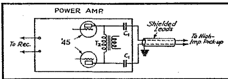
FIG. 3—THIS COUPLING ARRANGEMENT CAN BE USED WITH A HIGH-IMPEDANCE PICK-UP The condensers C_1 should each be 2 to 4 \mu d.
