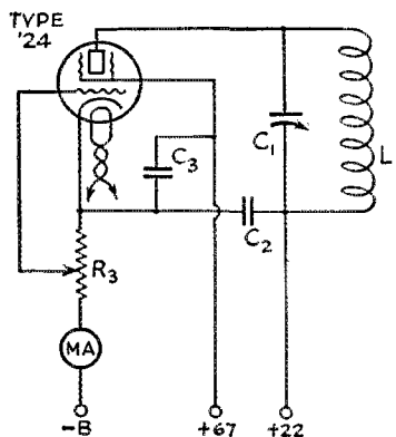
FIG. 5. — USING A TYPE '24 TUBE
