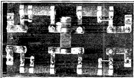
AN EASILY-CONSTRUCTED LINE PAD For matching a 500-ohm line to a 200-ohm microphone transformer.
