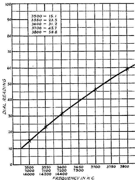
FIG. 6. — HOW TO MAKE UP THE CALIBRATION CHART
