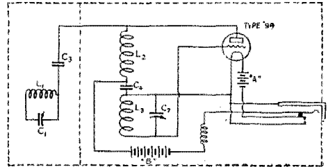
FIG. 4.—THE MONITOR-FREQUENCY METER
