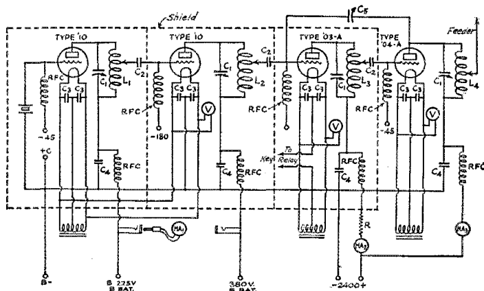
FIG. 1.—THE CRYSTAL-CONTROLLED TRANSMITTER
