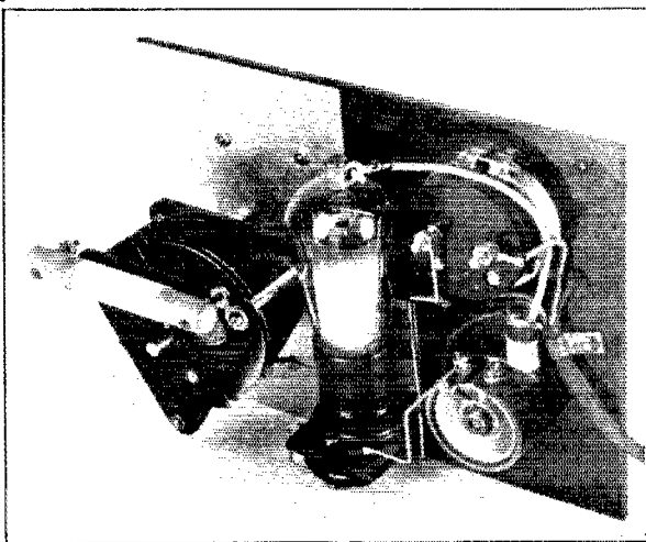
THE FREQUENCY-METER LAYOUT
