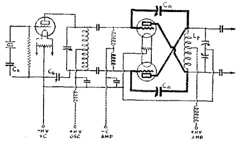
FIG. 3. — A TYPICAL NEUTRALIZED PUSH-PULL AMPLIFIER CIRCUIT
