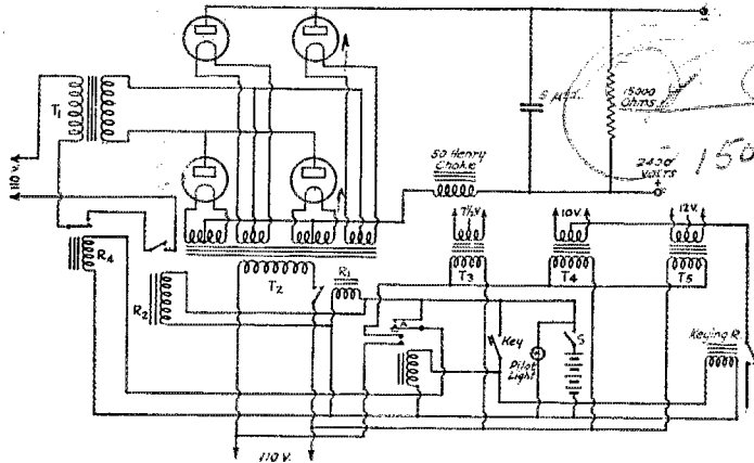
FIG. 2.—POWER SUPPLY AND KEYING SYSTEM The rectifier consists of four Type '66 tubes connected in the usual bridge arrangement.
