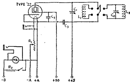
FIG. 7. — A FIVE-BAND FREQUENCY METER
