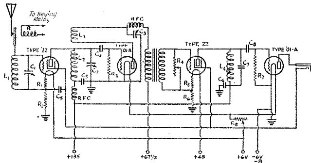
FIG. 3.—THE FOUR-TUBE RECEIVER (For constants see second col., Fig. 1.)
