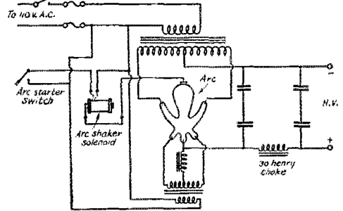
FIG. 2 — THE CONNECTIONS OF THE POWER SUPPLY UNIT
