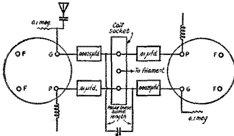
FIG. 5—THE SCHEMATIC DIAGRAM OF THE SUPER-REGENERATIVE CIRCUIT IS GIVEN ABOVE
