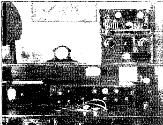
THE OPERATING POSITION AT W8ARO
