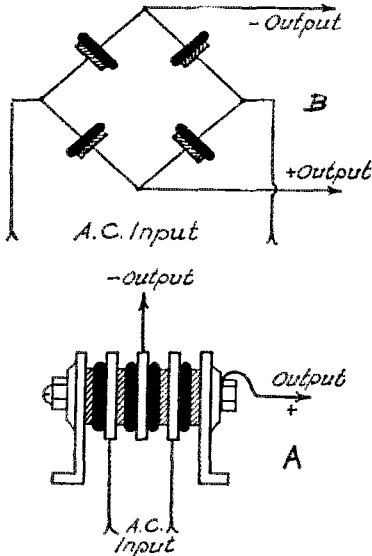
FIG. 2.—THE GENERAL ARRANGEMENT OF A SMALL "ELKON" RECTIFIER USED IN AN "A" SUBSTITUTE IS SHOWN ABOVE
