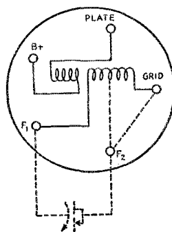
FIG. 2—THE CONNECTIONS TO THE UV SOCKET ARE SHOWN ABOVE
