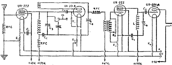
FIG. 3.—THE CIRCUIT OF THE RECEIVER
