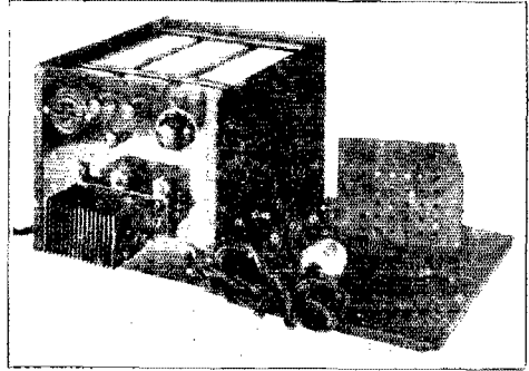
THE "A" BATTERY SUBSTITUTE SHOWN HERE USES AN "ELKON" RECTIFIER UNIT WHICH IS MOUNTED OUTSIDE OF THE MAIN HOUSING FOR BETTER VENTILATION
