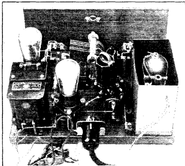
REAR VIEW WITH THE TOP OF THE R.F. SHIELD REMOVED, SHOWING BATTERY CABLE WITH PROTECTIVE LAMP
