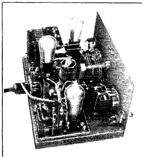
SIDE VIEW WITH TOP AND SIDES OF THE R.F. SHIELD REMOVED, SHOWING THE ASSEMBLY OF THE INPUT CIRCUIT
