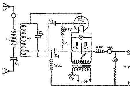
FIG. 1.—THE WIRING OF THE HIGH-C TRANSMITTER
