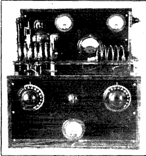
THE SELF-EXCITED HIGH-FREQUENCY HARTLEY TRANSMITTER
