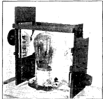
THE LATEST 5-METER LOW-POWER TRANSMITTER AT 8CMP, STATION OF DR. E. C. WOODRUFF, DIRECTOR, ATLANTIC DIVISION
