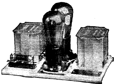
AmerTran Push-Pull Power Stage Type P-1—List price $48 complete with two UX-171 tubes, $54 with two UX-210 tubes. The unit is licensed under R. C. A. Patents and must be sold complete with tubes.
