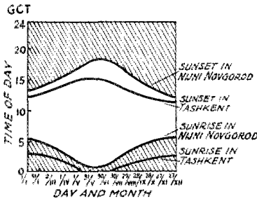
FIG. 11. DIAGRAM SHOWING THE AUDIBILITY OF THE 40-METER SIGNAL IN TASHKENT
