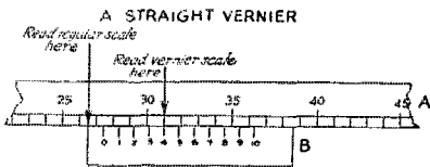
A - Regular Scale B - Vernier Scale, 11 divisions here equal to 10 on main scale METHOD OF READING
