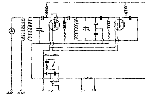
FIGURE 2. THE CENTER TAP METHOD OF FIG. 1 AS USED AT 9BR
