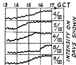
FIG. 9. REAPPEARANCE OF SIGNALS IN TASHKENT IN MARCH, 1926, AT 40 METERS
