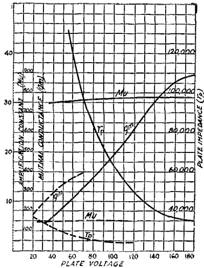
FIG. 2—SHOWING EFFECT OF CHANGING PLATE VOLTAGE ON THE 201-A AND 240 TYPE TUBES
