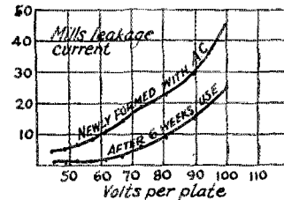
FIG. 4. CONDENSER LEAKAGE
