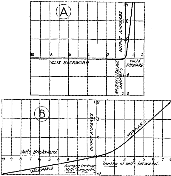
FIG. 5—COMPLETE D. C. CURVES ON RECTIFIER COUPLE Curve A is to the same scale all the way thru and gives a correct idea of the proportions. Curve B has been drawn on a distorted scale to open out the readings. Neither curve gives a correct picture of the a. c. action as is explained by Fig. 6 and the text.
