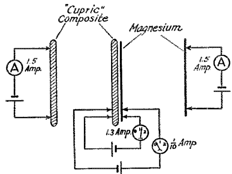
FIG. 4—SHOWING ACTION OF A RECTIFIER COUPLE UNDER D.C. CONDITIONS AT VERY LOW VOLTAGE. THE PERCENTAGES ARE DIFFERENT AT HIGHER VOLTAGE
