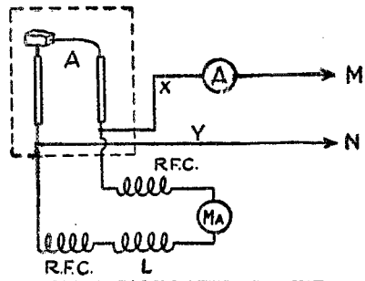
FIG. 2. CALIBRATING CIRCUIT
