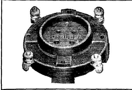
The "Sofrubba" Standard Socket 2 1/2" diameter. Lugs are equipped with N. P. binding posts and are drilled and tinned for soldering.
