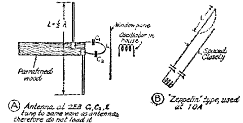
ANTENNAS—NOTE: All may be used with reflectors
