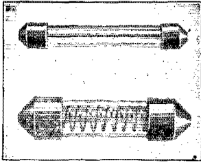
The present standard international resistor of the coated filament type and the new 15 watt resistor unit of the helical type. The resistance element in the latter is a coated glass filament, as in the smaller units.
