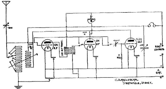
The Circuit That Brings in American Calls. Wiring diagram of the short-wave receiver at 2CM.
