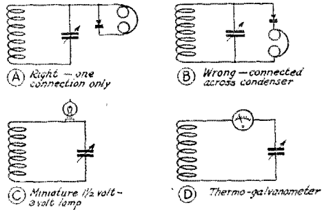
FIG. 3 WAVEMETER CIRCUITS
