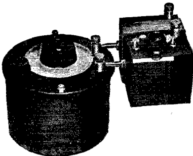
Fig. 1 A Compact Wavemeter and Trap Combined.
