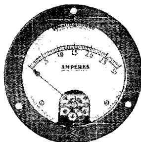
Direct-Current Ammeter, 3-in. Dials, 2 1/2-in. Scales. For Radio Application.
