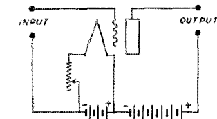
CONNECTIONS FOR R.F. AMPLIFIER WHEN NO STABILIZER IS USED FIG. 12
