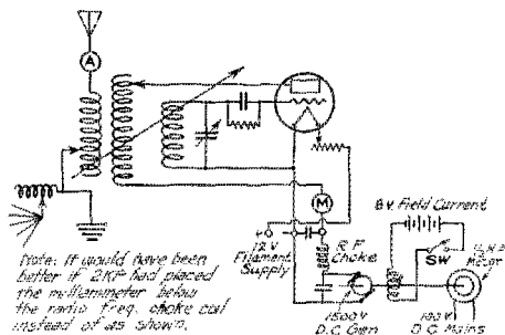
THE WIRING OF BRITISH 2Kf's TRANSMITTER
