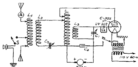
9CCV'S LOOSE-COUPLED TRANSMITTING SET
