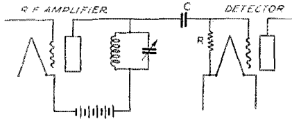
RADIO FREQUENCY AMPLIFIER AND DETECTOR SHOWING CONNECTIONS OF GRID CONDENSER AND GRID LEAK.
