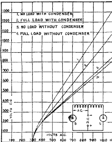
CHART 3 2 TUBES-TAPPED TRANSFORMER
