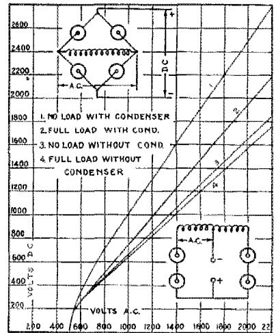
CHART 4 SERIES TUBES BY BRIDGE METHOD OR TAPPED TRANSFORMER
