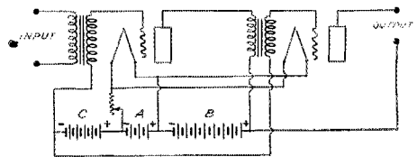
CONNECTIONS FOR TWO AUDIO FREQUENCY AMPLIFIER TUBES SHOWING COMMON BATTERIES
