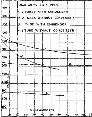
CHART 2 REGULATION 1 & 2 TUBES
