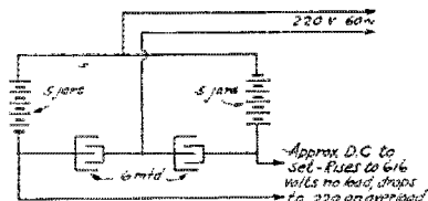
FIG. 3b With condensers rated about 400v on two "E" tubes
