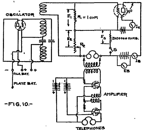
BRIDGE METHOD OF MEASURING AMPLIFICATION CONSTANT.
