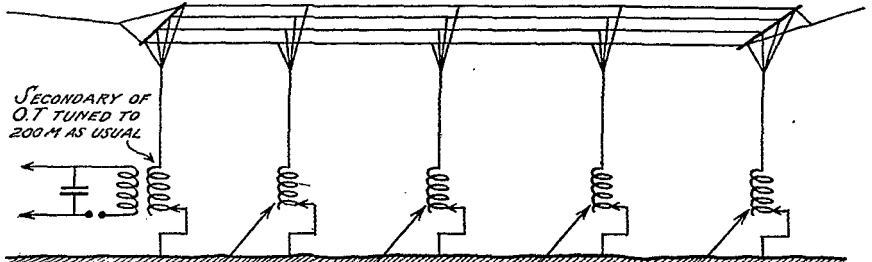
FIG. 4 COILS SITUATED OUTSIDE UNDER AERIAL. LEADS BROUGHT DOWN AND TUNED TO 200 METERS
