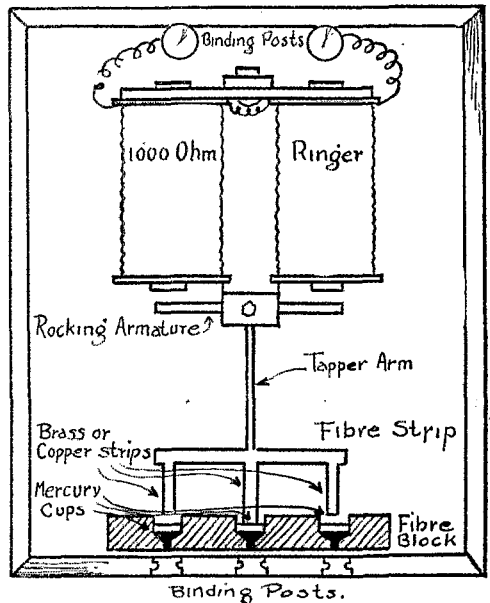
FIG. 1 An Electromagnetic Aerial Switch
