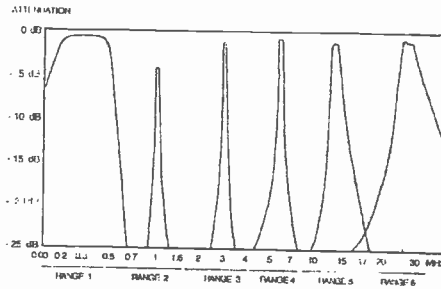
RESPONSE CURVES P-3 PRESELECTOR The response curves in the upper traces 2 to 6 are for approximately midband. The curves center is about over the range with a small overlap into the adjacent ranges. The bandwidth is wider at higher frequencies and smaller at lower frequencies within the same range. See specifications for the 5 dB bandwidth in each range. A 10 dB selective voltage response with 40 dB rejection and less bandwidth, with respect to the peaks shown. Note the significant change in slope 1 or signal strength on a section 6 dB attenuation results. 1.5 dB per octave and 10 dB per octave for comparison and also 20 dB attenuation 10 dB per octave cause 40 dB rejection with section 2. 10 dB per octave and 10 dB per octave for comparison products.
