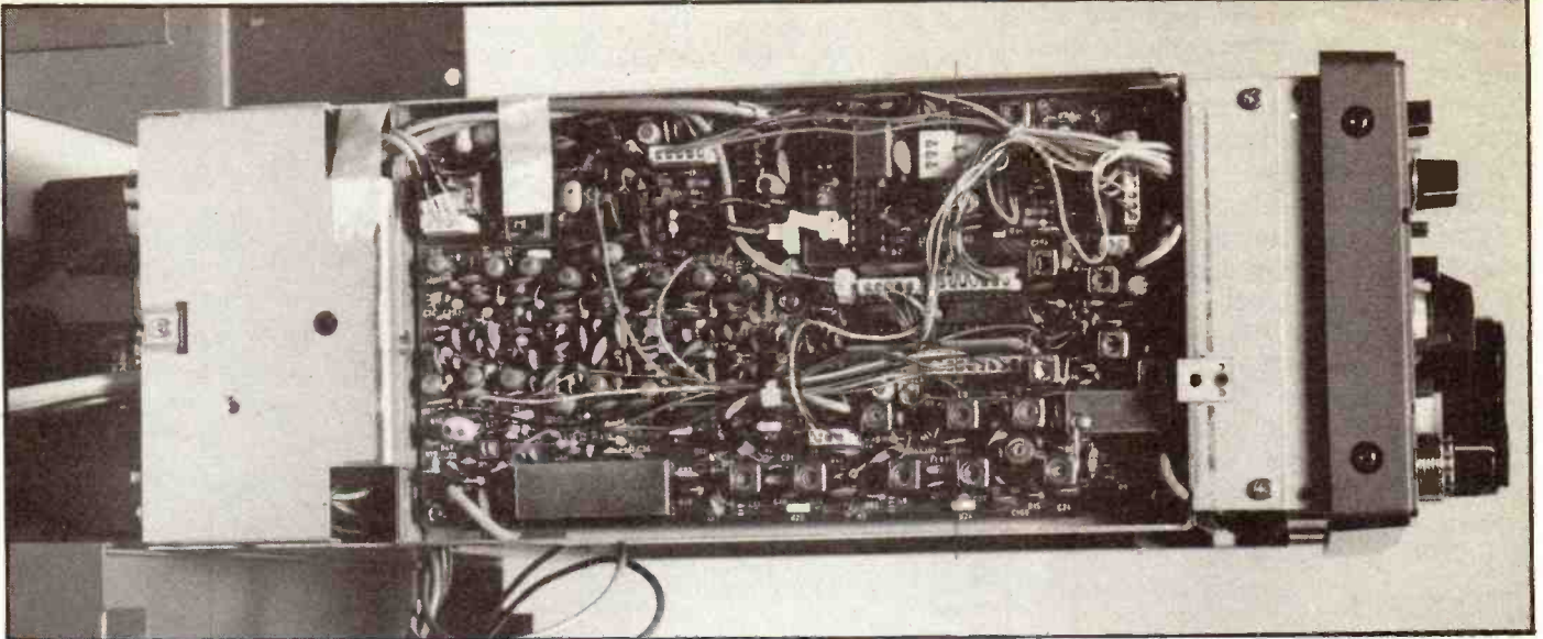
The standard of construction of the IC745 is high, most of the components being mounted on two PCBs, one side mounted, shown here.
