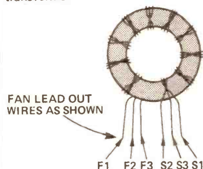
Fig. 1 Constructing T1, the toroid transformer.
