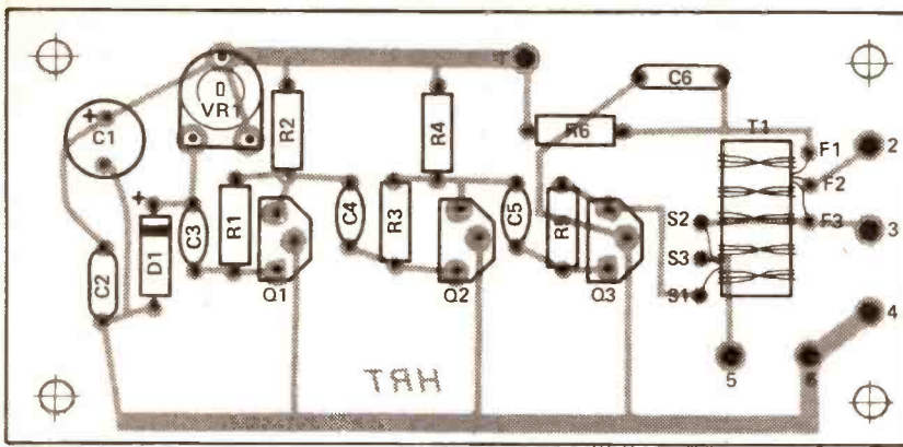
Fig. 2 Component overlay.
