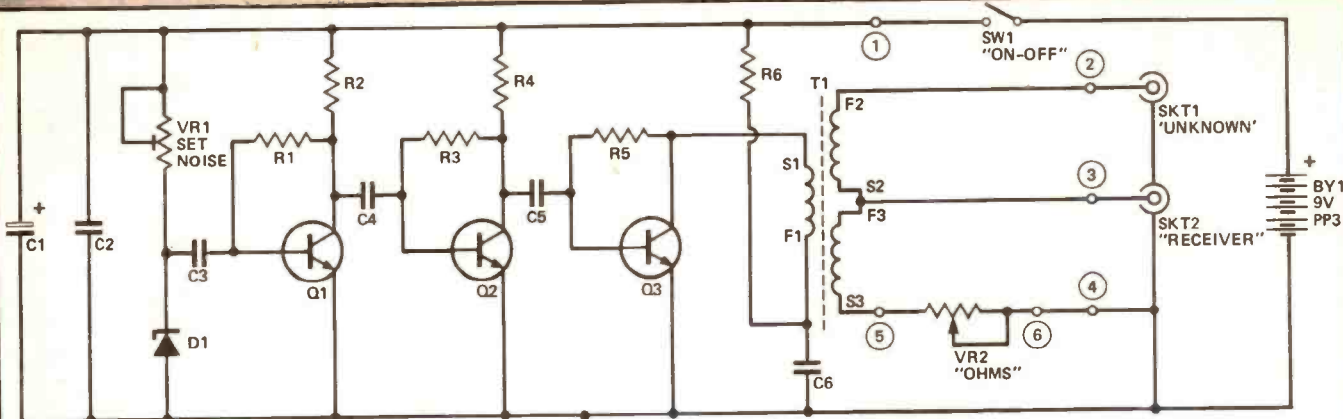
Fig. B Full circuit diagram of the noise bridge.
