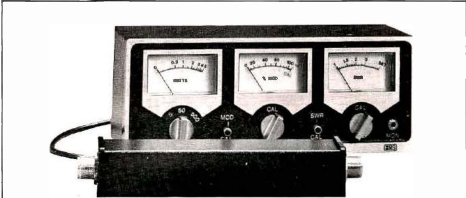
Besides measuring power and SWR, this meter will show the percentage of modulation of an a-m rig. In addition, the front panel monitor jack, with an earphone, lets the user listen to his signal.
