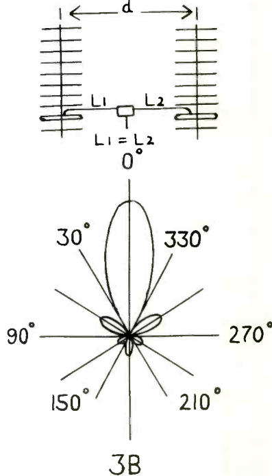
ONE WAVE LENGTH HORIZONTAL STACKING TWO YAGIS
