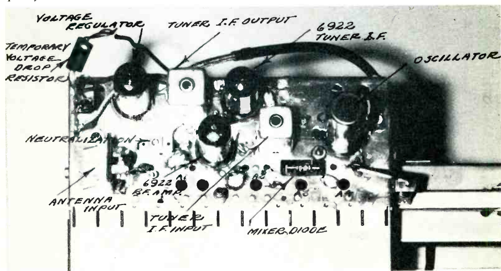
Gould Modified Tuner — 6922 — Diode — 6922
