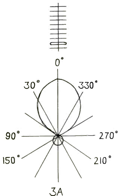
SINGLE YAGI PATTERN
