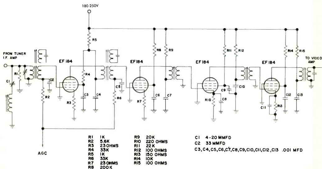
Gould Modified EF184 I.F. Strip
