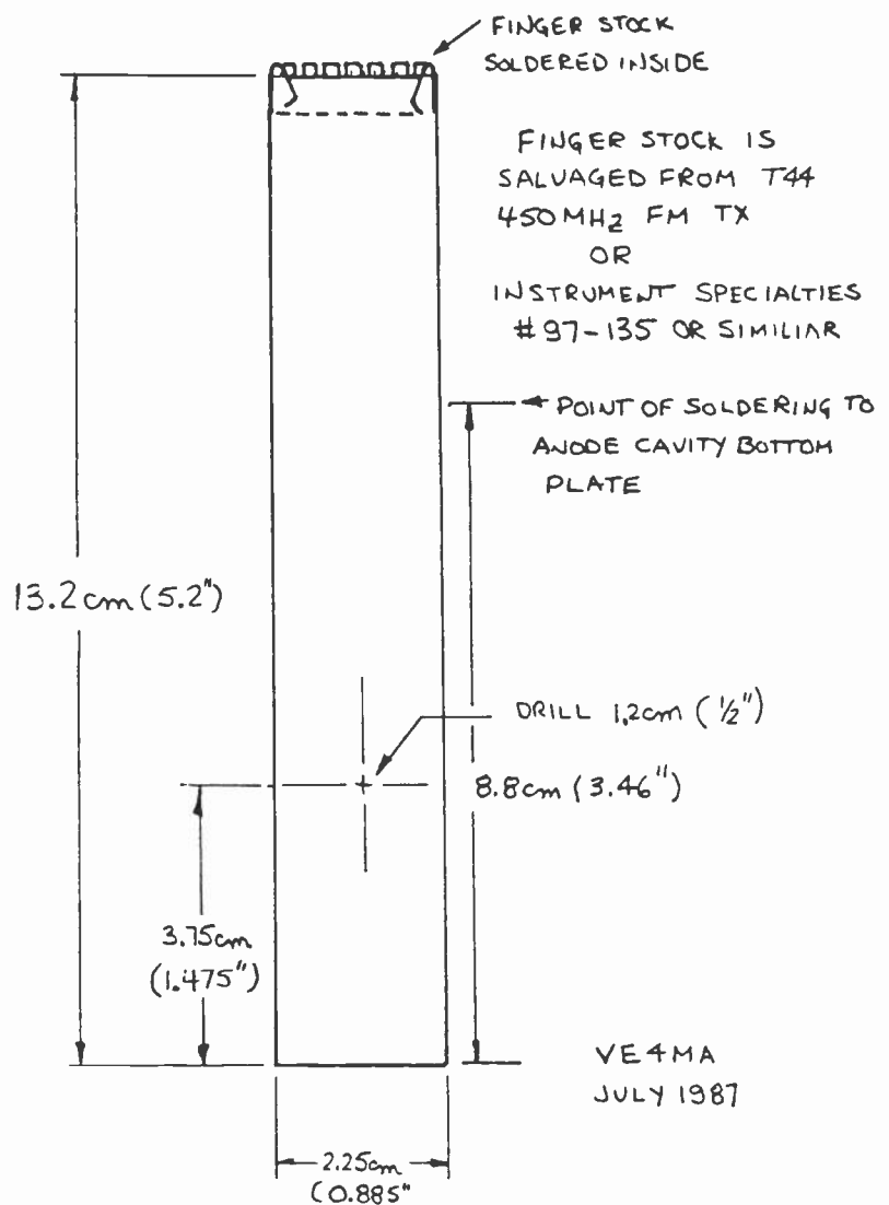
⑩ CATHODE CAVITY OUTER CONDUCTOR
