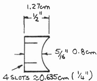
⑧ INPUT PROBE MOUNTING SLEEVE
