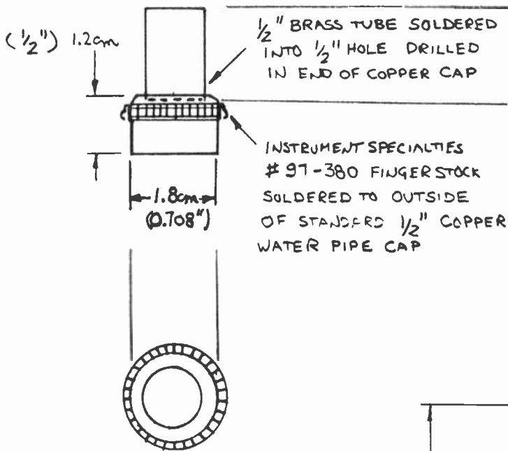
⑥ TUNABLE CATHODE SHORT
