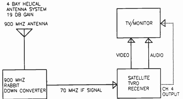
900 MHZ FM-ATV RX SYSTEM
