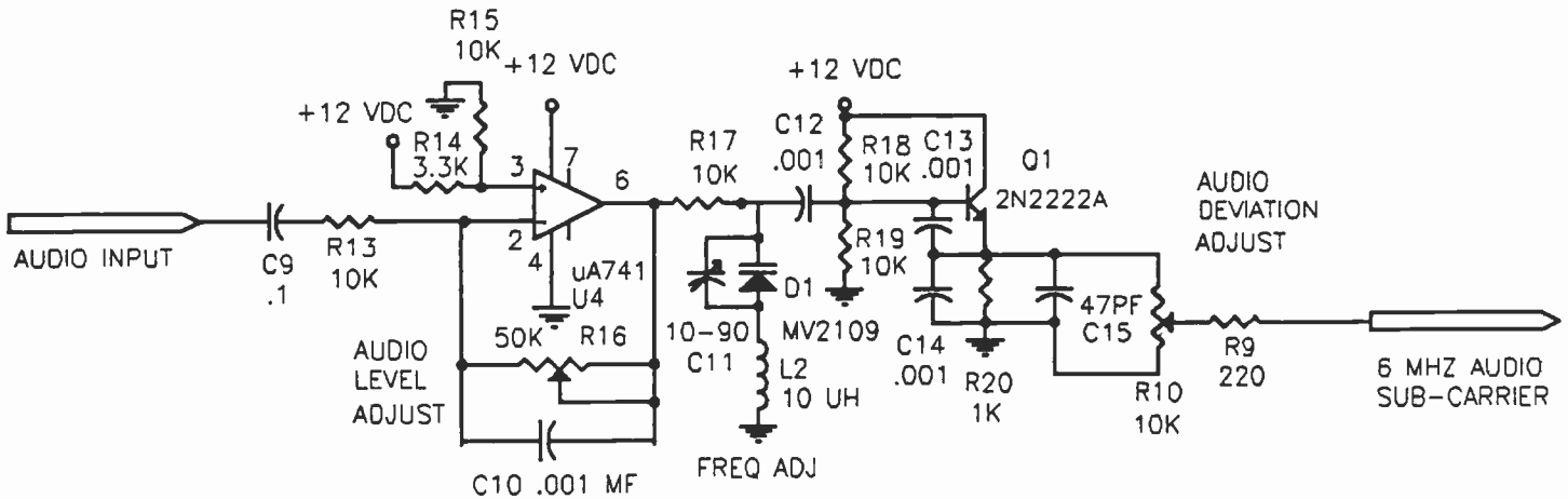
6 MHZ SUB-CARRIER CIRCUIT
