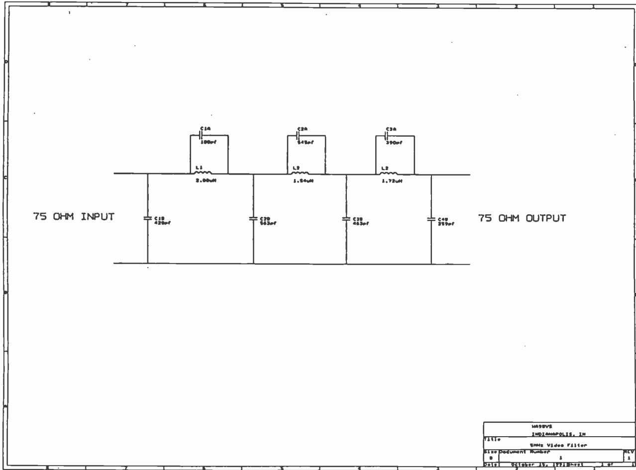
5MHz Filter
