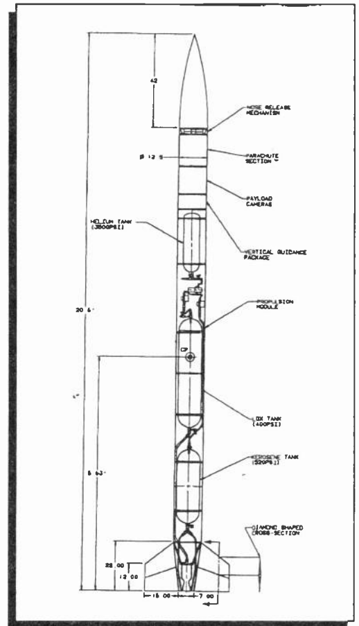
Figure 1. Diagram of David Crisalli's liquid-fuel ATV rocket.
