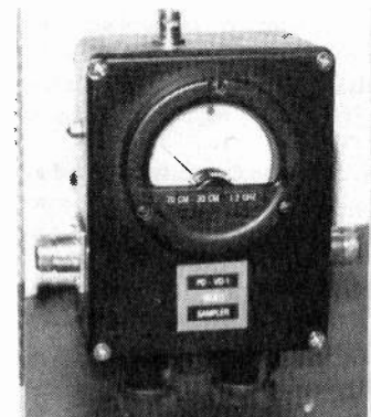
The PAULDON ASSOCIATES Model PD-VB-1 ATV VIDEO SAMPLER unit picks up your transmitted Fast Scan TV signal by sampling the transmission line with near negligible insertion loss. It employs 2 Type "N" connectors for input and output connections. The furnished BNC mentioned on the top of the unit is used as a video output port, useful for connections to a CCTV monitor or scope (for adjusting proper video and sync levels). Transistors included in the electronic circuit design are: O1-ÉCG 123, O2-ÉCG 123 and O3-ÉCG 159.
