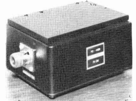
The PAULDON ASSOCIATES Model PD-VB-1 ATV VIDEO SAMPLER unit picks up your transmitted Fast Scan TV signal by sampling the transmission line with near negligible insertion loss. It employs 2 Type "N" connectors for input and output connections. The furnished BNC mentioned on the top of the unit is used as a video output port, useful for connections to a CCTV monitor or scope (for adjusting proper video and sync levels). Transistors included in the electronic circuit design are: O1-ÉCG 123, O2-ÉCG 123 and O3-ÉCG 159.
