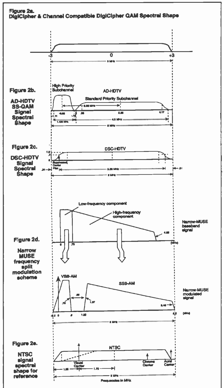
ABOVE: Spectrum of the various HDTV proposed systems. Diagram courtesy TV Technology
