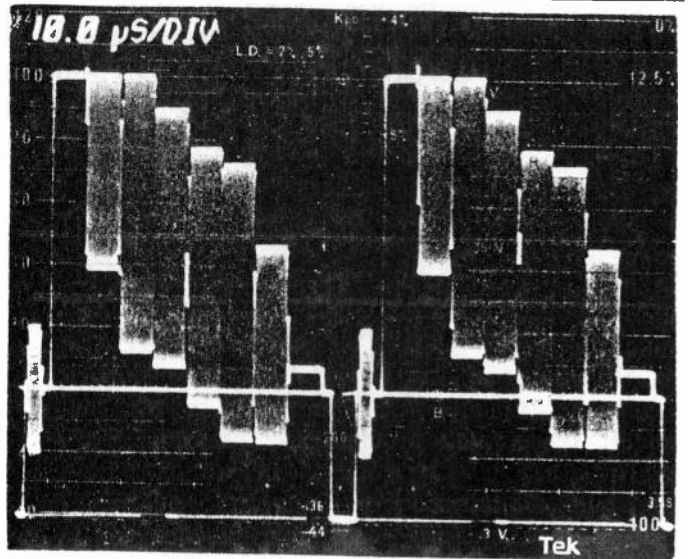
FIG.3a,3b 75% color bars with 100% white and as shown on monitor
