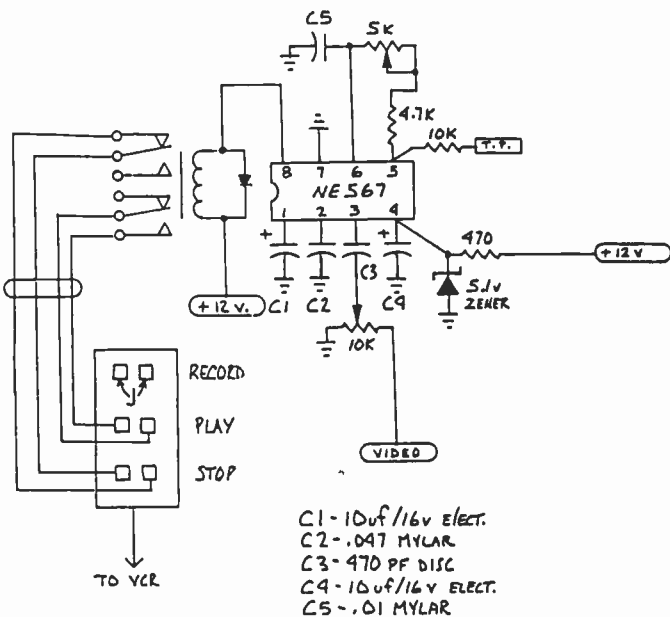
VCR CONTROLLER K6YDW 12-90
