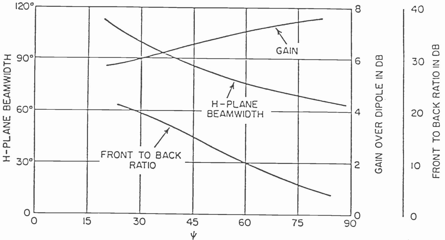
Effect of angle \psi on pattern characteristics. GRAPH #3
