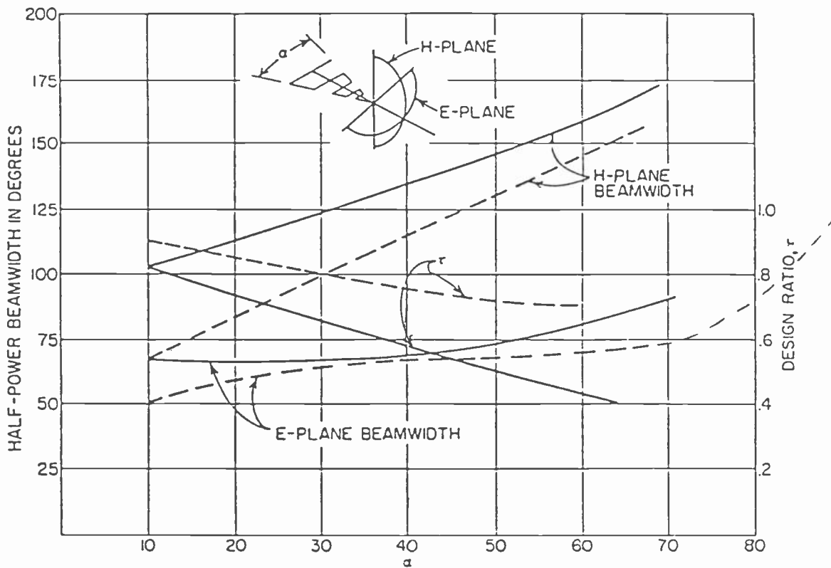
Pattern characteristics of wire trapezoidal tooth element for: ——— Approximate minimum value of r . - - - A larger value of r .
