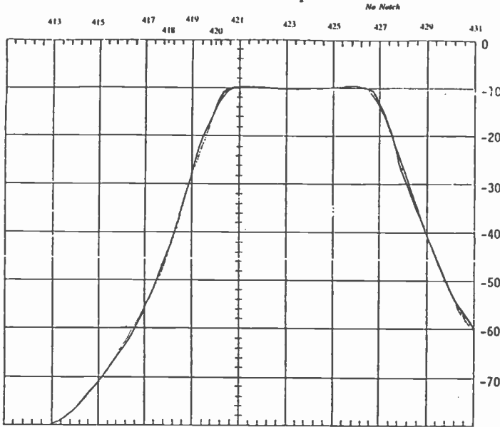
Interdigital B.P. Filter Response.
