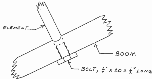
Element to Boom Attachment Figure
