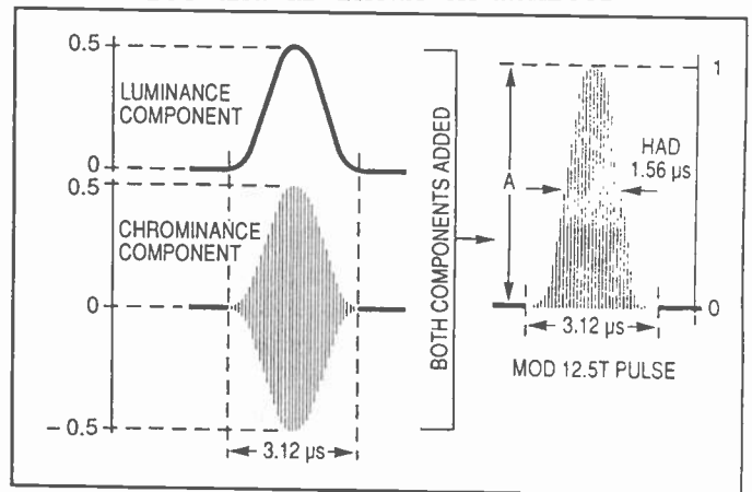
FIG.6 Chroma & Luma components of the modulated 12.5T pulse.
