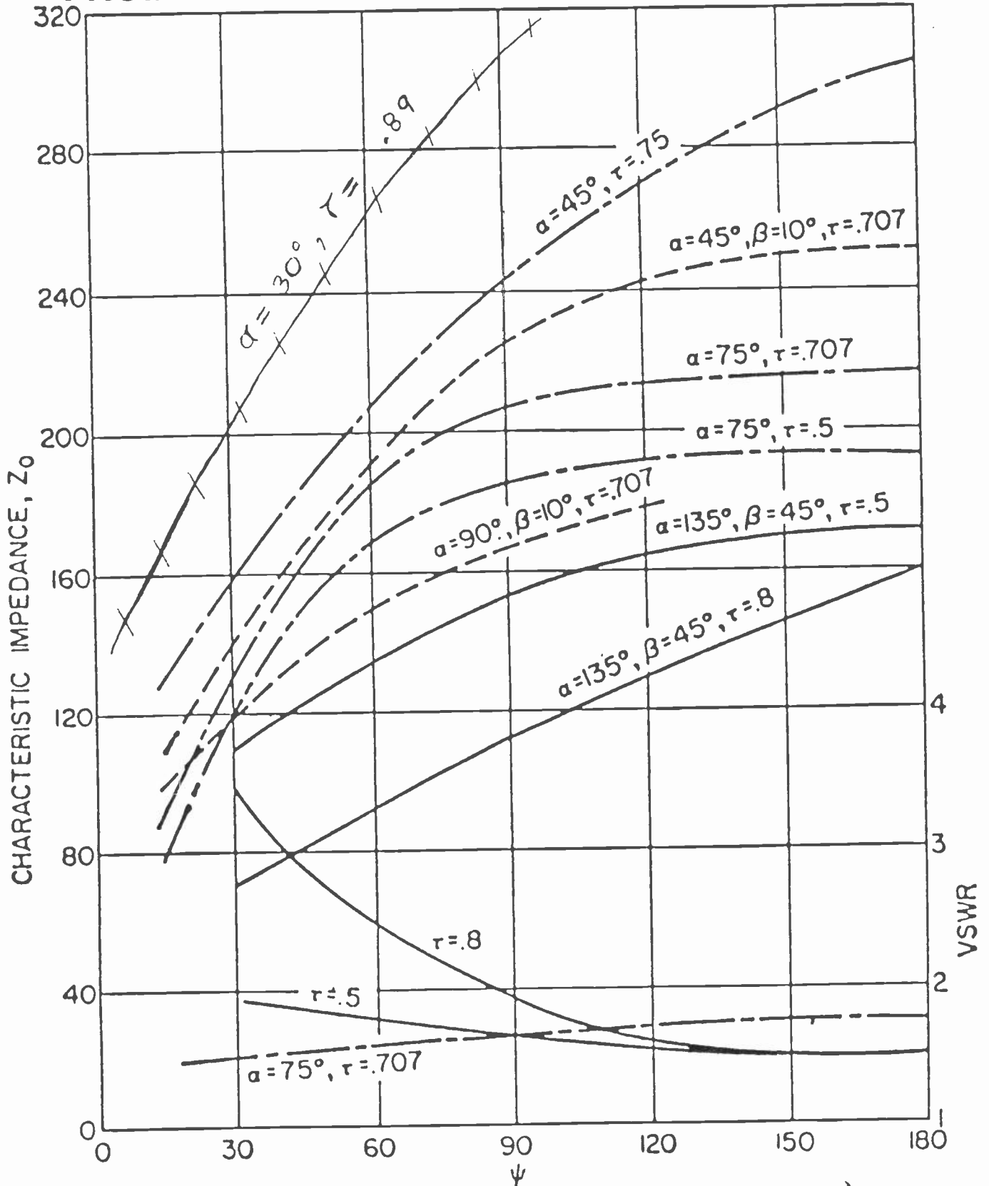
Variation of Z_0 and VSWR with \psi , Circular teeth (---) Trapezoidal teeth (-.-.-), Wire Trap. teeth (— — —) Dipoles - interpolation (+ + +)
