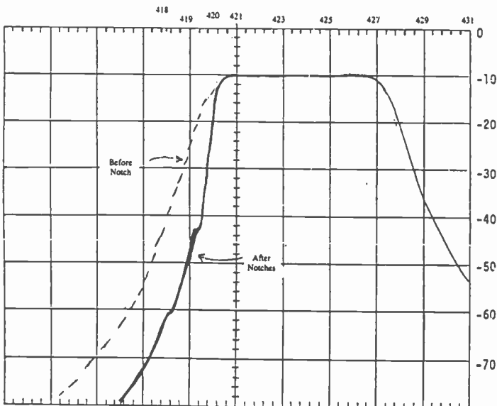
BPF & NOTCHES COMBINED
