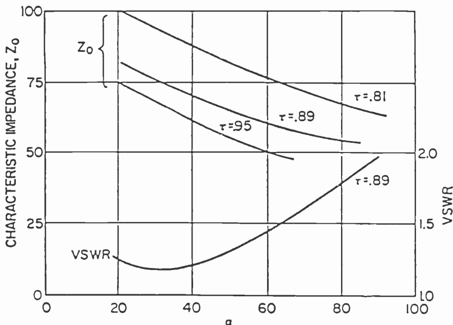
GRAPH #1 Variation of Z_0 and VSWR with \alpha for log-periodic dipole array
