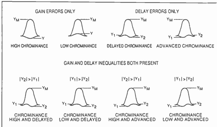
FIG.7 Gain and Delay Distortions on 12.5T
