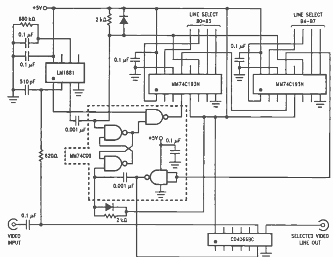
FIG.1 Test Pattern Selector
