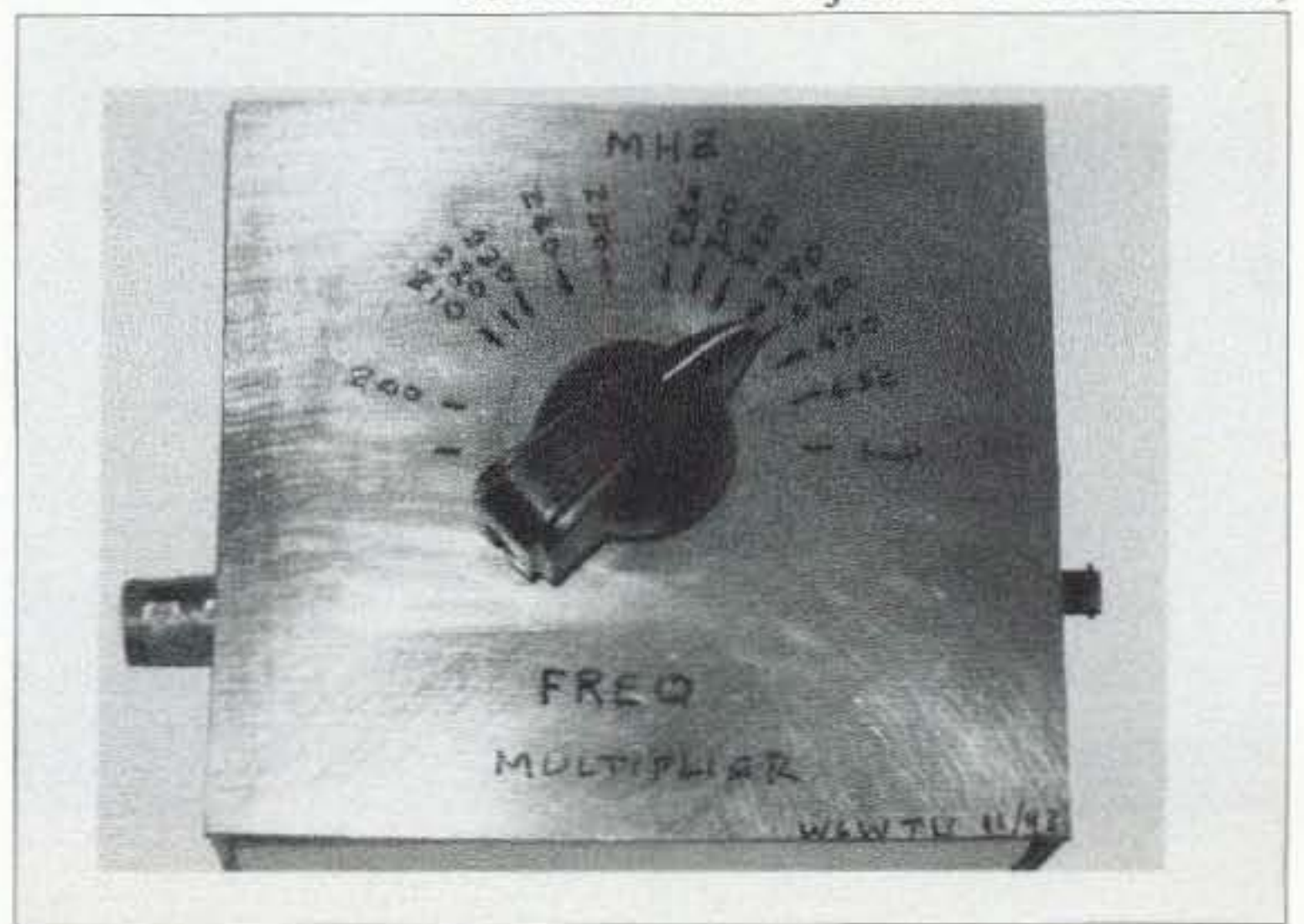
Photo P. A dial hand-drawn onto a panel face. The pointer knob is attached directly to a capacitor's shaft.
