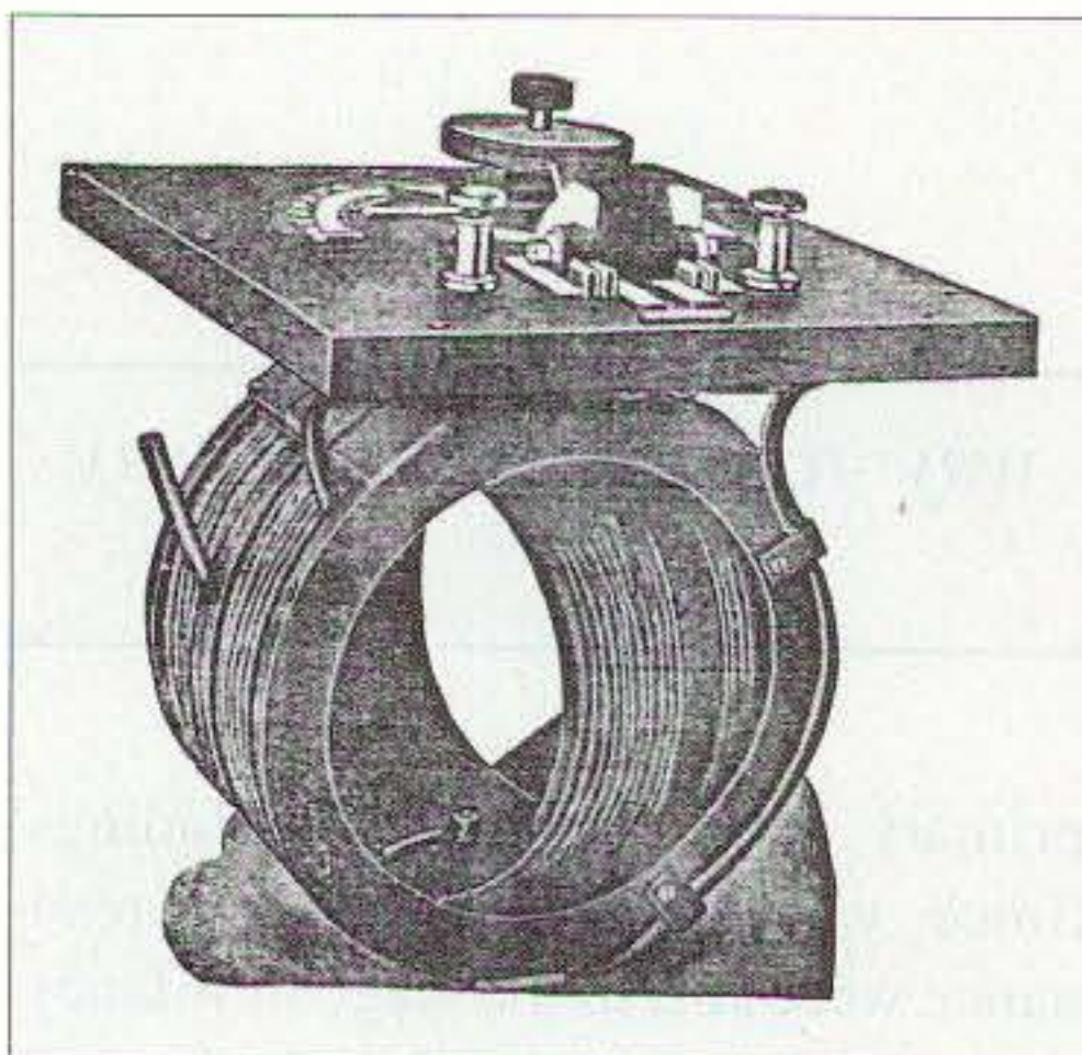
Photo D. This is a variometer. One winding is allowed to rotate within another. A tap switch is provided to change/control the turns ratio. (Photo ref. 2, pg. 80)
