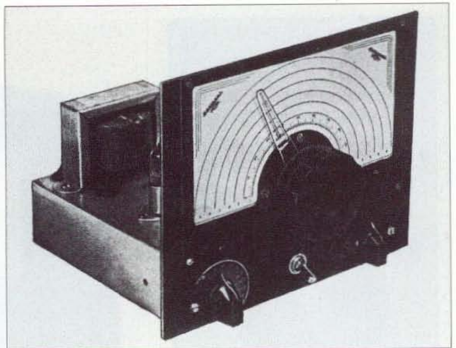
Photo R. A National ACN dial. A smaller version, MCN was also produced. This dial utilized a Velvet Vernier planetary drive mechanism. (Photo ref. 4, pg. 42)
