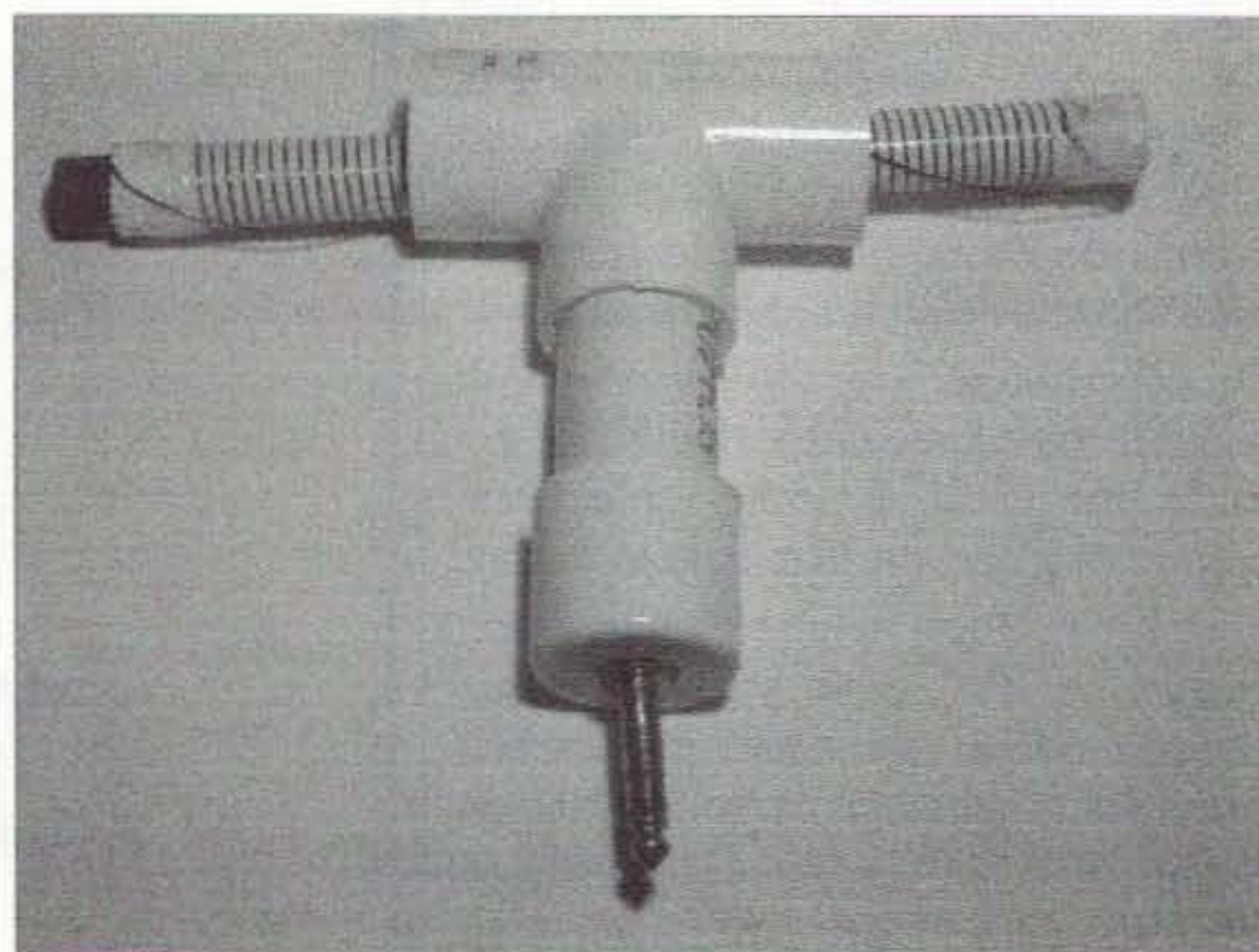
Photo L. Ferrite coil antenna with ends removed.
