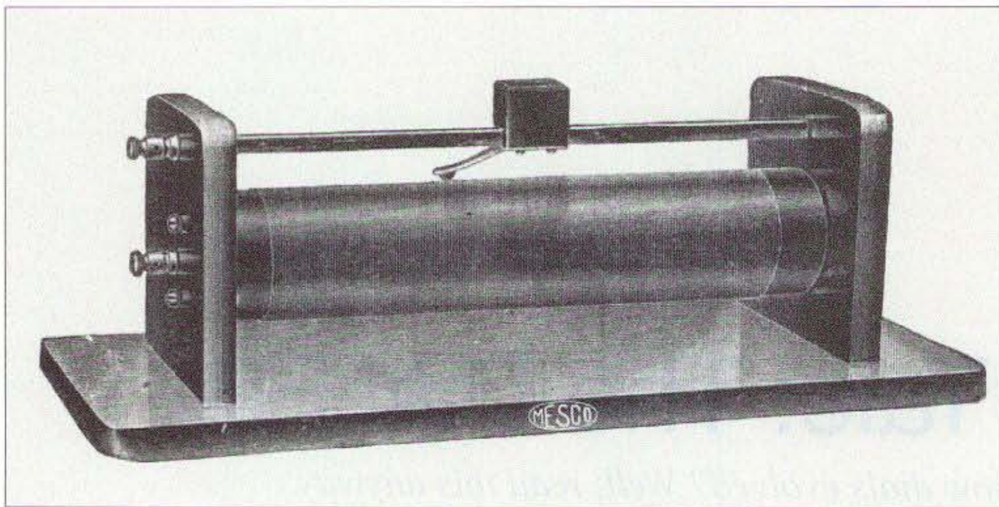
Photo C. This is a single RF inductor having a single slider. (Photo ref. 1, pg. 2308)
