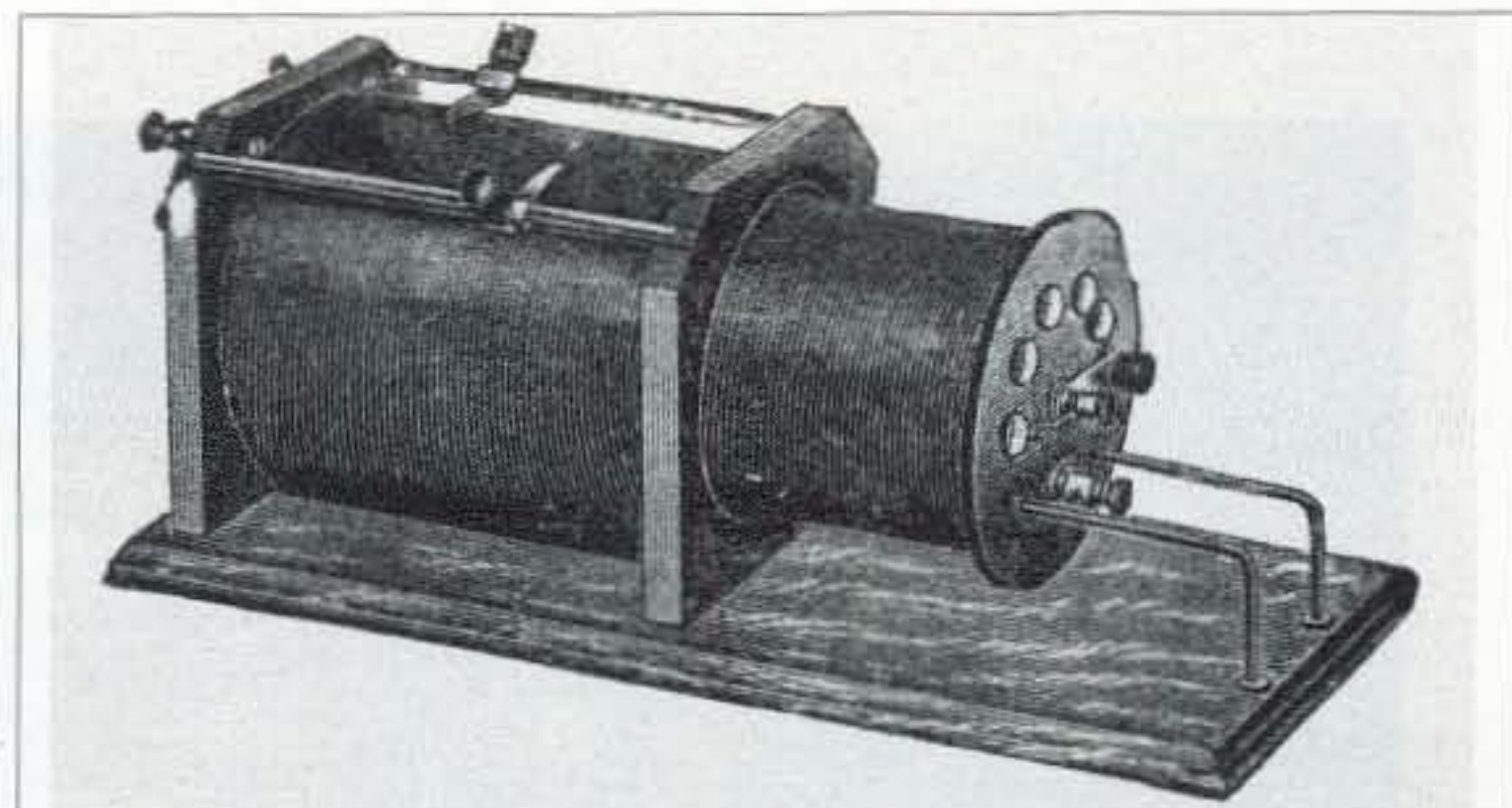
Photo B. This is an RF transformer exhibiting the typical tap switch and slider adjustments. In addition, one winding is capable of sliding along a set of rails providing control over the coupling factor. (Photo ref. 1, pg. 2310)
