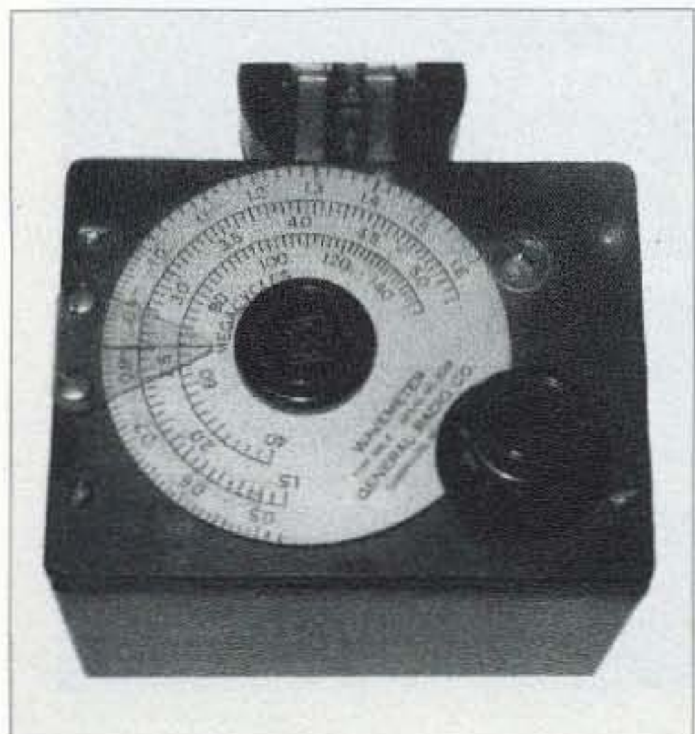
Photo O. A flat friction-driven dial as was used on a General Radio wavemeter.
