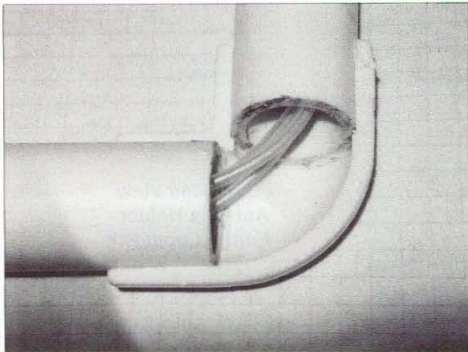
Photo I. 90-degree elbow with turn loop.
