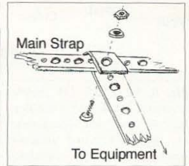
Fig. 4. Tapping into the main grounding strap for connection to an individual piece of equipment.
