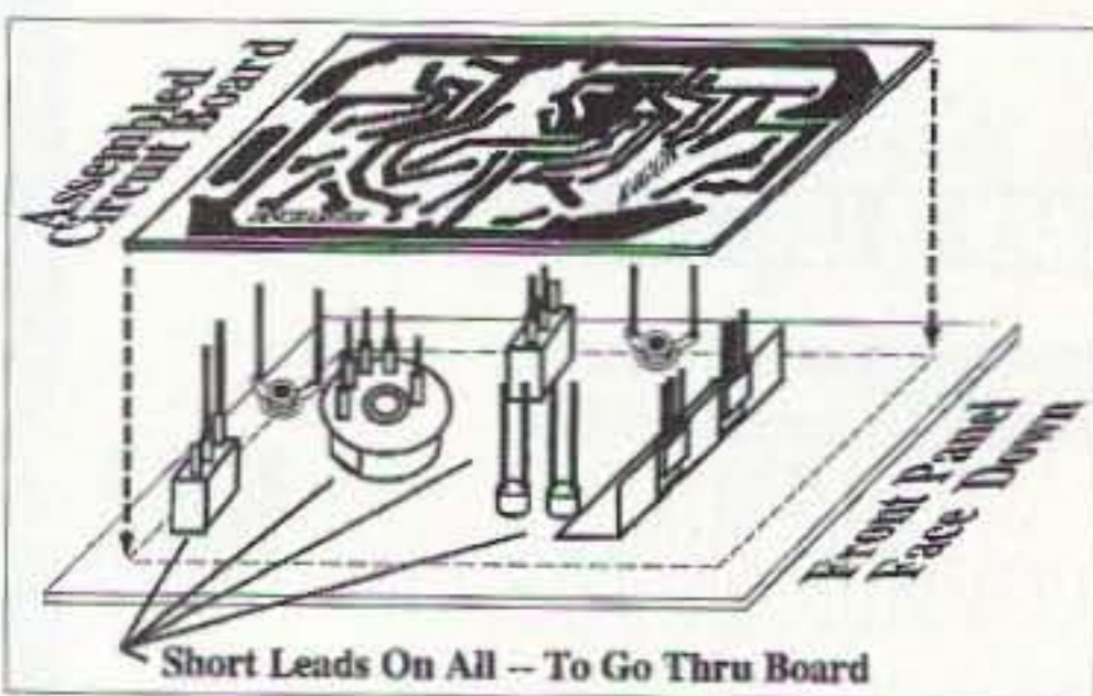
Fig. 6. Suggested assembly sequence
