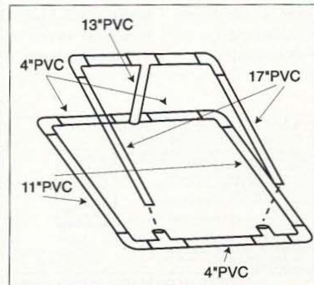
Fig. 2. Final assembled frame.
