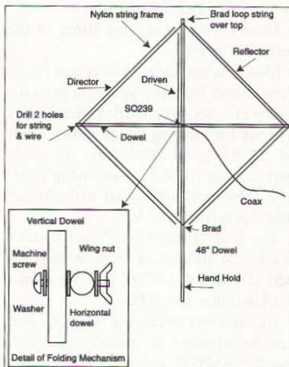
Fig. 1. Construction details for the 2 meter diamond beam.
