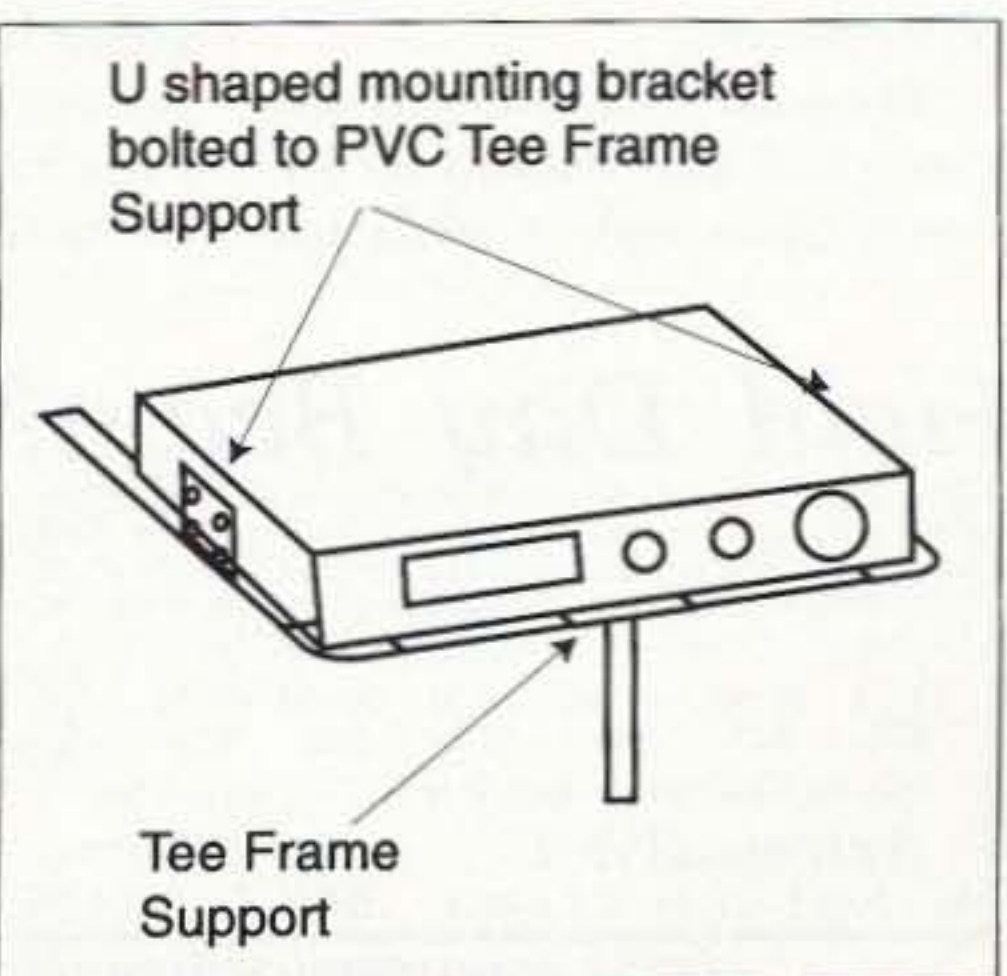
Fig. 3. Mounting radio to frame.
