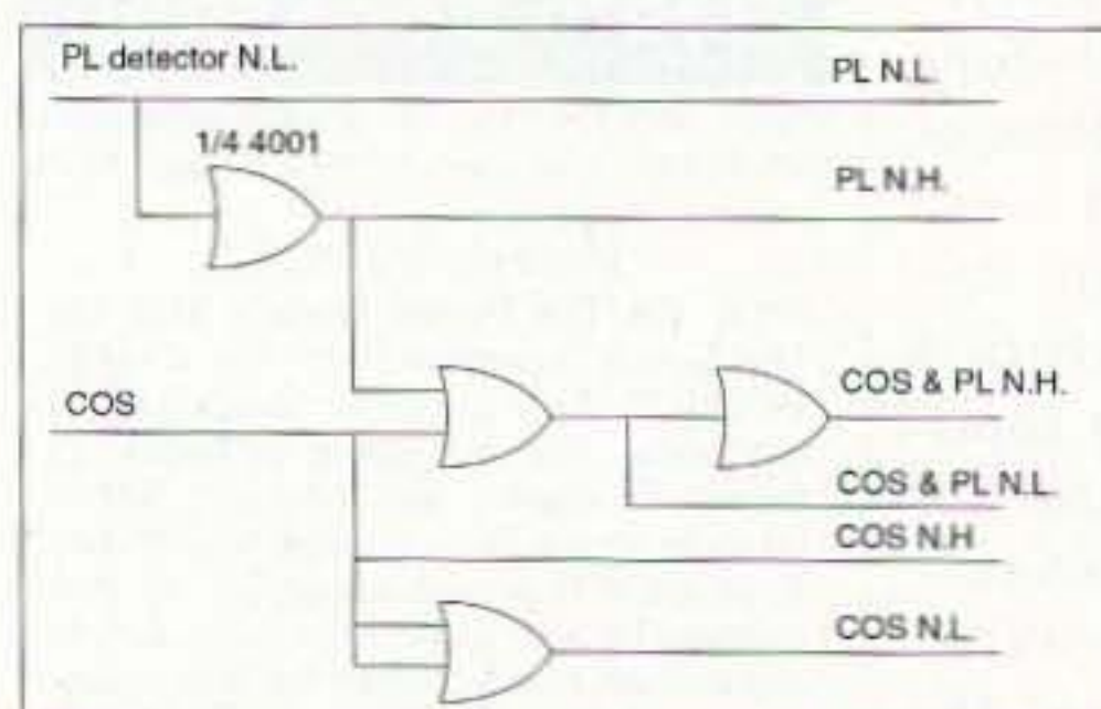
Fig. 1. The CMOS gate wiring.
