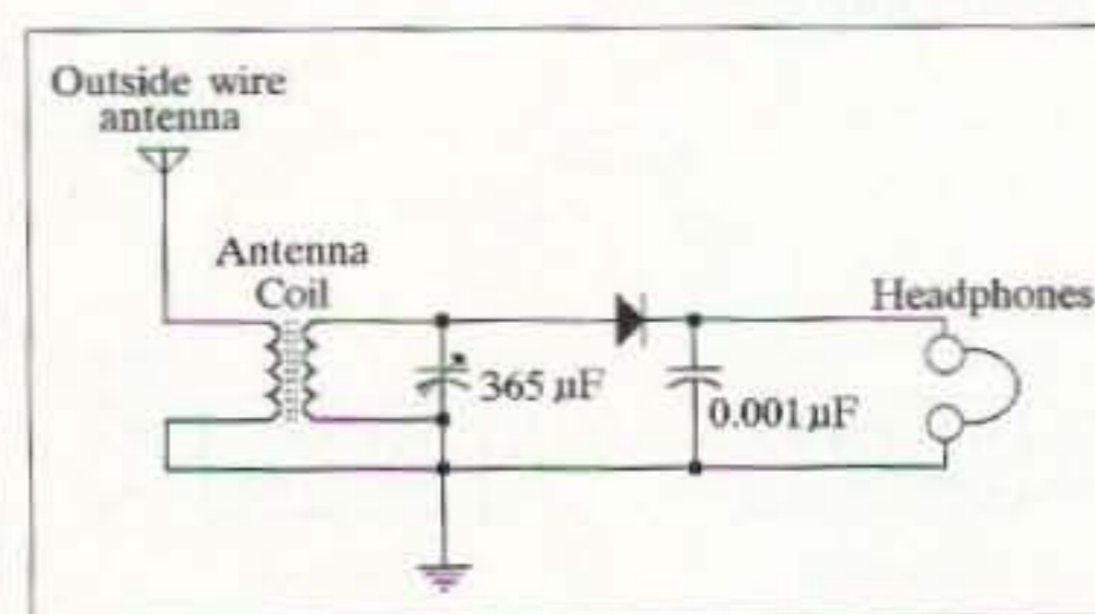
Fig. 4. A crystal radio receiver.
