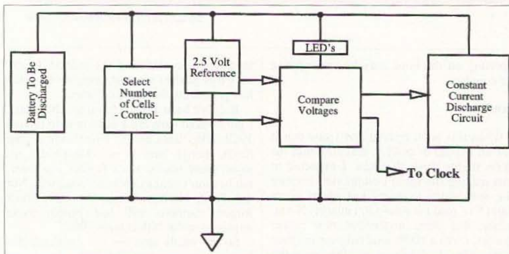
Fig. 1. Discharger block diagram.
