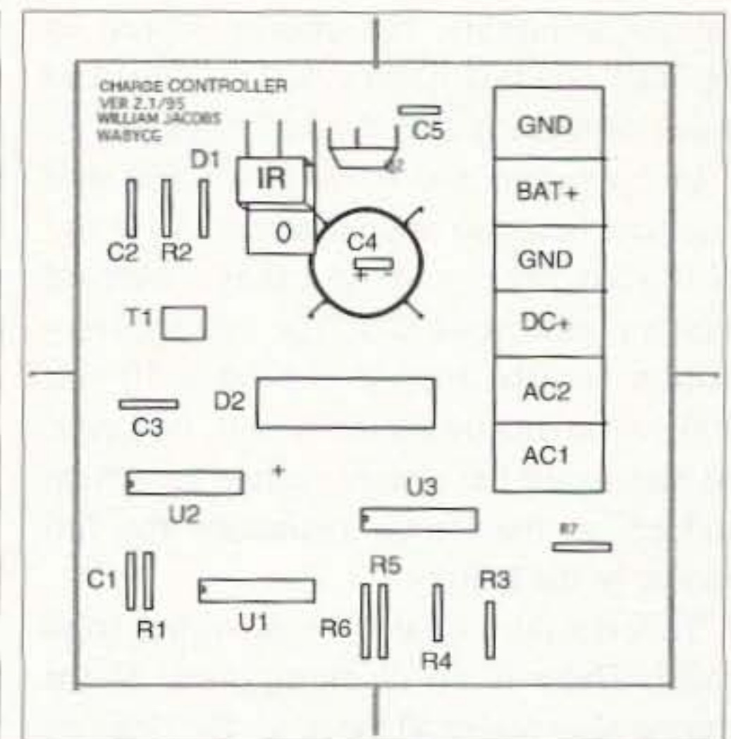
Fig. 2. Silk-screen pattern.
