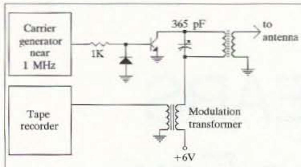
Fig. 5. A simple AM transmitter lab experiment.
