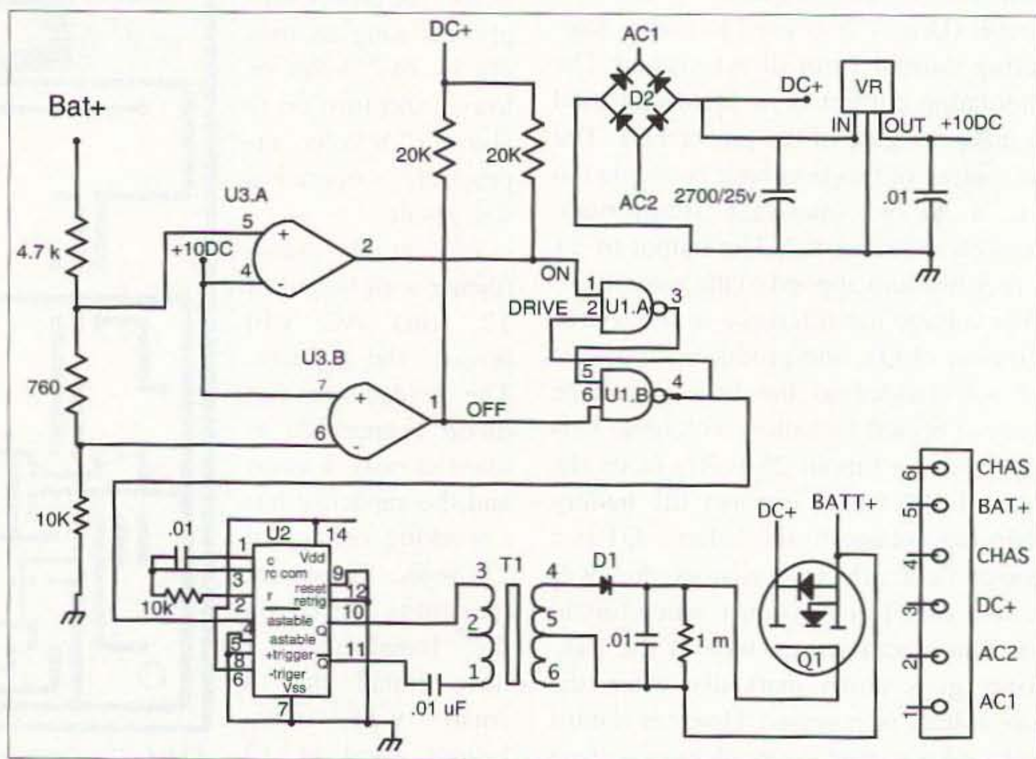
Fig. 4. Charge controller schematic.
