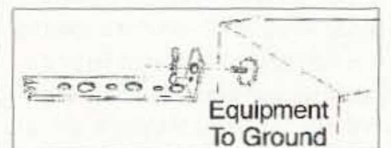
Fig. 5. Connection to the actual piece of ham gear at its rear ground stud. If a direct connection via the steel strapping isn't practical (because of the need to pull a particular piece of equipment out to gain access to the rear apron), then a short piece of flexible braid with a terminal lug installed on it (such as the braid from the inside of an RG-8 coax cable) can be used as a jumper to the main strap.
