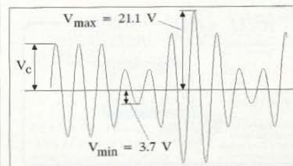
Fig. 7. Calculating the modulation percentage.
