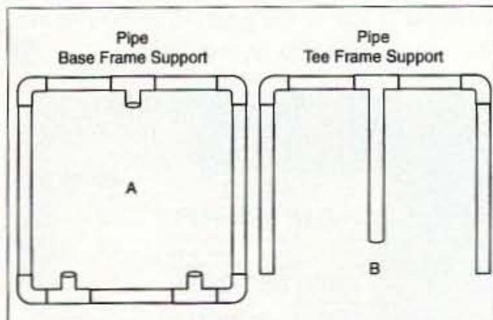
Fig. 1a. Pre-assembled frame: pipe base frame support.
