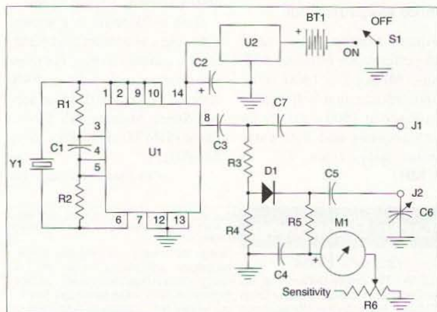
Fig. 1. Schematic diagram.
