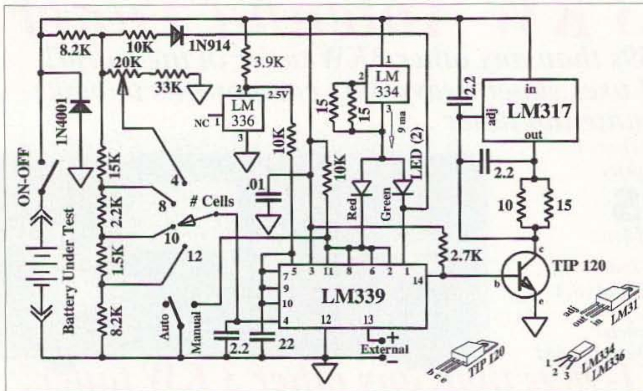
Fig. 2. Discharger schematic.
