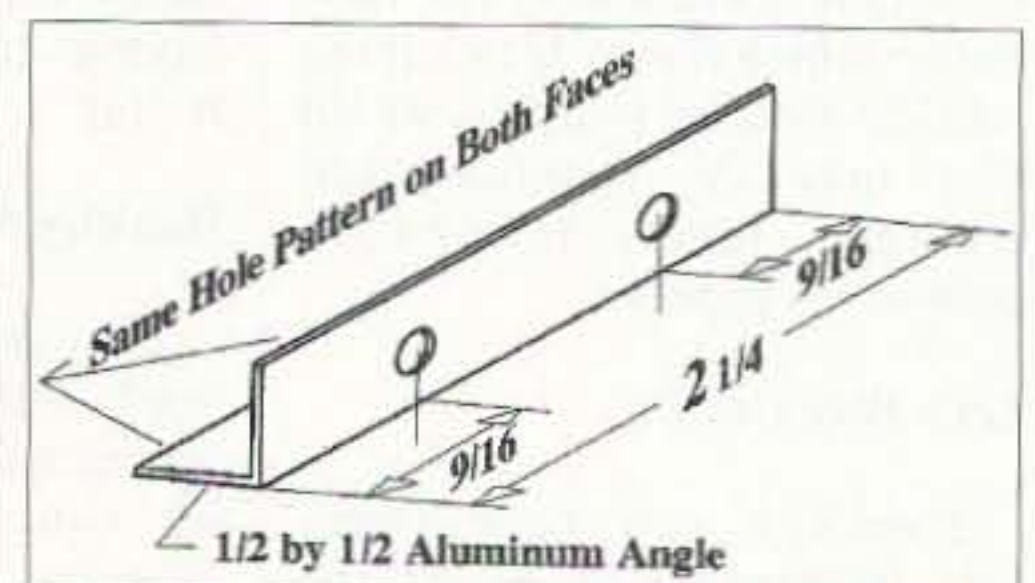
Fig. 7. L-mounting bracket.
