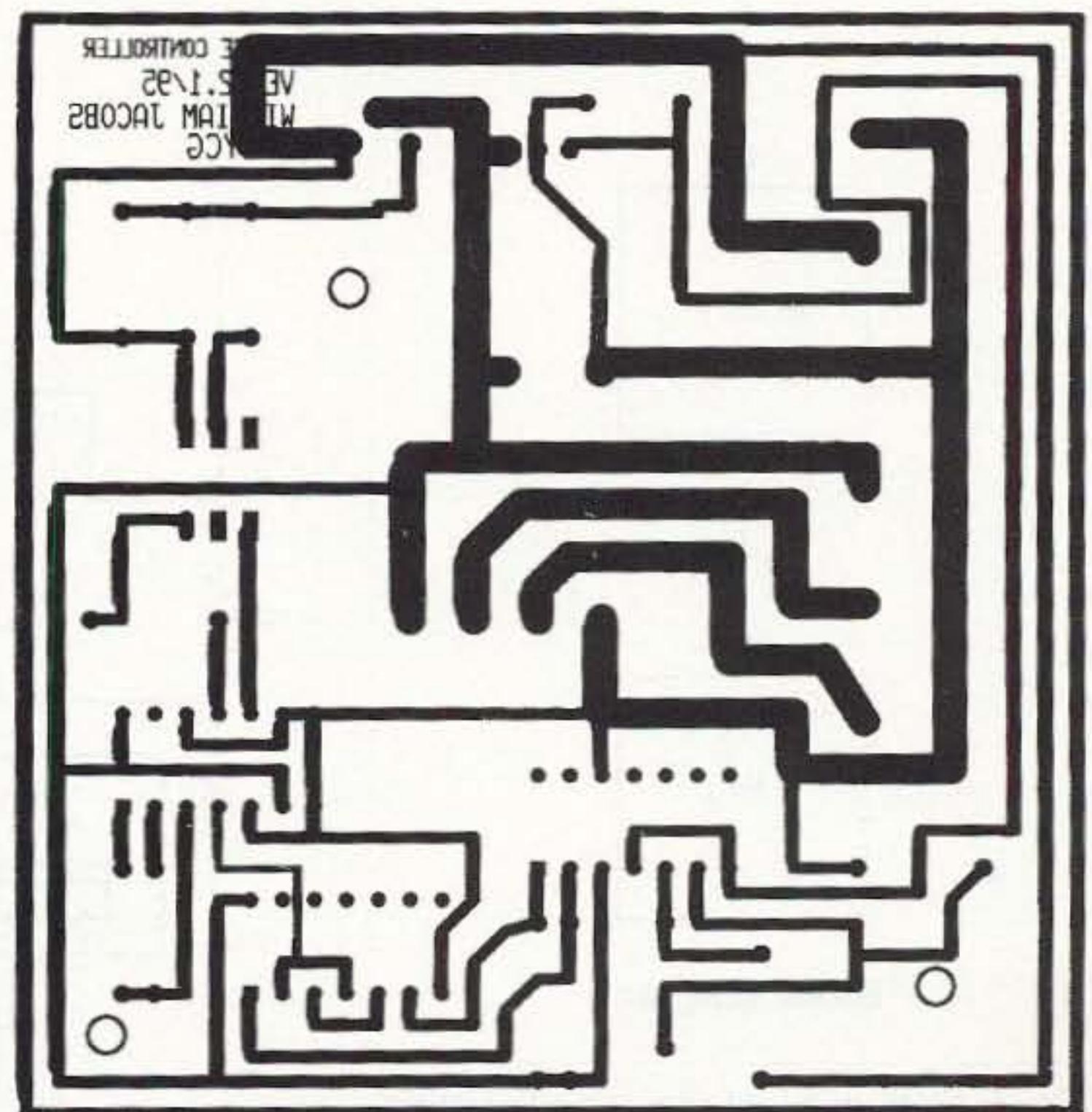
Fig 1. PC Pattern from the top of the board. When the board is printed, the text will be "correct reading."
