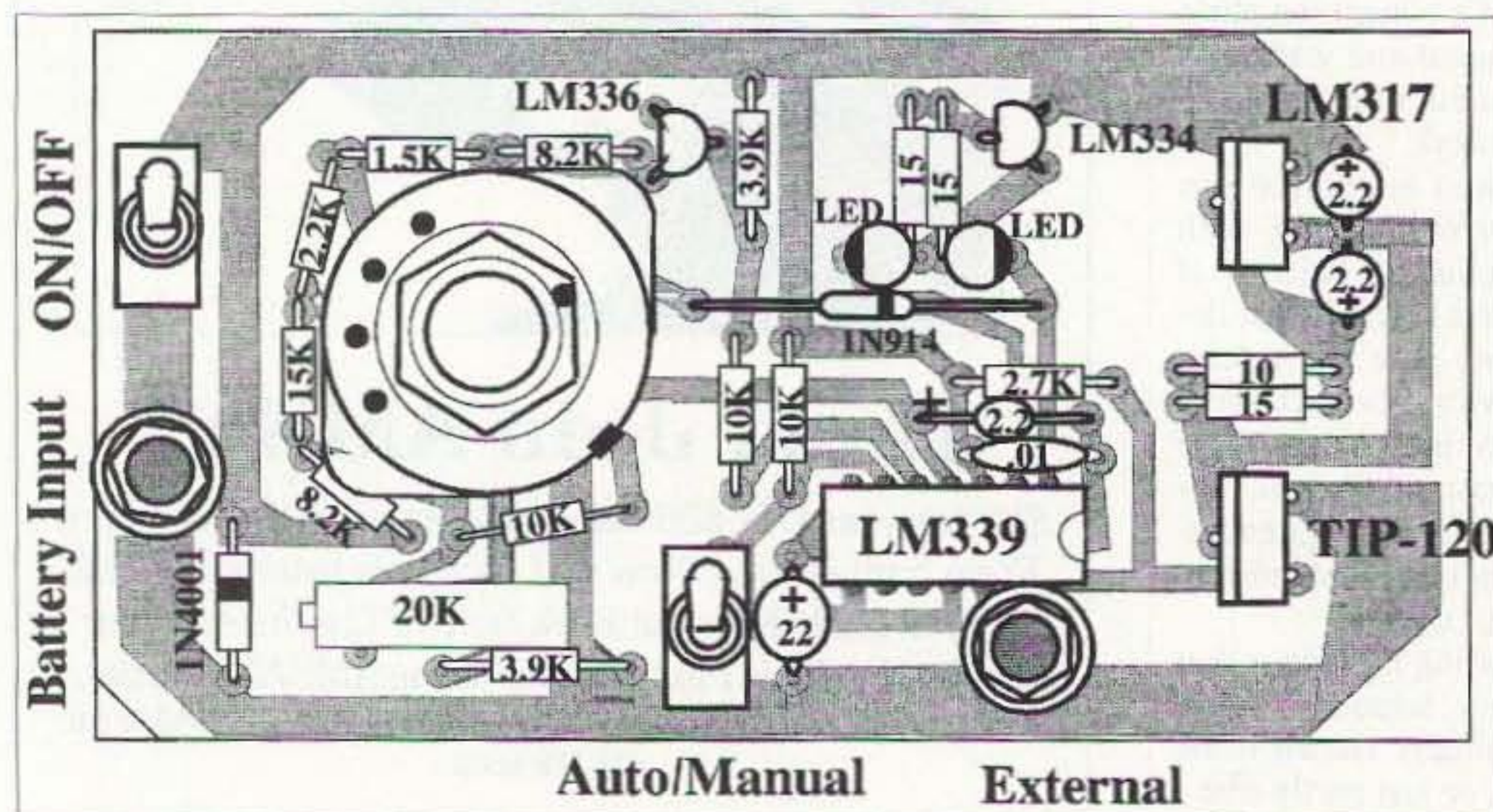
Fig. 5. Parts placement diagram.
