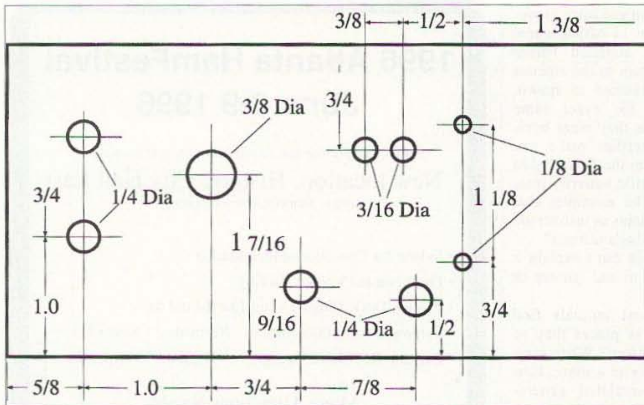
Fig. 4. Drill hole pattern for a 5" x 2.5" panel.
