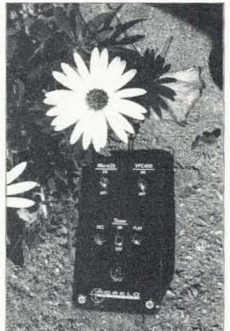
Photo B. This little hidden T has gotten a workout during practice sessions for on-foot foxhunts at Hamcon-95 and the West Coast VHF/UHF Conference. It contains a digital voice recorder, timer board, and 190-milliwatt transmitter, all sold by Agrelo Engineering. Four AAA alkaline batteries power it.
