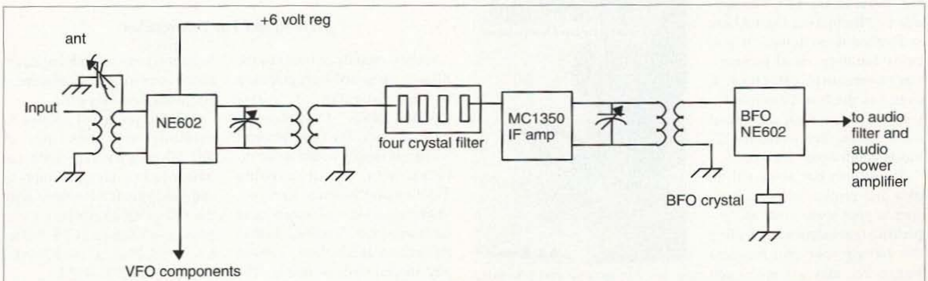
Fig. 1. Block diagram of the 15 meter CW transceiver.
