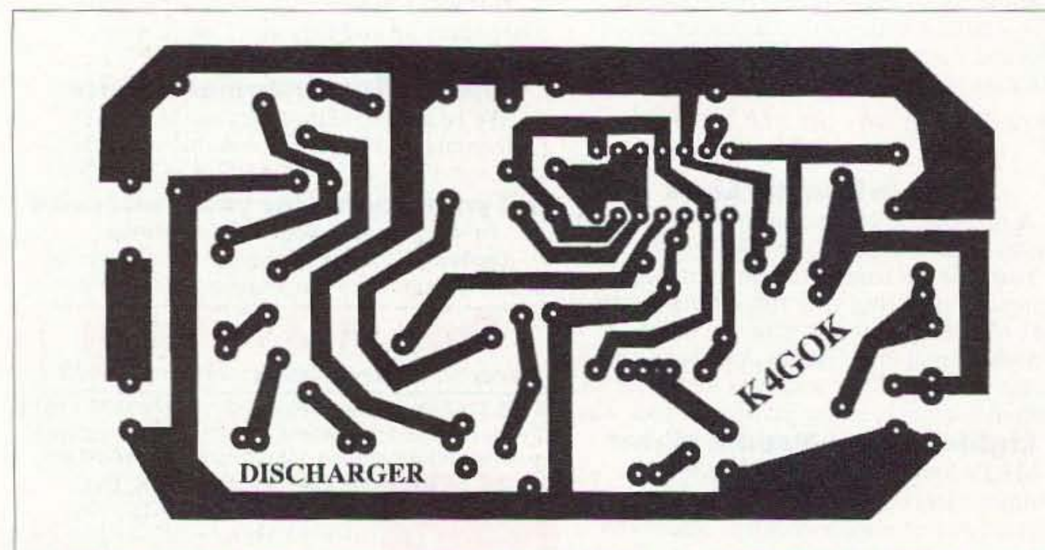
Fig. 3. PCB layout pattern.
