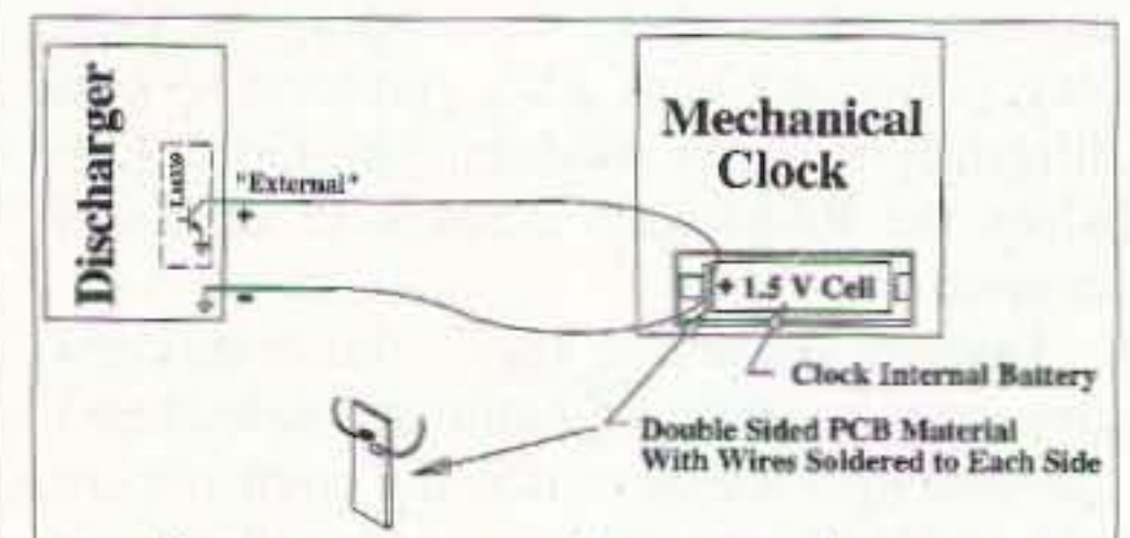
Fig. 8. Clock timer connections.
