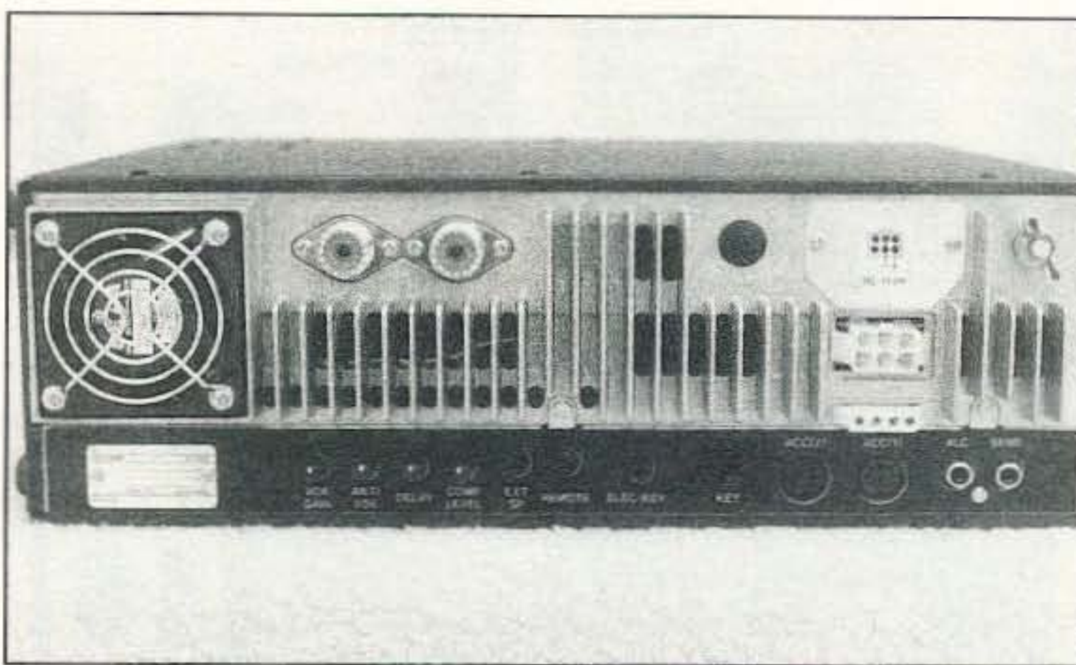
Photo B. Rear View of the IC-738. The two side-by-side SO-239 coaxial receptacles are for two antenna connections. The cooling fan to the left side of the photo is one of two cooling fans used to keep the unit loafing along even at continuous duty at full power.
