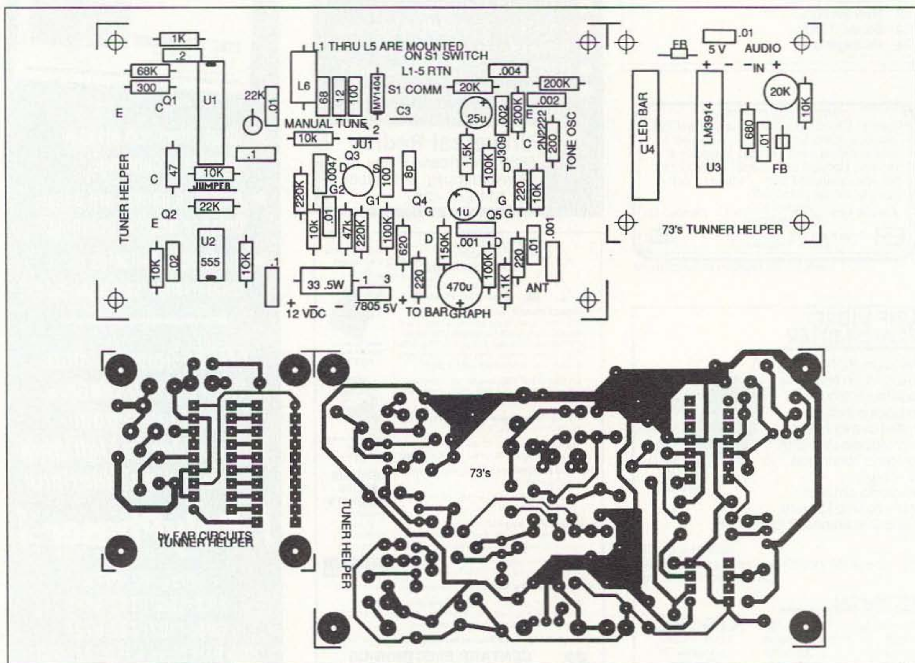
Figure 5. Printed circuit board layout. Pre-made boards are available for $6.00 cash plus $1.50 S&H per order from FAR Circuits, 18N640 Field Ct., Dundee, IL 60118.
