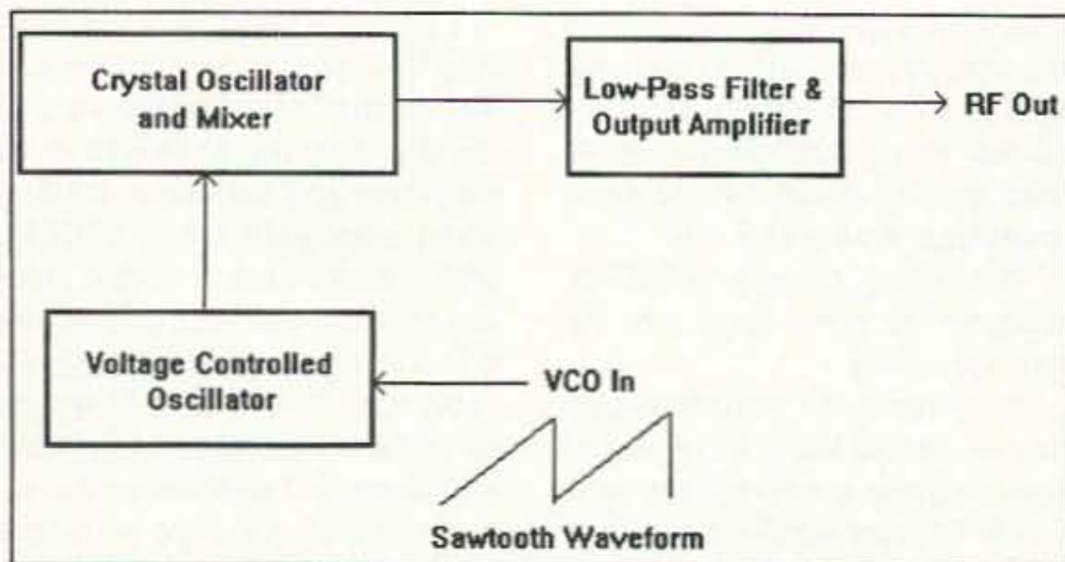
Fig. 2. A more detailed block diagram.
