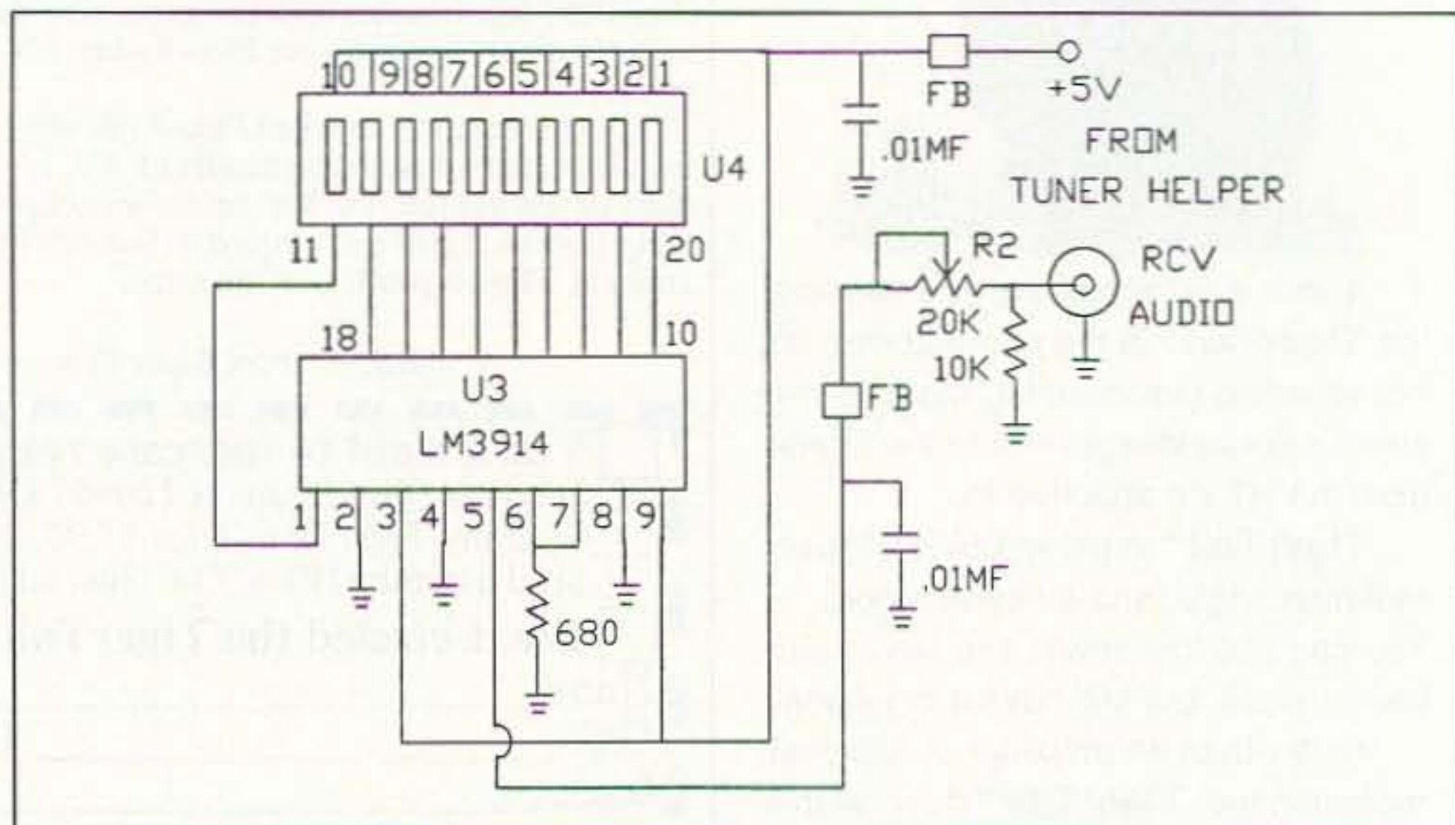
Figure 3. Bar graph schematic.
