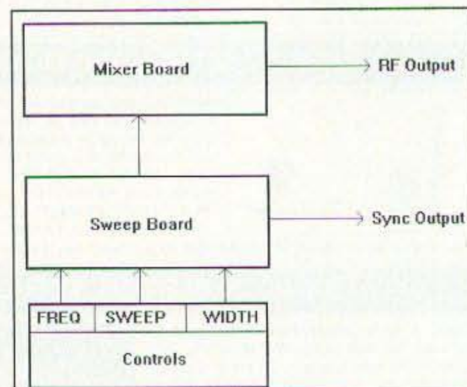
Fig. 1. Internal block diagram of the RSG-2.
