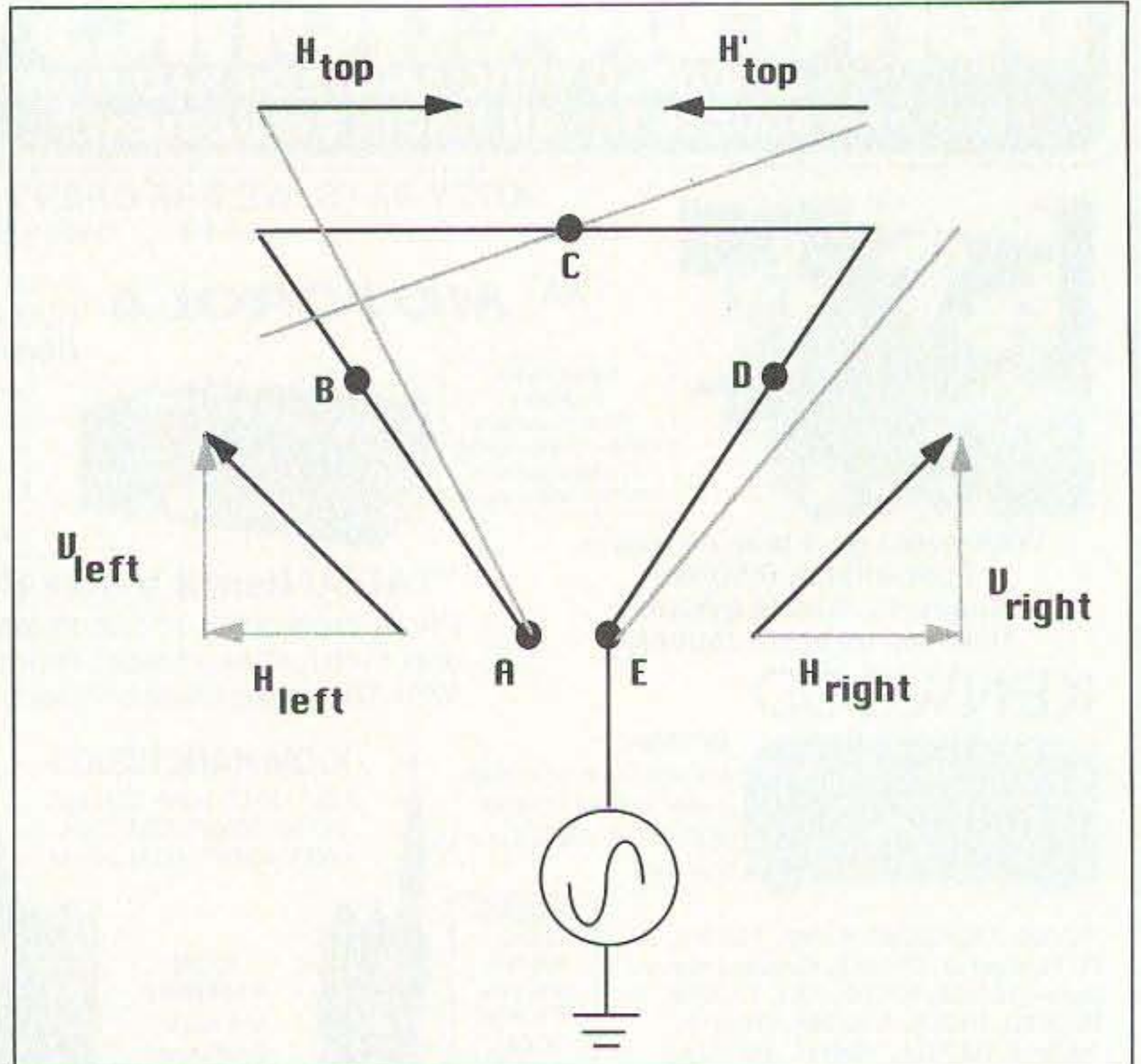
Figure 5. Current distribution of an end-fed full-wavelength loop.
