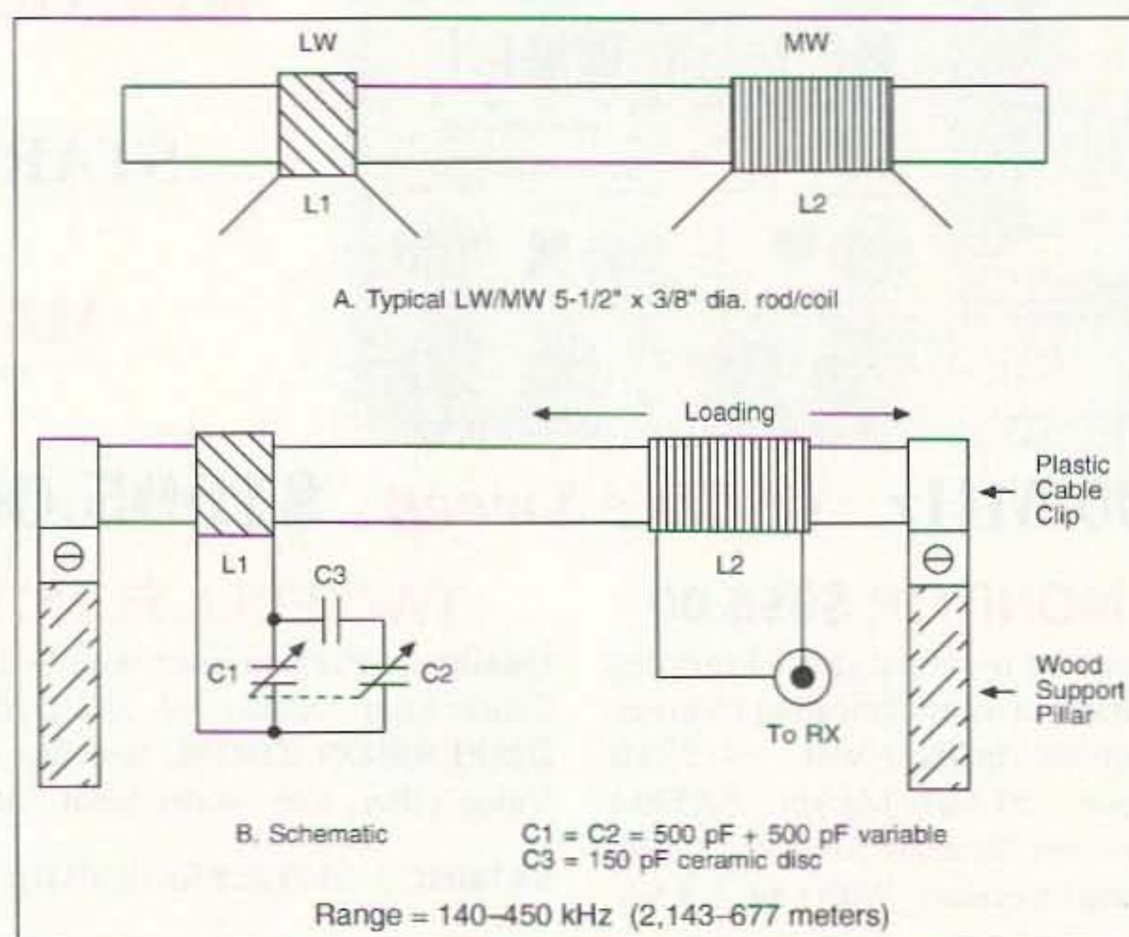
Figure 1. Typical LW/MW 5 1/2" x 3/8 dia. rod/coil.
