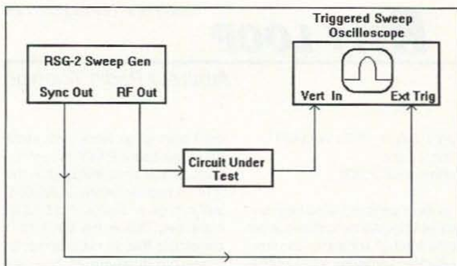
Fig. 3. External connection configuration for the RSG-2.
