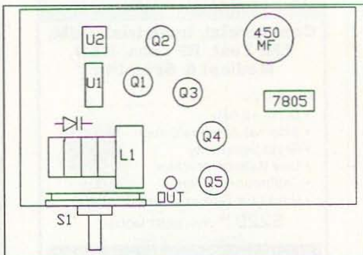
Figure 4. Suggested layout.
