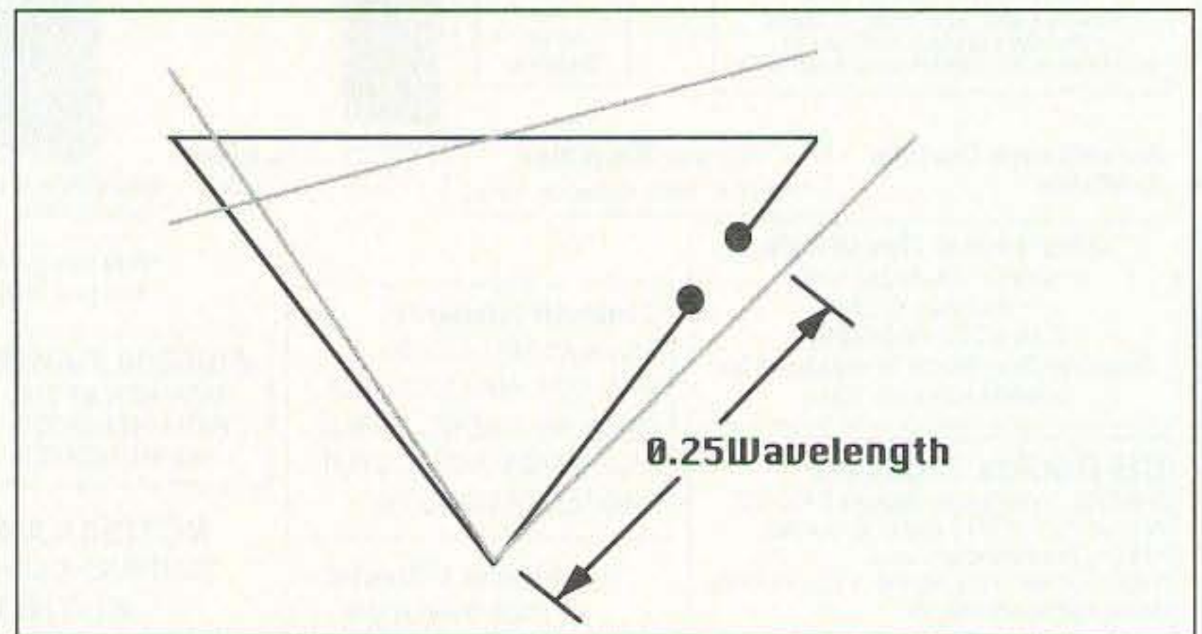
Figure 6. Current distribution of an inverted delta loop, side-fed.
