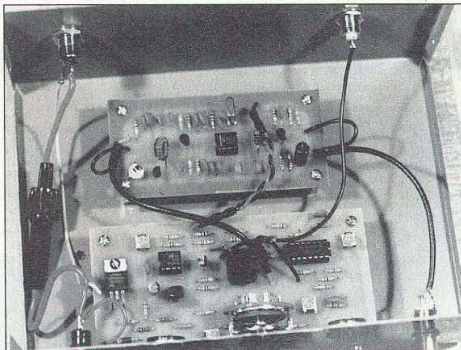
Photo B. Internal view of the RSG-2.
