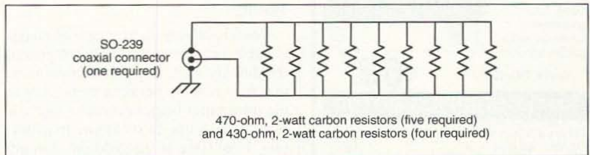
Figure 2. Schematic for the 50-ohm "add-on" load.
