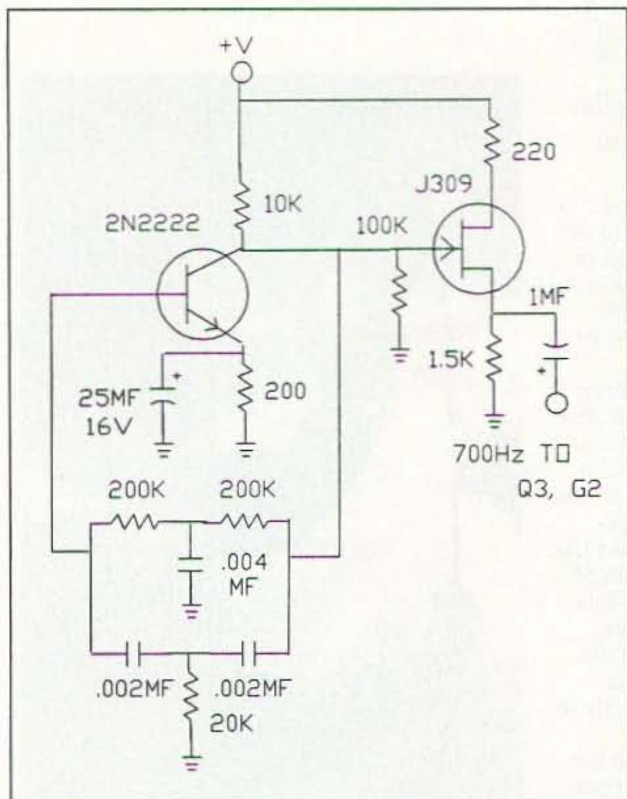
Figure 2. Tone oscillator.
