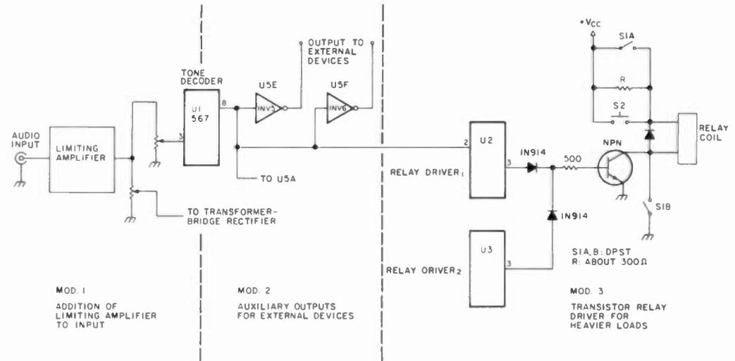
Fig. 8. Some modifications to CRASH.
