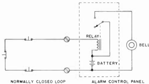
Fig. 1. Schematic of a simple closed-loop alarm using a relay, battery, and bell. The closed loop is self-testing because the loop must be made up before the alarm is turned on.
