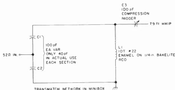
Fig. 1. Transmatch network in the minibox.
