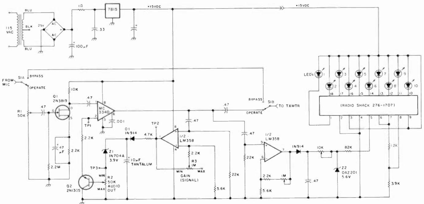
Fig. 1. Speech expander/clipper with LED bar-dot display.
