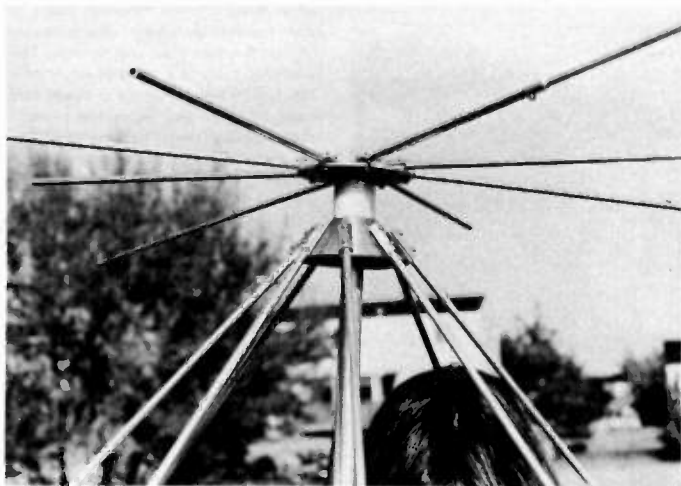
Photo C. The two discs of the disccone, top (radiator) and bottom (ground-plane reflector).
