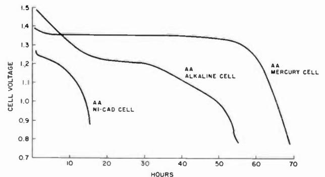
Fig. 1. Cell discharge curves. 25 Ohms continuous discharge.
