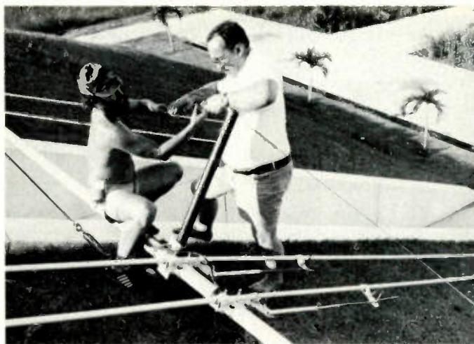
Jean H51ANV/ON8JA (left) and Hans H51BG secure the supporting truss on the 20/15-meter (full-size) beam. Note the gamma match, using aluminum piping, plastic hose, and an inner core of copper tubing for the driven elements.
