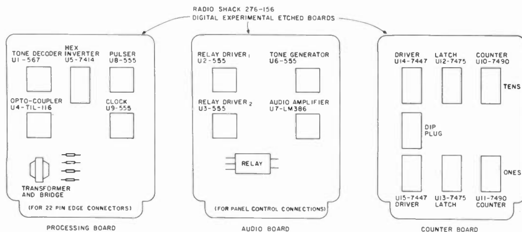
Fig. 7. Suggested board layouts for CRASH.
