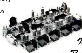
TTC 100 Touch Tone Control Board
