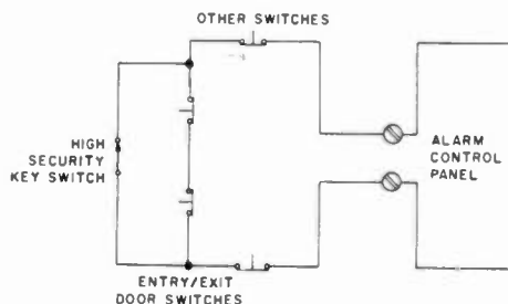
Fig. 4. Example of how a high-security keyswitch is used to bypass entry/exit doors. This type of circuit is used on commercial intrusion alarms.
