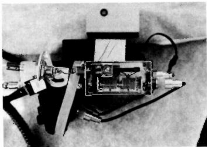
The modification of the antenna-mounting bracket.
