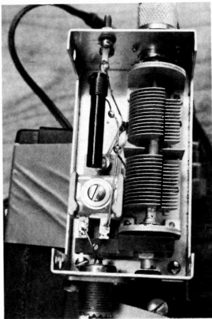
The transmatch innards in the minibox.
