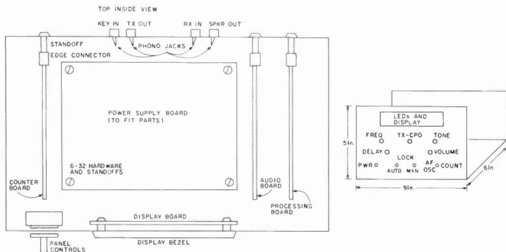
Fig. 6. General layout sketch for CRASH.
