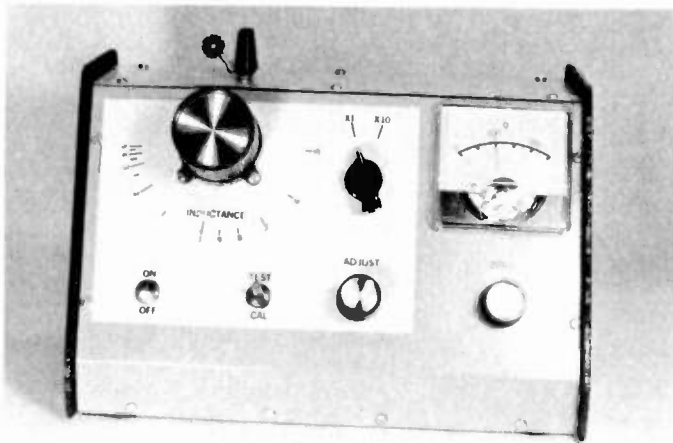
Front view of completed Q-meter.
