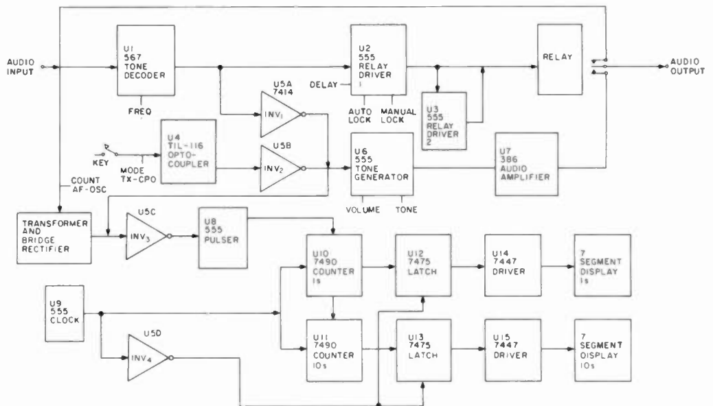
Fig. 1. Block diagram of CRASH.
