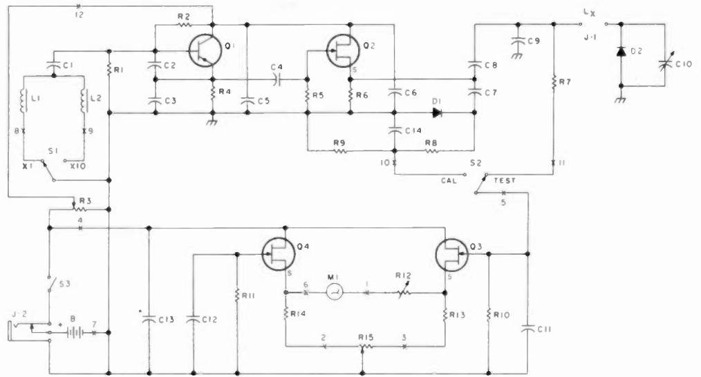
Fig. 1. Circuit schematic.
