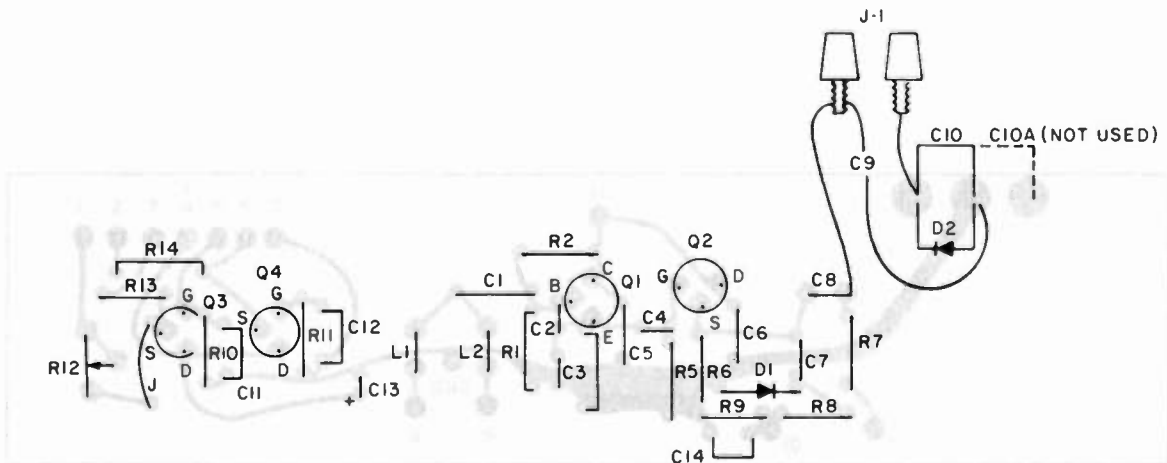
Fig. 3. Component layout, foil side view.
