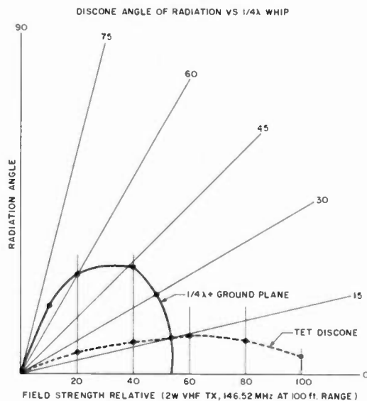
Fig. 1. Angle of radiation relative to a quarter-wave vertical.
