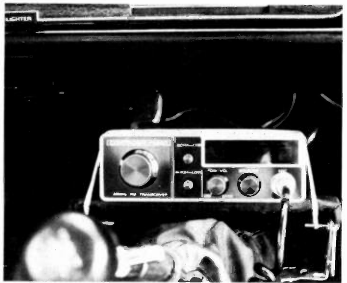
Fig. 5. This rig-mounting bracket is ideally suited to rapid installation artists. The unit is merely placed on the mount and secured with a heavy rubber band. Either top or bottom-mounted speakers can be used with this arrangement.
