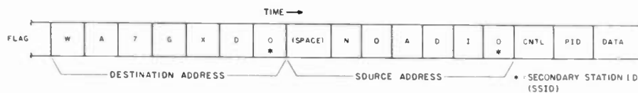
Fig. 2. Typical AX.25 non-digipeated address header.
