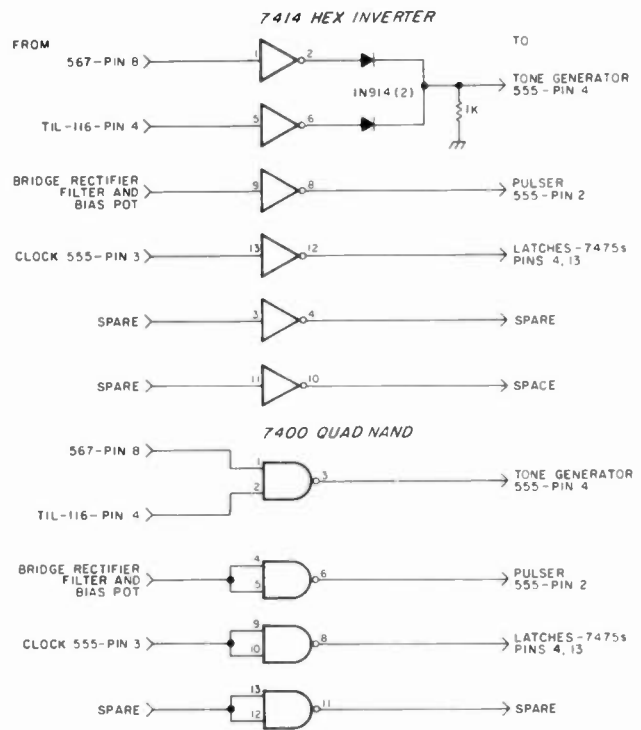
Fig. 4. Using a 7400 in place of the 7414.
