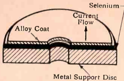
Fig. 1—All commercial metallic rectifiers contain three essential elements—a good conductor, a poor or semi-conductor, and a barrier layer between the two. In the selenium rectifier a thin layer consisting of a compound of selenium itself acts as the semi-conductor. →
