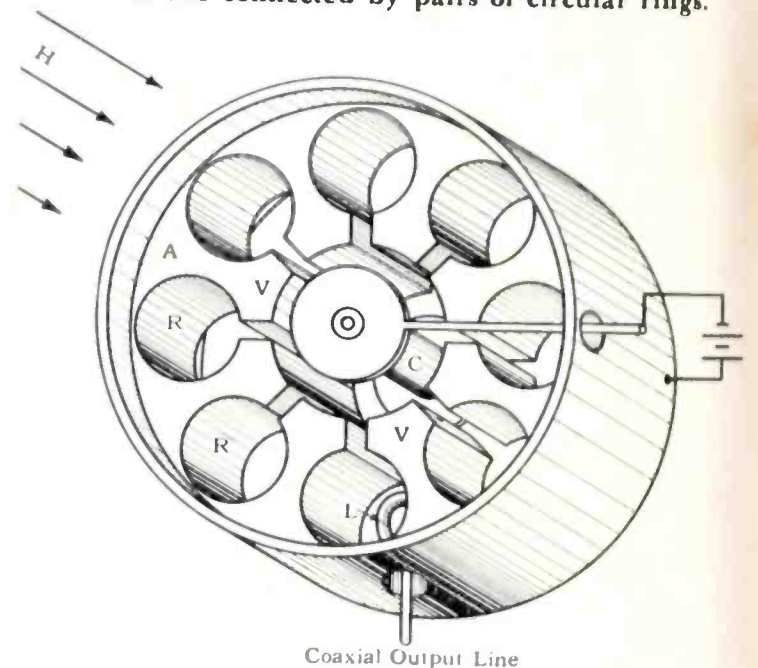
Fig. 2—The magnetron can be considered as employing the action of resonant circuits.
