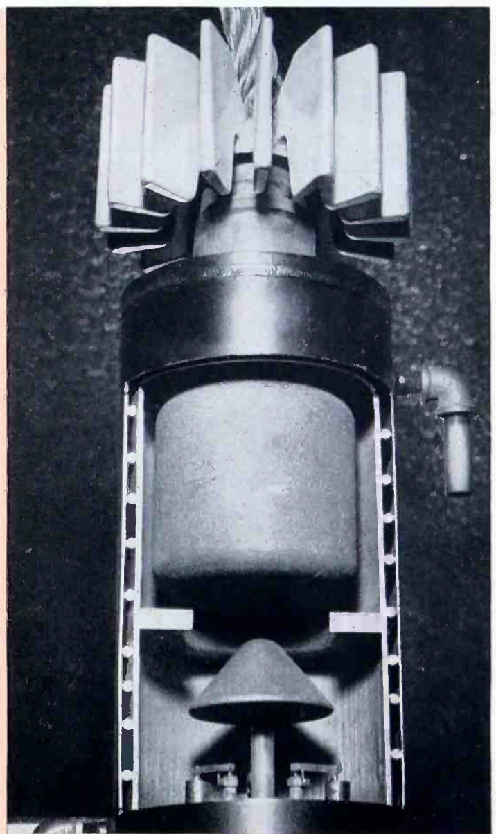
Figs. 1 and 2—The sealed ignitron for resistance-welding service (left above) is somewhat simpler than a rectifier tube (right above). The rectifier, shown in cutaway at the right, has two ignitors and has additional arc shielding.
