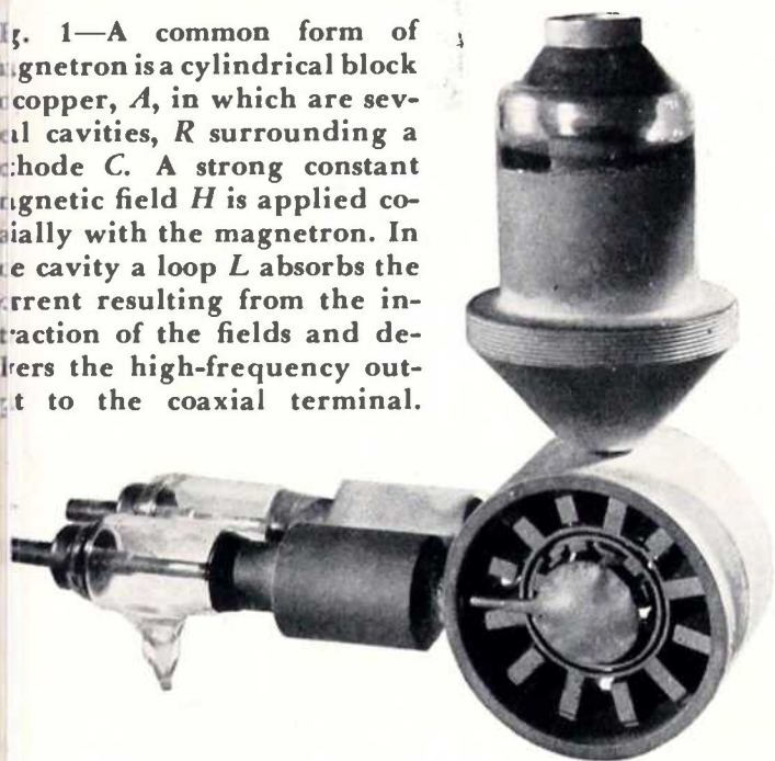
In this 10-cm magnetron the cavities, instead of being holes milled out of a solid block of copper, are formed by brazing vanes into a cylindrical shell. The tube delivers approximately 700-kw peak or pulse power.
