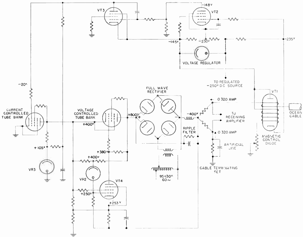
Figure 3. Complete theory of power source
