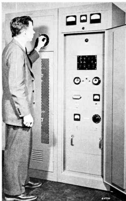
Power supply unit and cable terminating equipment—Manual adjustment of primary voltage. This is necessary only on initiation of service
