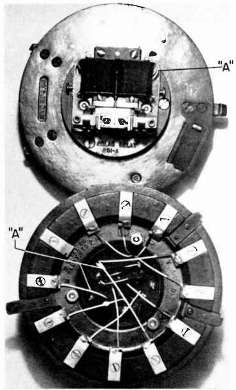
Figure 6. Polar Relay 201-A, top and bottom views "A" shows 28 A.w.g. vinyl insulated and nylon jacketed wire leads
