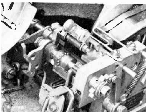
Figure 4. Printer-Perforator 39-A modified to produce folds
