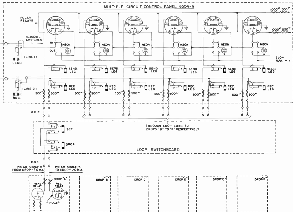
Figure 14. Theory of Multiple Control Panel 6504-A
