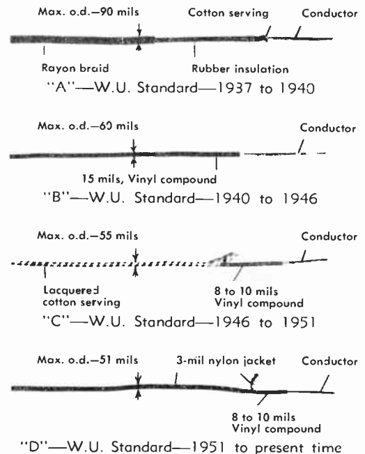
Figure 1. No. 22 A.w.g. instrument wire—successive standards established during the past 12 years
