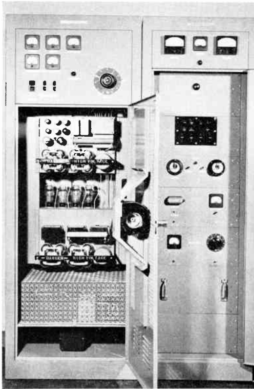
Power supply unit and cable terminating equipment. Left-hand cabinet shows rectifier tubes near middle with absorption banks above and below. Right-hand cabinet contains line terminating equipment and control amplifier
