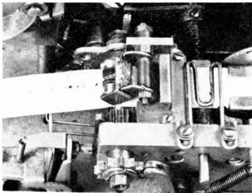
Figure 5. Left—unstiffened perforator tape in accumulator; Right—same accumulator holding almost twice as much stiffened tape
