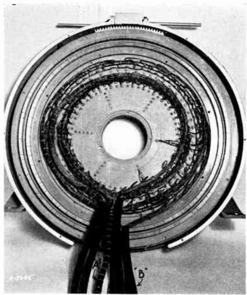
Figure 3. 6-channel face plate, for Multiplex Distributor 226-A, illustrating the intricate wiring, forming and terminating in this unit, requiring some 1,500 ft. of 22-A.w.g. flexible vinyl insulated and nylon jacketed instrument wire. "A" shows one of the hand-made forms before applying the vinyl tubing indicated at "B"
