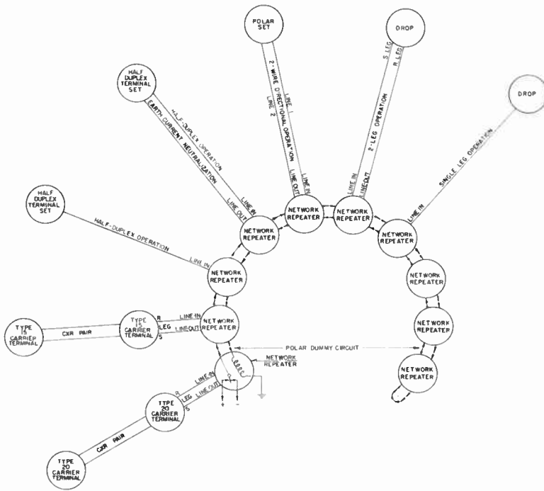
Figure 6. Theory of Application of Half-Duplex Network Repeater 4617
