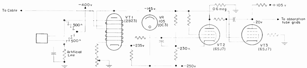
Figure 1. Cable terminating set and current control amplifier
