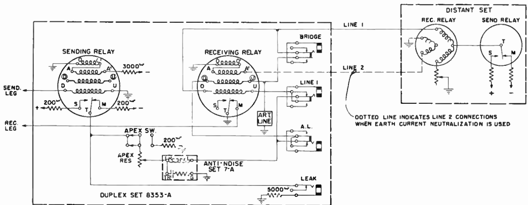
Figure 11. Theory of Duplex Set 8353
