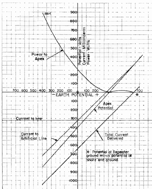
Figure 2. Potential current and power as affected by earth potential
