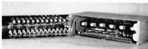
Figure 13. Multiple Control Panel 6504-A showing, at bottom, inside assembly and wiring
