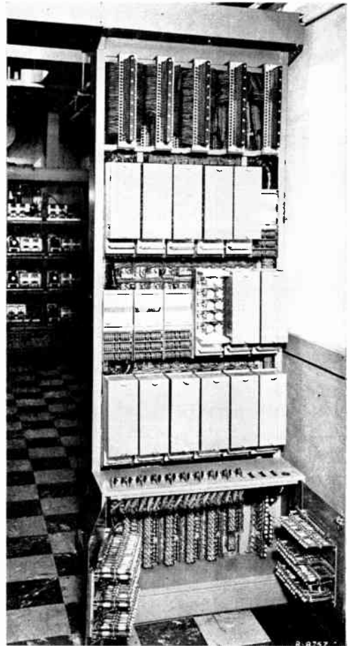
Figure 5. CND multi-send rack—rear view
