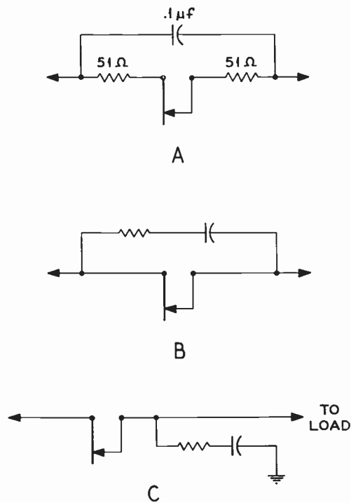
Figure 4. Spark killers
