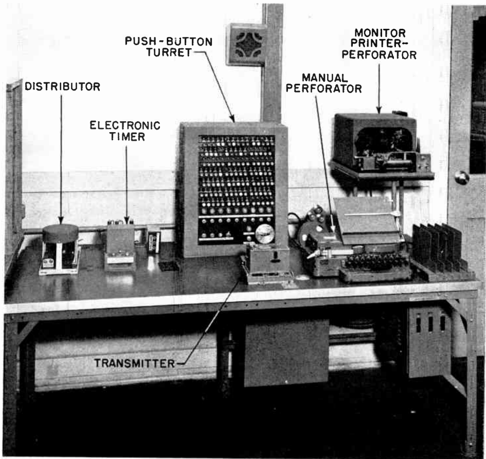
Figure 2. CND multi-send table
