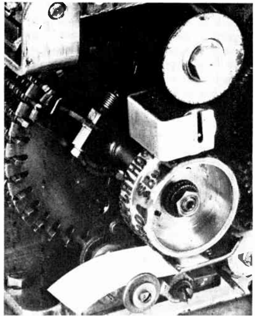
Ink roller and rubber faced typewheel of a quotation ticker. For projection, printing is on cellophane
