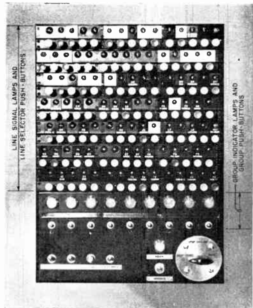
Figure 3. CND multi-send turret
