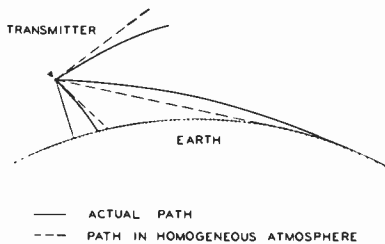
Figure 3. Geometric ray curvature
