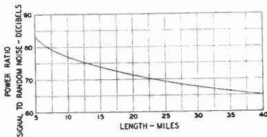
Figure 2. Radio path signal-to-noise ratio
