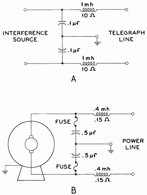
Figure 6. Line interference eliminators
