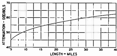
Figure 1. Path attenuation at 4000 megacycles
