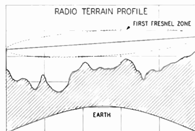
Figure 4. Radio terrain profile
