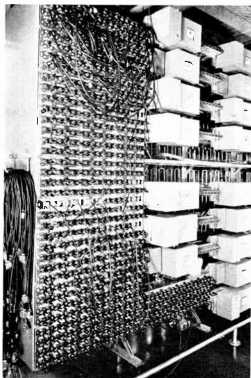
Figure 70. Receiving leg patching board
