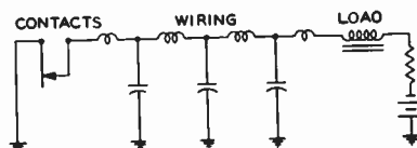
Figure 3. Typical contact circuit
