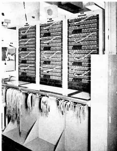
Figure 68. Traffic routing board
