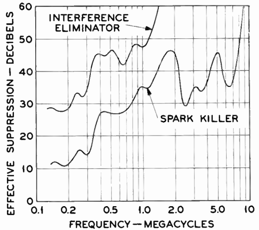
Figure 7. Interference eliminator performance
