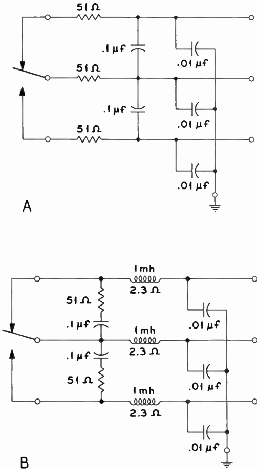
Figure 5. Contact-protecting interference eliminators
