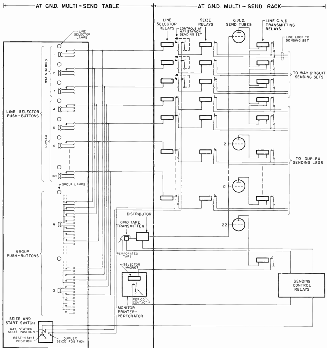
Figure 1. CND multi-send arrangement
