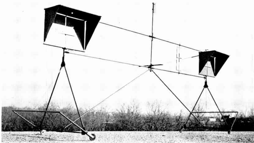
Figure 3. Target for boresighting fighter planes.
