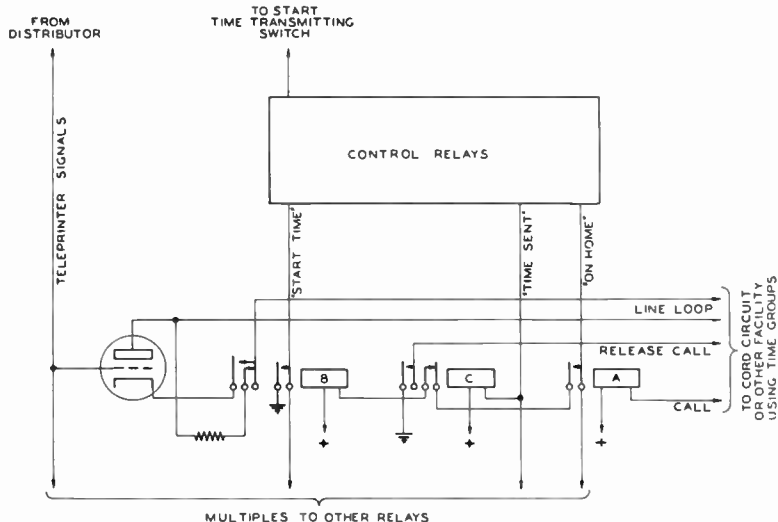
Figure 3. Circuit for sending time and date
