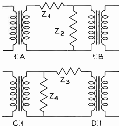
Figure 11. Equivalent L networks using ideal transformers
