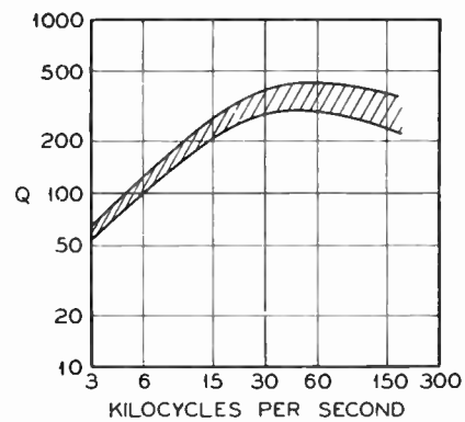
Figure 9. Coil reactance—resistance ratios realized in WN filters
