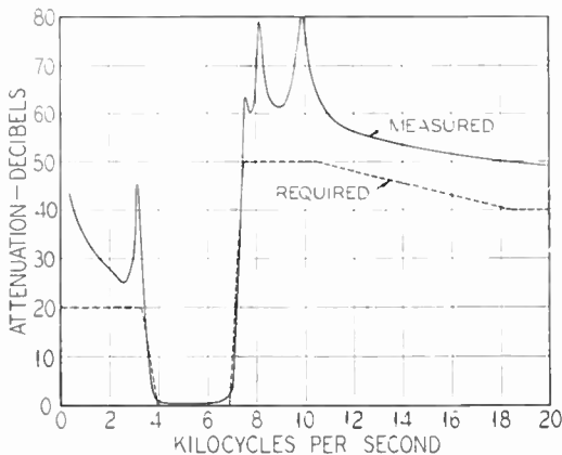
Figure 3. Required (dotted) and measured (solid) attenuation
