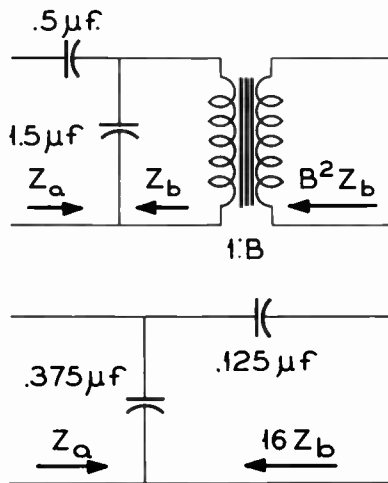
Figure 12. Example of ideal transformer use
