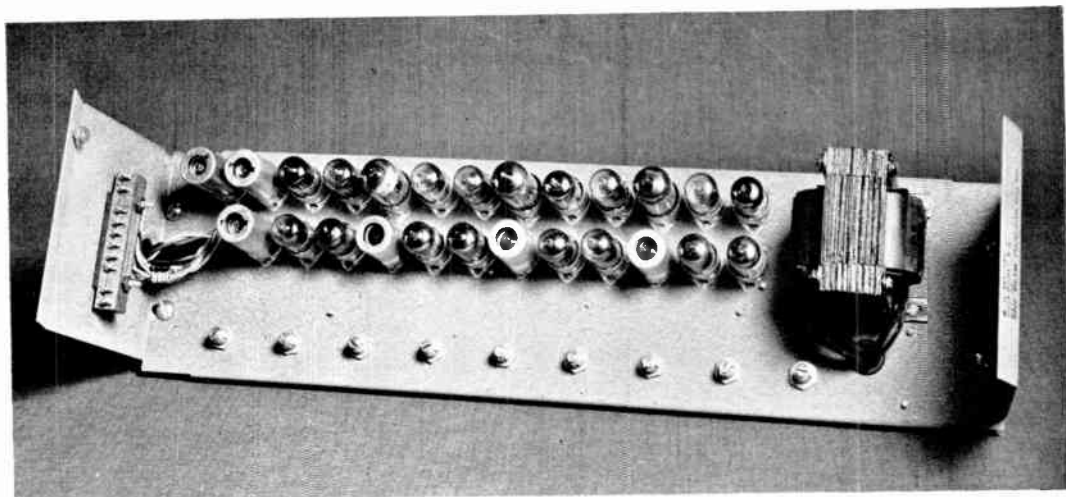
Western Union pulse modulation equipment is compact
