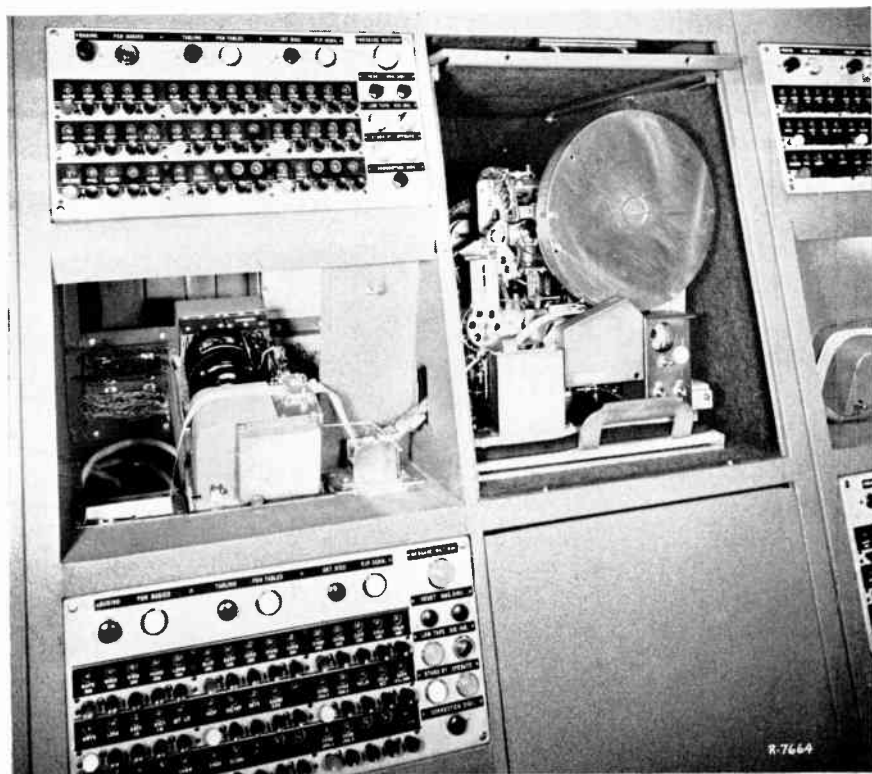
Figure 6. Operating position of Plan 51 unit
