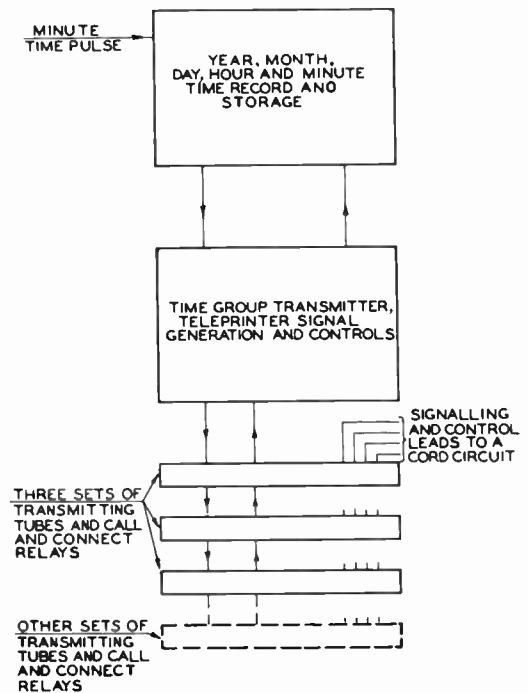
Figure 1. General arrangement of time and date transmitter
