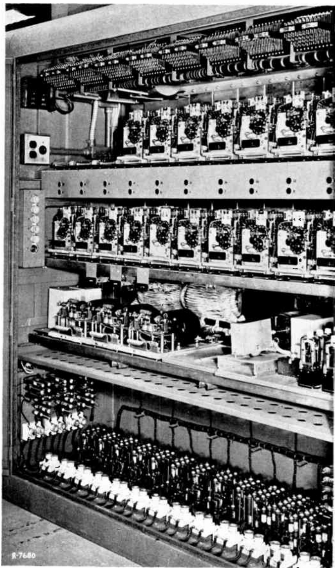
Figure 14. Central control cabinet
