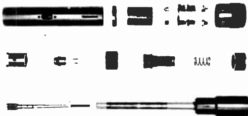
Figure 2. Exploded view of boresighter
