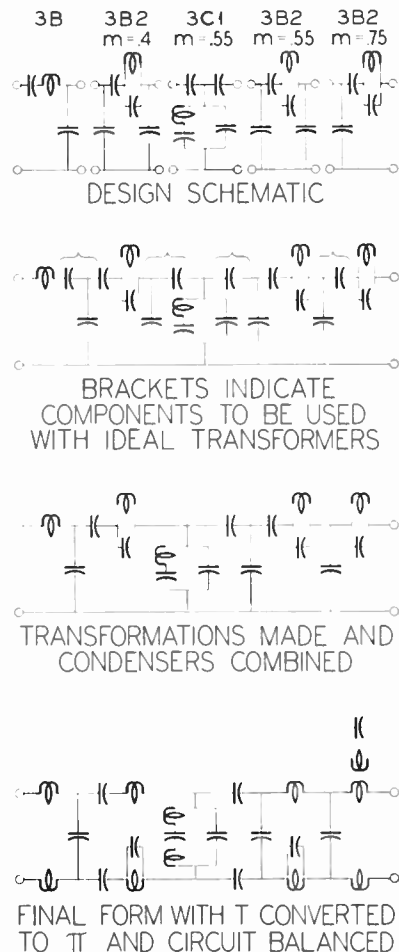
Figure 2. Successive stages in design of typical filter
