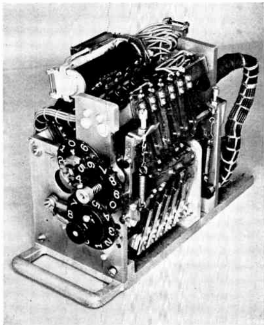
Figure 15. Three-digit automatic numbering machine
