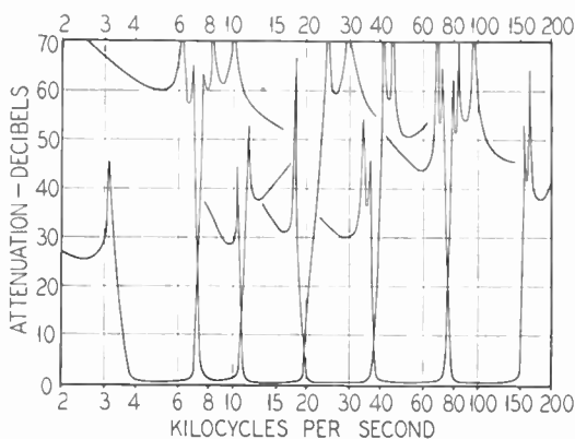
Figure 5. Measured attenuation of six WN System filters
