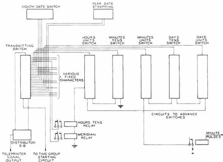
Figure 2. Circuit for setting up time and date
