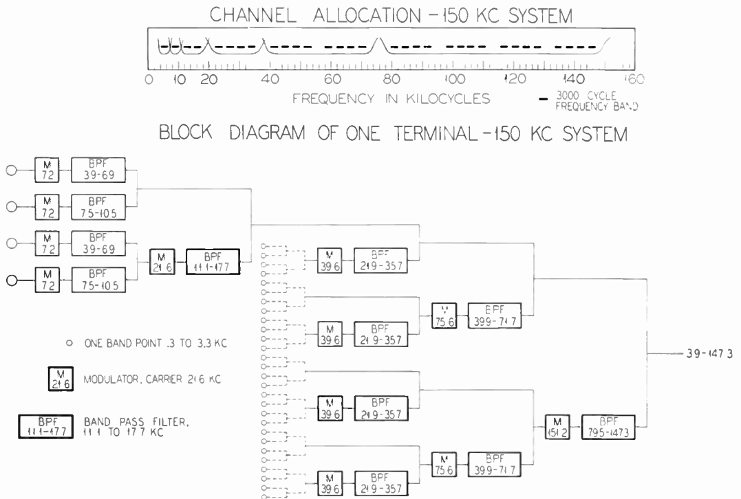
Figure 1. WN system block diagram
