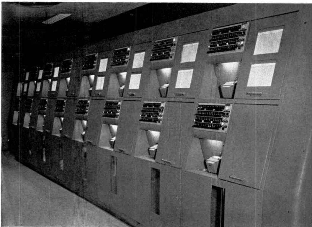
Figure 5. Assembly of operating cabinets of Plan 51 unit
