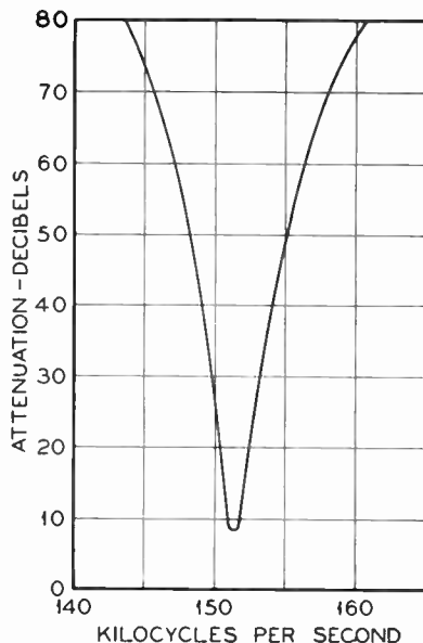
Figure 6. Measured attenuation of 151.2-kc filter
