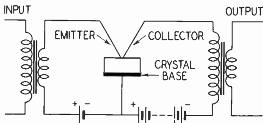
Figure 2. Transistor amplifier circuit
