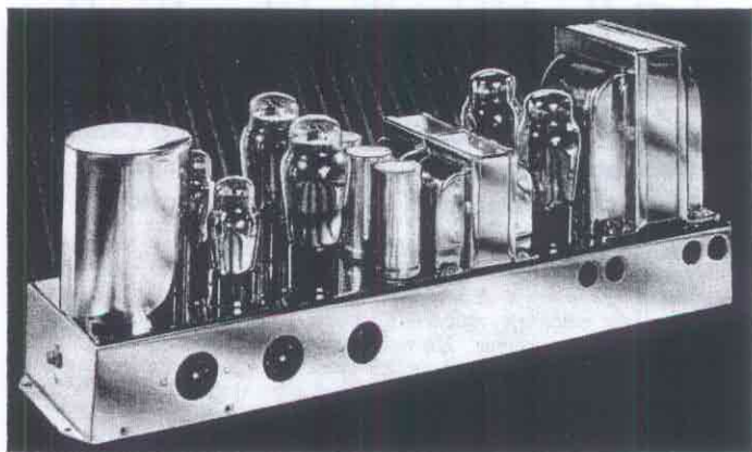
View Showing Separate Power Amplifier Used in the Scott FM-AM Phantom.
