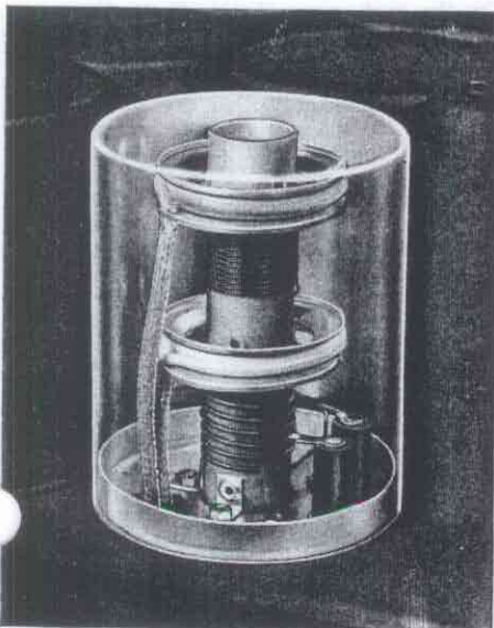
Sectional View of the Scott Supershield Antenna Coupling Unit.
