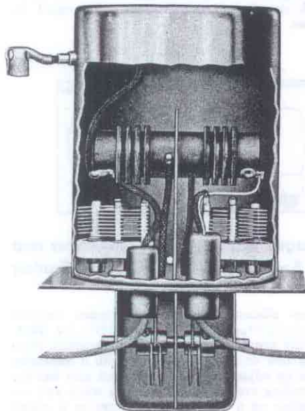
Sectional view of one of the four stage IF transformers used in the Scott FM-AM Philharmonic, showing the four Pi Litzendrath coils, air tuning condensers, and part of the Selectivity Control.
