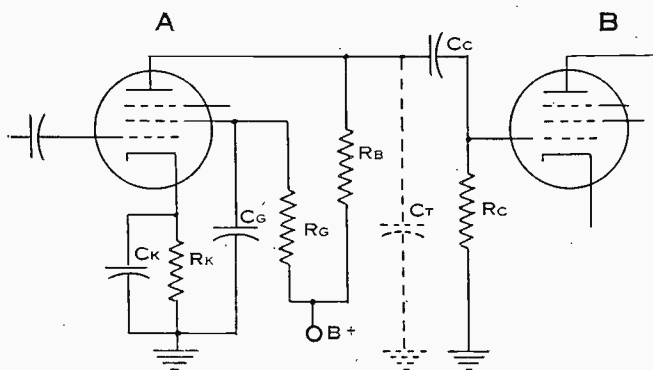
FIGURE 1 TYPICAL UNCOMPENSATED AMPLIFIER
