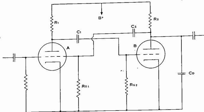
TYPICAL MULTIVIBRATOR CIRCUIT
