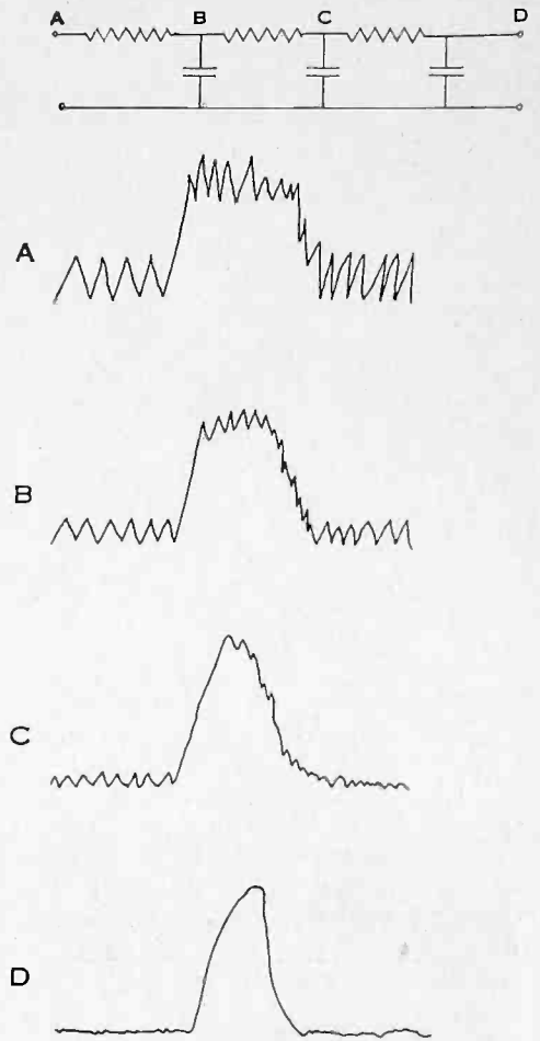
WAVE FORMS OF A TYPICAL INTEGRATOR
