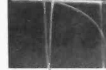
Figure 10—Waveforms obtained at various points in horizontal sweep circuit.
