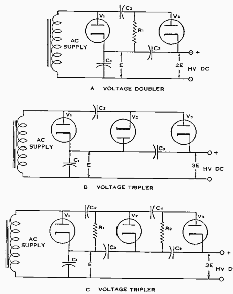
FIGURE 2 VOLTAGE MULTIPLIER CIRCUITS
