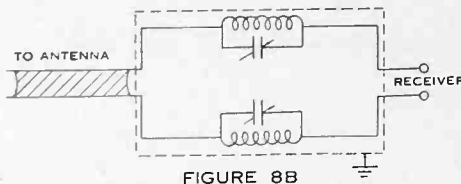
FIGURE 8B PARALLEL-TUNED WAVE TRAP IN ANTENNA TUNE TO FUNDAMENTAL OF INTERFERING STATION
