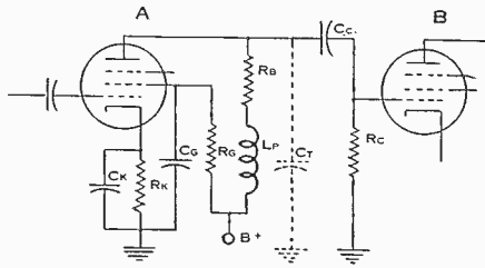
FIGURE 3 AMPLIFIER WITH HIGH FREQUENCY SHUNT COMPENSATION
