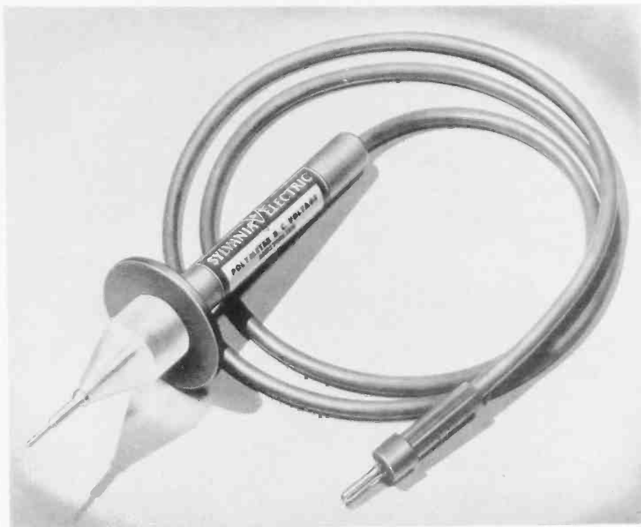
Compact dc voltage multiplier consists of a 48" plug-in flexible lead tested for 22,000 volt breakdown; nickel-plated brass contact pin mounted in tapered polystyrene rod 13/4" long, a removable bakelite safety flange 2" in diameter; and varnished bakelite handle, 4 1/4" long, enclosing dropping resistor tested at 30,000 volts.
