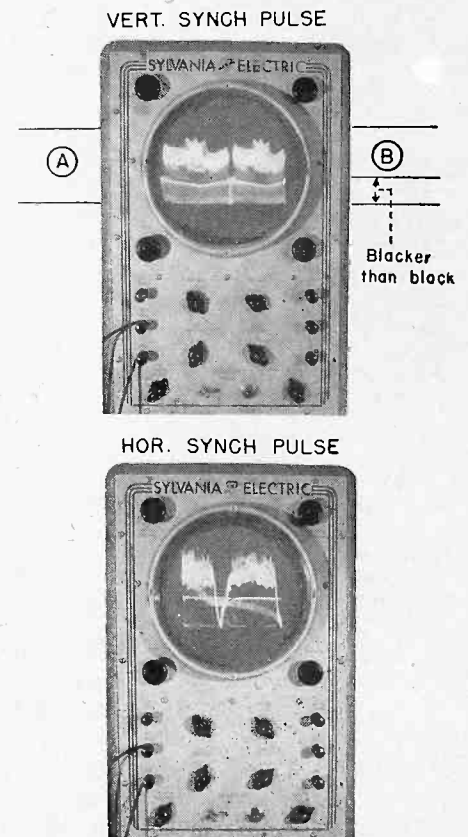
Figure 1 Waveforms horizontal and vertical obtained at detector output.
