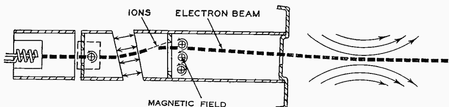
FIGURE 3—BEAM PATH WITH MAGNET TOO FAR FORWARD
