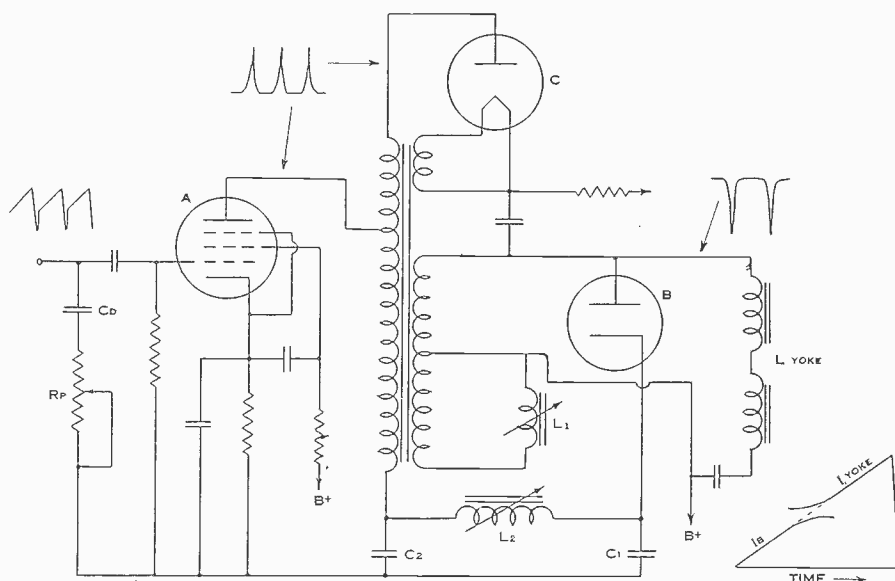
HORIZONTAL AMPLIFIER CIRCUIT FOR MAGNETIC DEFLECTION
