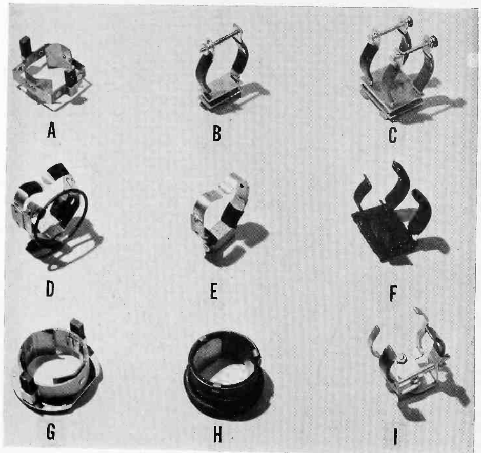
FIGURE 1—TYPES OF ION TRAP MAGNETS
