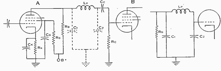
FIGURE 5 A SERIES PEAKING HIGH FREQUENCY COMPENSATION
