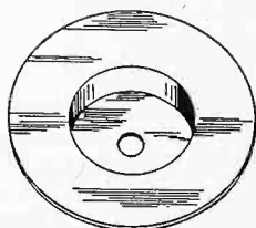
NORMAL ANODE TOP DISC ION TRAP MAGNET CORRECTLY ALIGNED
