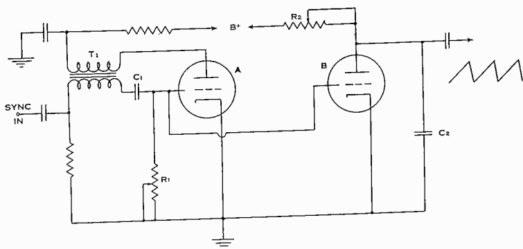
TYPICAL BLOCKING OSCILLATOR AND SAWTOOTH GENERATOR FIGURE 2
