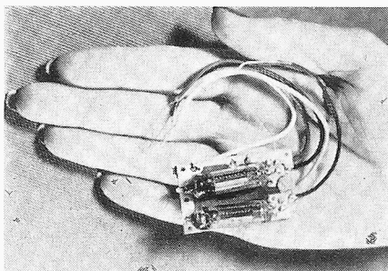
Receiver audio section of new transceiver developed by the Citizens Radio Corporation of Cleveland, Ohio embodies new silver-on-ceramic circuit techniques. This audio section (shown above) uses two Type 1V5 Sylvania subminiature tubes.
