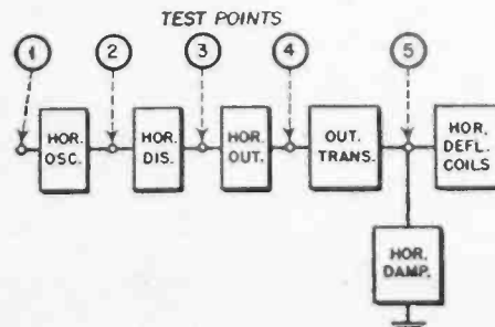
BLOCK DIAGRAM OF PARTIAL HORIZ. SYNCH. DEFLECTING CIRCUIT
