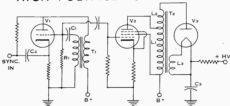
FIGURE 4 TYPICAL PULSE TYPE HIGH VOLTAGE SUPPLY
