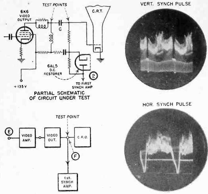
Figure 3 Horizontal and vertical pulses obtained at video output tube.
