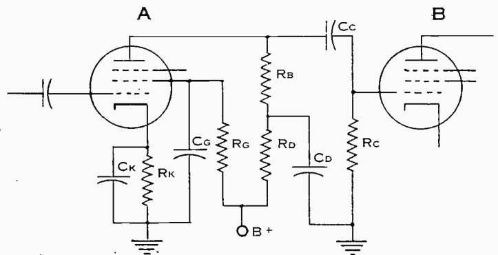
FIGURE 2 AMPLIFIER WITH LOW FREQUENCY COMPENSATION
