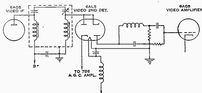
FIGURE 2 ANOTHER VIDEO DETECTOR
