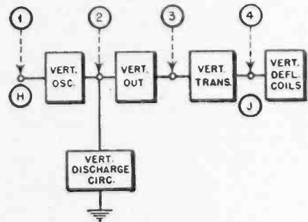
PARTIAL BLOCK DIAGRAM
