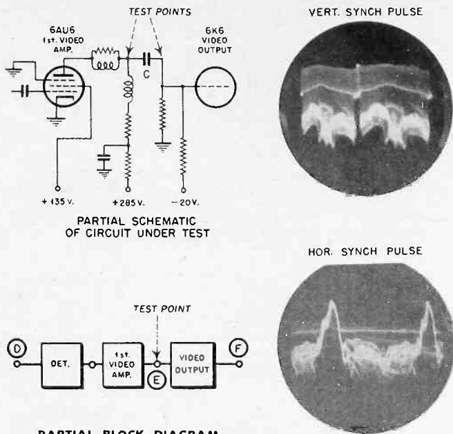
Figure 2 Horizontal and vertical pulses obtained at 1st video amplifier.
