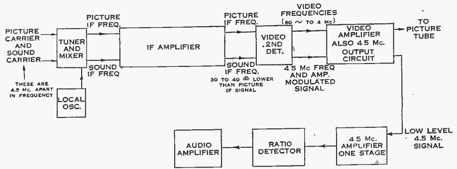
FIGURE 1 BLOCK DIAGRAM OF INTERCARRIER SYSTEM
