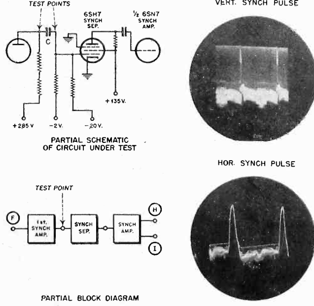
Figure 5 Pulses obtained at input of 6SH7 sync separator. Note waveforms.
