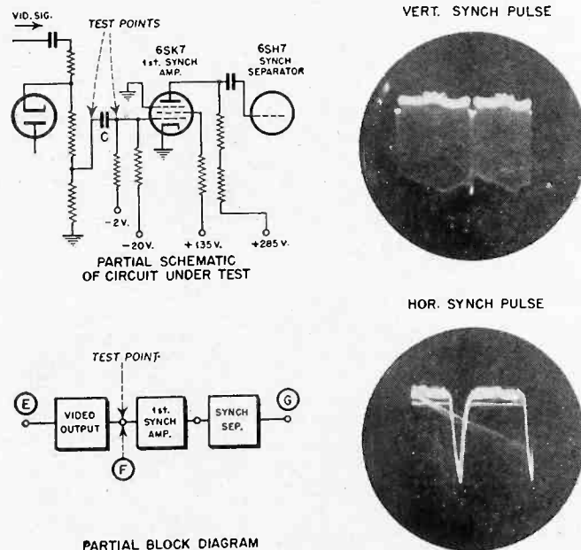
Figure 4 Pulses obtained at 1st sync amplifier on either side of C.
