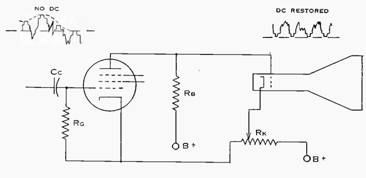
FIGURE 9 TYPICAL GRID LEAK DC RESTORER CIRCUIT
