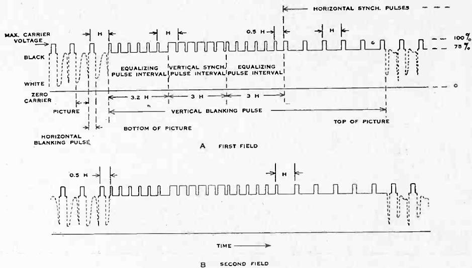
STANDARD TELEVISION SYNCHRONIZING WAVE SHAPE FIGURE 1
