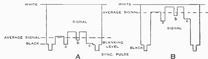
FIGURE 7 IDENTICAL SIGNALS WITH DIFFERENT BRIGHTNESS LEVELS.
