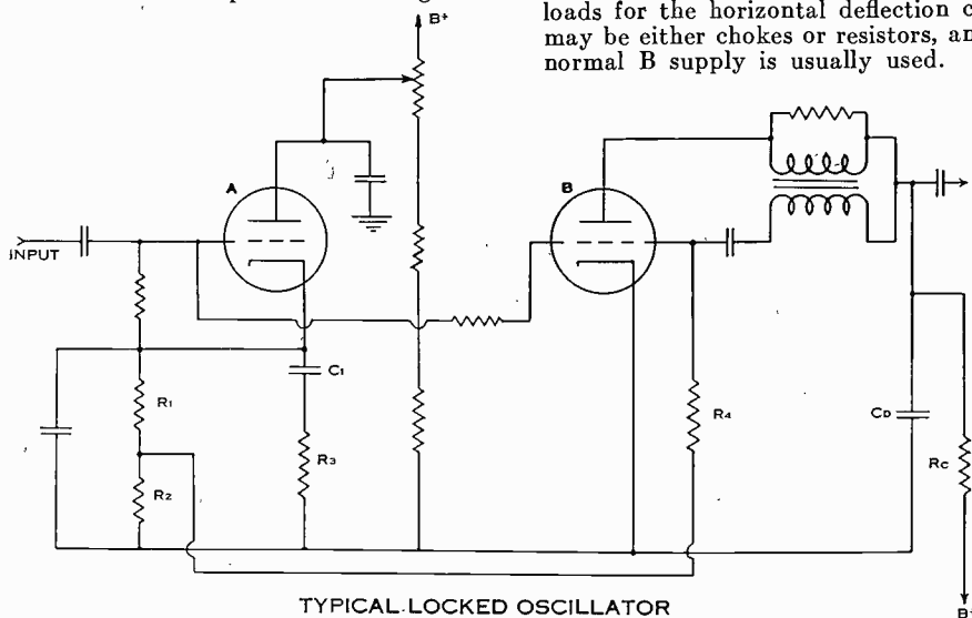
TYPICAL LOCKED OSCILLATOR FIGURE 4
