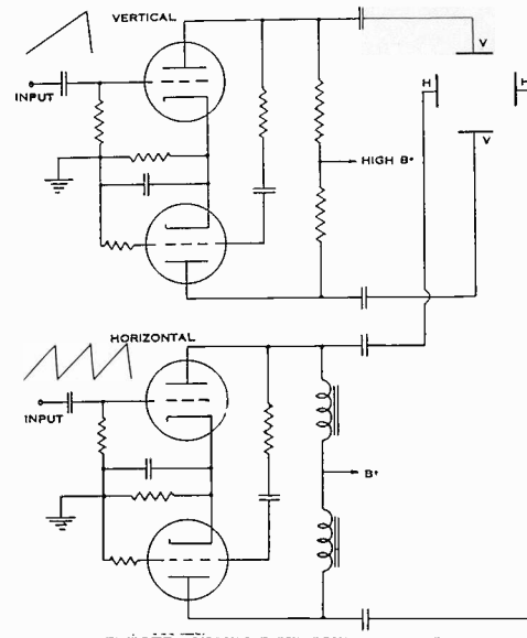
ELECTROSTATIC DEFLECTION SYSTEM FIGURE 5
