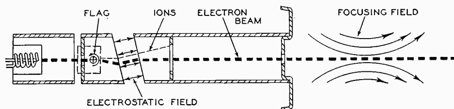
FIGURE 2—BEAM PATH WITH MAGNET CORRECTLY ALIGNED
