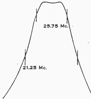
FIGURE 3 TYPICAL SYMMETRICAL IF RESPONSE CURVE
