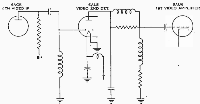
FIGURE 1 DIODE VIDEO DETECTOR OF A TYPICAL RECEIVER
