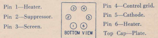
Bottom View of Socket Connections.
