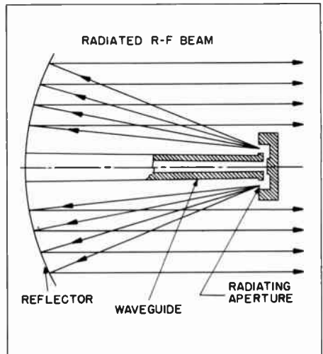
Figure 19. Cutler Feed
