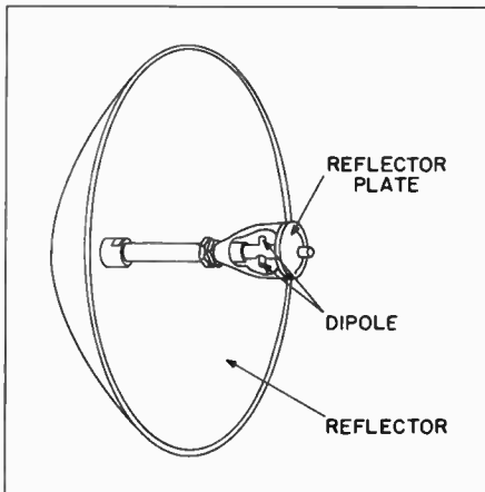
Figure 3. SCR-584 Antenna
