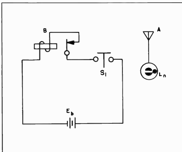
Schematic Diagram of Line Checker for Airborne IFF Transponders
