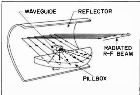
Figure 20. Pillbox Feed to a Cylindrical Reflector
