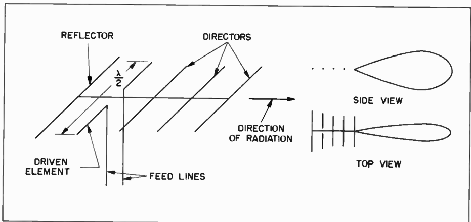
Figure 25. Yagi Antenna and Radiation Pattern
