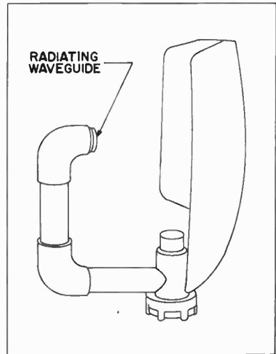
Figure 5. SL Radar Antenna
