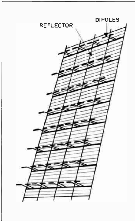
Figure 2. SCR-270 Bedspring Antenna
