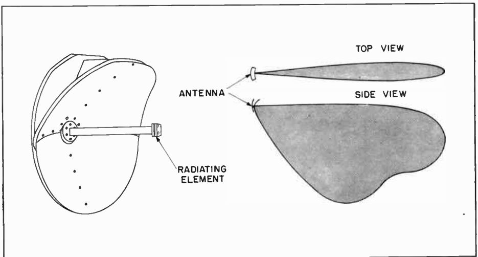
Figure 10. Cosecant-Squared Antenna and its Radiation Pattern
