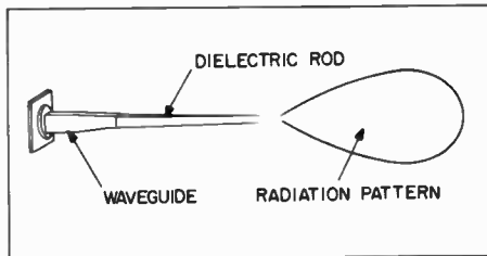
Figure 22. Dielectric-Rod Antenna
