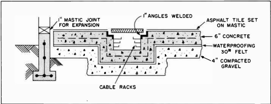
Figure 2. Cross-Sectional View of Typical Concrete Floor
