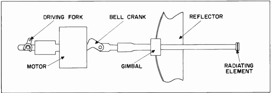
Figure 17. Nutating-Scan Feed for SCR-584
