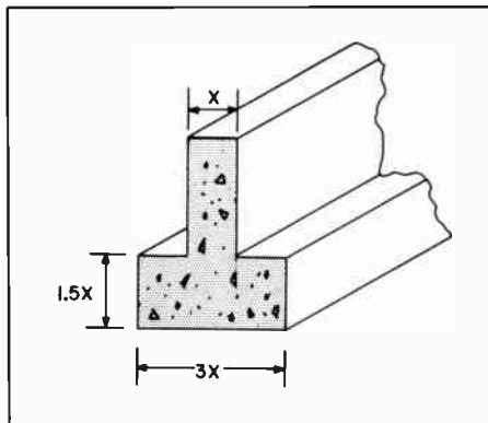
Figure 1. Aspect Ratio of Concrete Foundation
