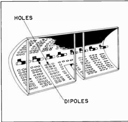
Figure 9. Parabolic-Cylinder Antenna
