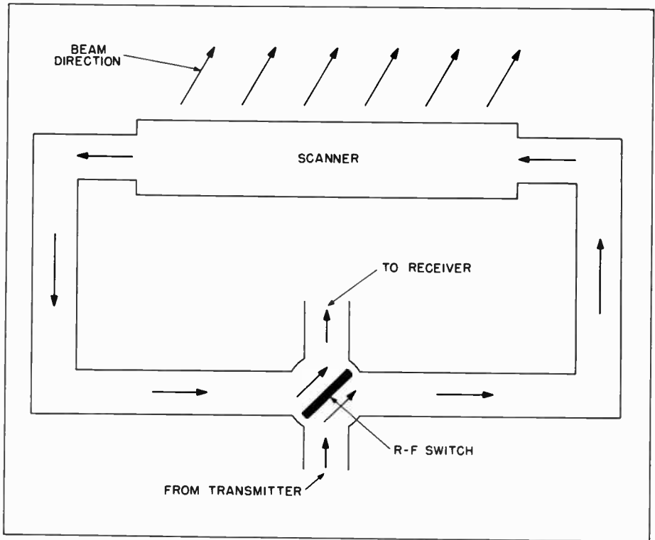
Figure 28. Energy Flow in Waveguide of Eagle Scanner
