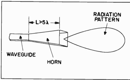
Figure 24. Horn Antenna
