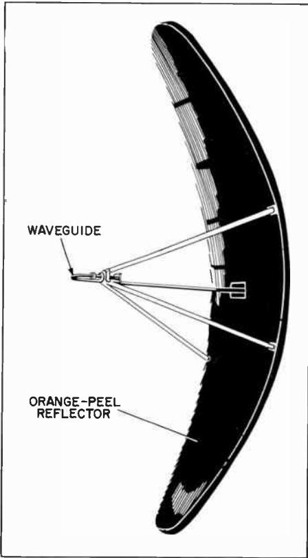
Figure 7. AN/TPS-10 Antenna
