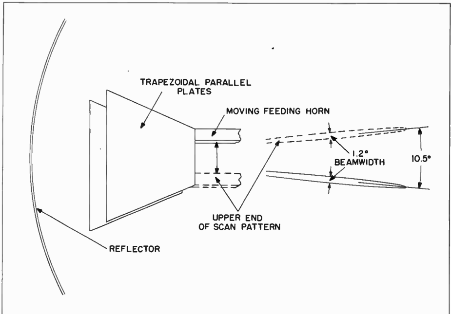
Figure 21. Robinson Electrical Feed for SCI Height-Finder Antenna
