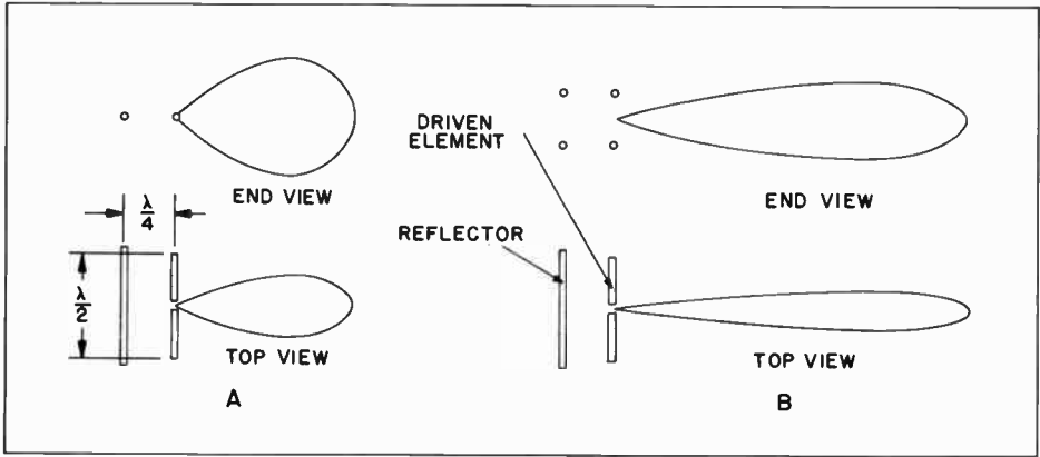
Figure 11. Radiation Pattern of Dipoles and Reflectors
