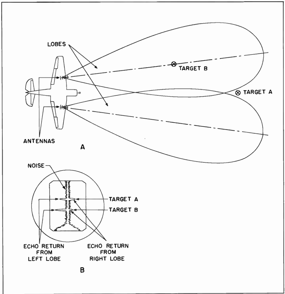
Figure 26. Yagi Antennas Used for Lobing
