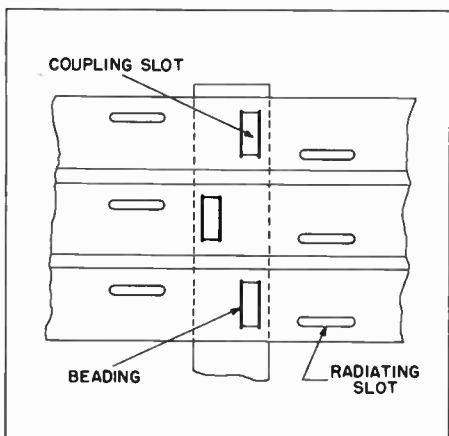
Figure 32. Feeder for Short-Range Array of MK-6 Antenna
