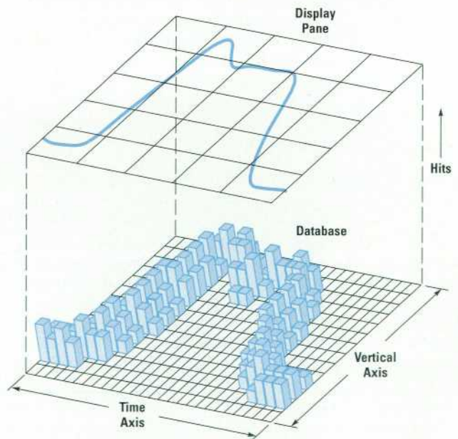
Fig. 2. Waveforms are mapped onto a database for statistical analysis. The database consists of 115,456 pixels arranged in 451 columns by 256 rows. Each pixel can record up to 65,535 waveform hits.
