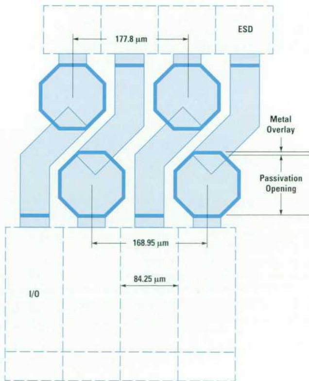
Fig. 2. Sample bond pad connection.
