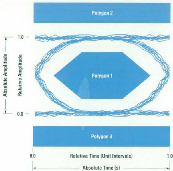
Fig. 8. Concept of mask testing.
