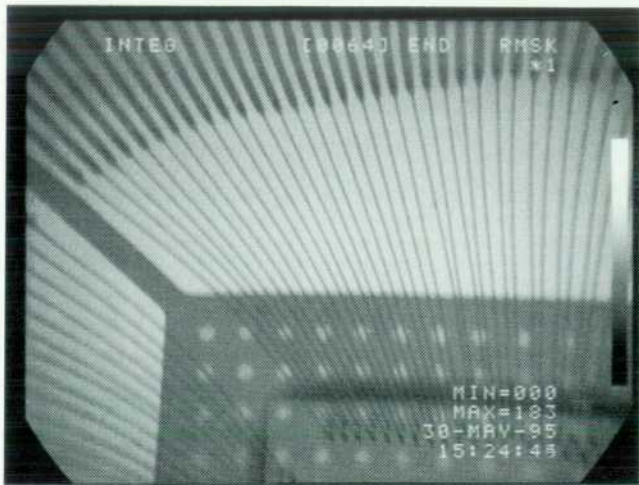
Fig. 2. X-ray micrograph of a molded package showing wire sweep. The curvature in the wire trajectories is induced by resin flow during soldering.
