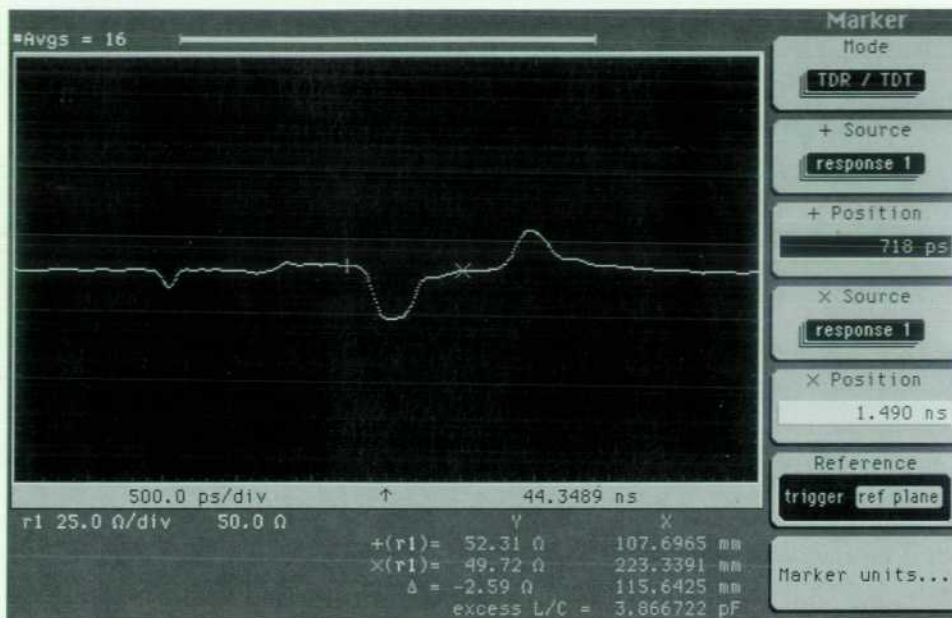
Fig. 4. The waveform is integrated between the + and x markers to yield an excess capacitance of 3.86 pF. Negative-going variations are capacitive and positive-going variations are inductive.
