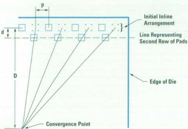
Fig. 6. Graphical method for radial staggering.
