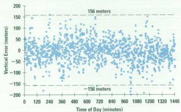
Fig. 3. GPS vertical errors over a 24-hour period using SPS (from reference 1).
