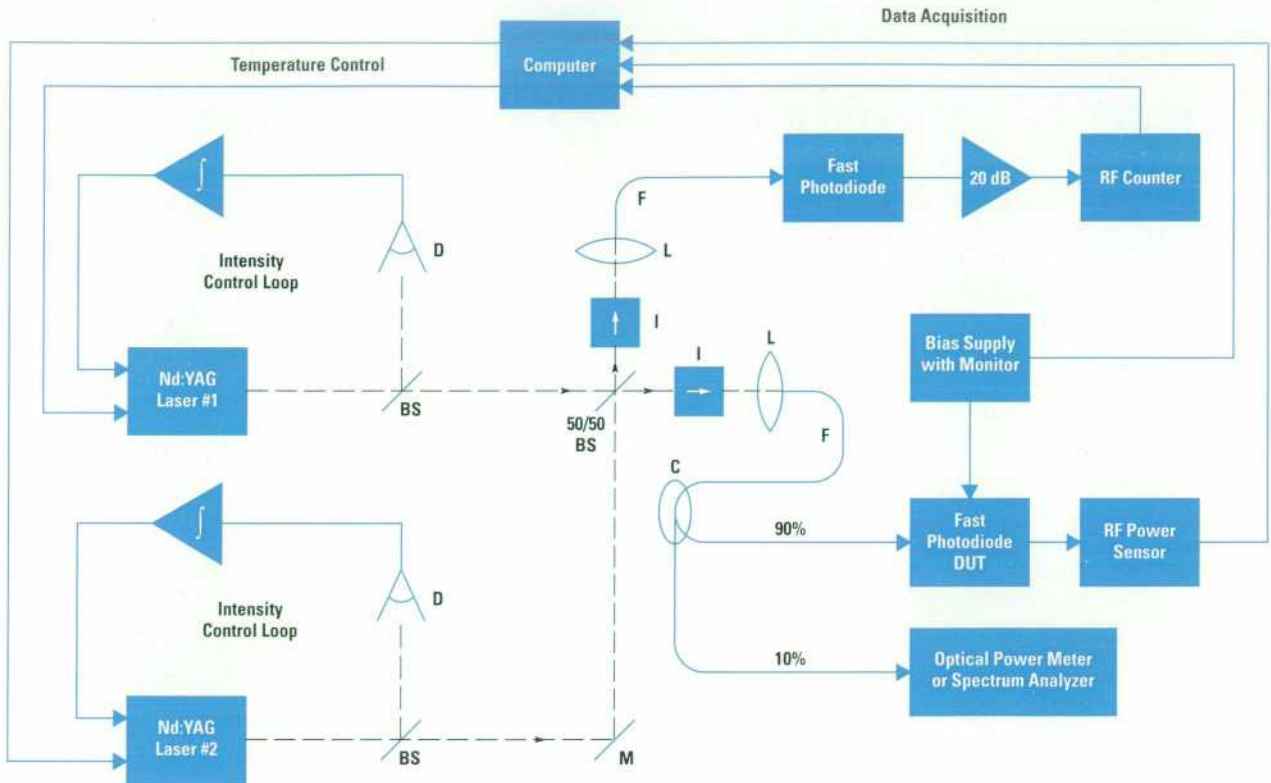
Fig. 1. NIST Nd:YAG heterodyne system. Labeled components are the beam splitter (BS), mirror (M), isolator (I), lens (L), single mode fiber (F), large-area detector (D), and integrating amplifier (∫).
