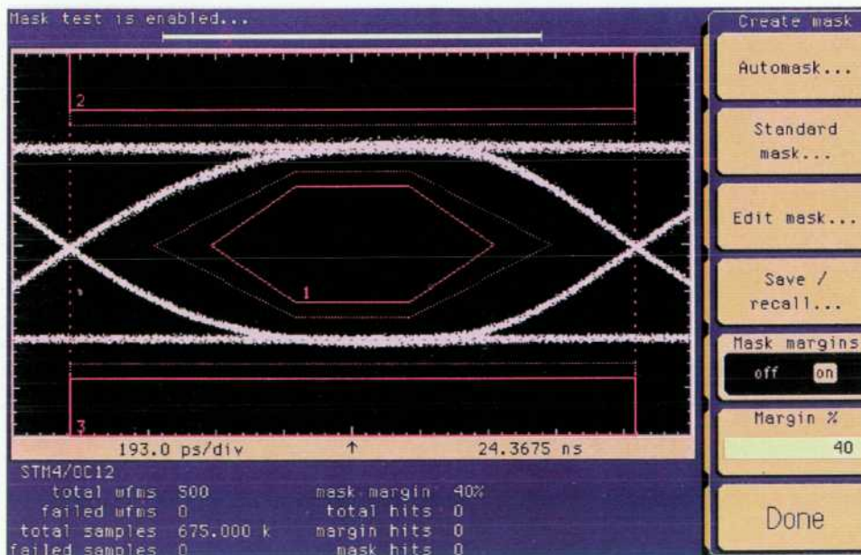
Fig. 9. Mask margins are used to add guardbands for production testing. In this example a 40% margin has been added to an industry-standard OC-12 mask at 622.08 Mbits/s.
