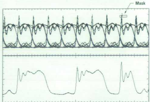
Fig. 4. Error trace capture using HP Eyeline mode. The upper trace shows the complete eye diagram. The lower trace shows the bit pattern leading up to a mask violation. A custom mask was constructed to capture only those waveforms showing extreme overshoot.
