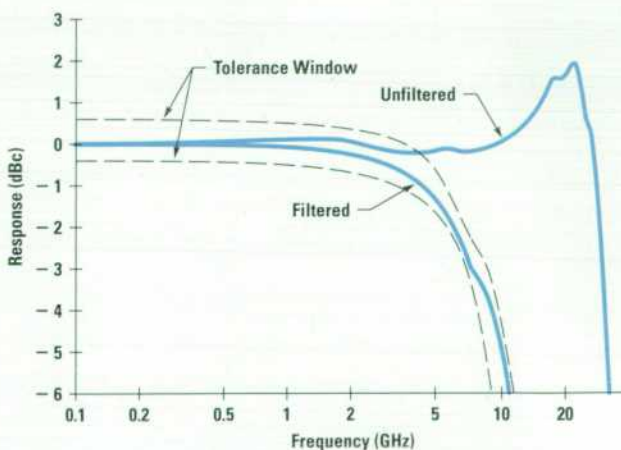
Fig. 5. Measured frequency responses of the HP 83480 digital communications analyzer with HP 83485B plug-in module.
