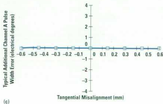
Fig. 7. Performance curves for the 75-line-per-inch encoder.
