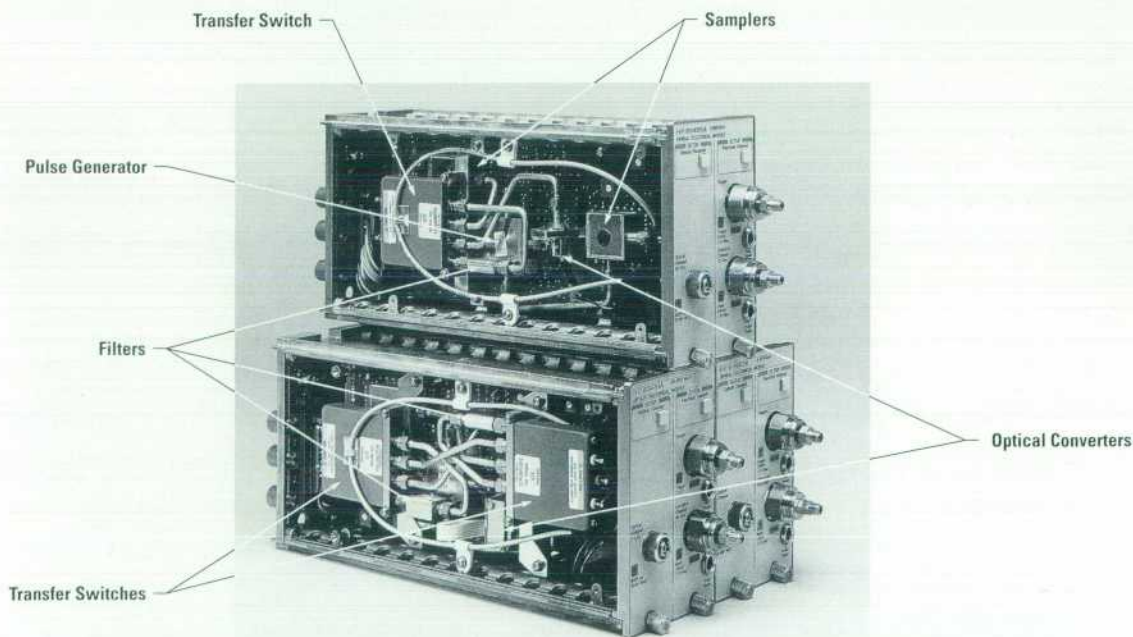
Fig. 3. Three optical-to-electrical plug-in modules are available.
