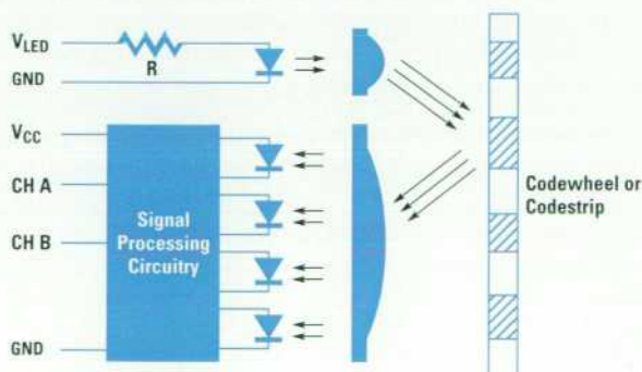
Fig. 3. HEDR-8000 Series encoder block diagram.
