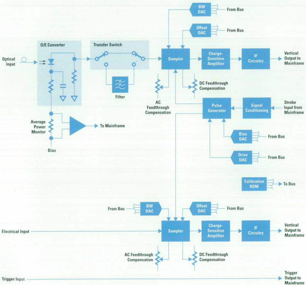
Fig. 1. Generalized HP 83480 plug-in module block diagram.
