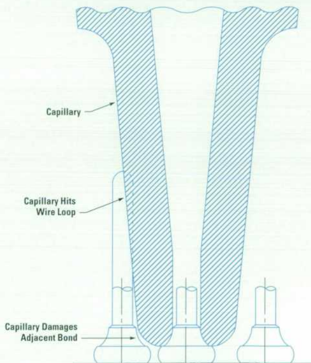
Fig. 1. Capillary interference.
