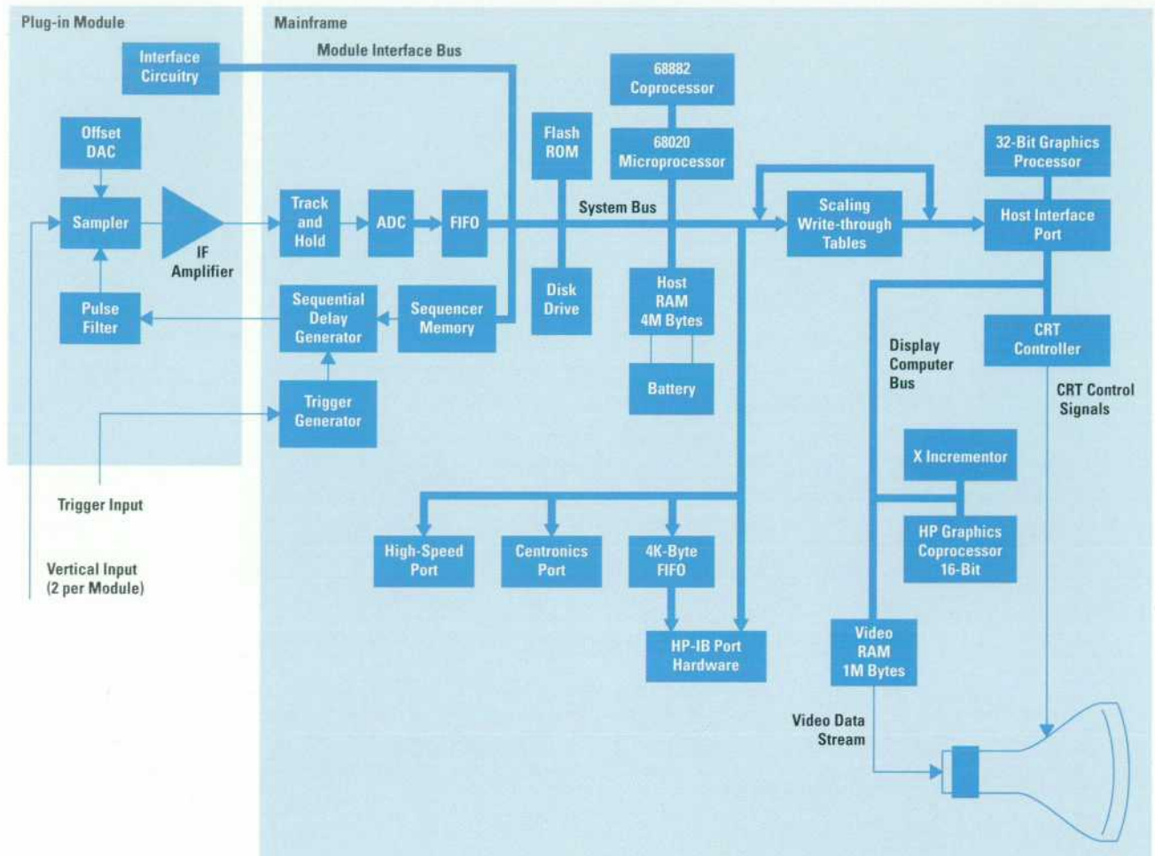
Fig. 5. HP 83480 hardware block diagram.
