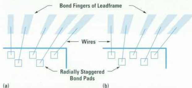
Fig. 7. Effects on angle of approach of two different bond pad layouts corresponding to two distinct choices of convergence point. The angle of approach is the angle between the wire trajectory and the bonding finger. (a) Convergence point at the geometric center of the die. (b) Convergence point far from the geometric center along the negative y-axis.
