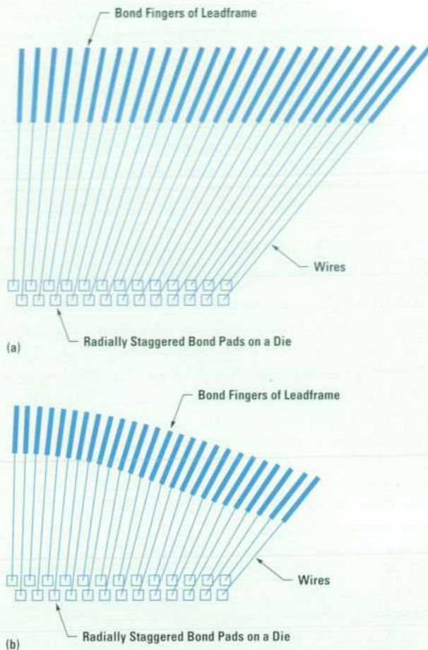
Fig. 13. Role of leadframe design in angle of approach and wire length reduction. (a) The angles of approach have been minimized. (b) The wire lengths have been minimized. In both cases, the leadframe design rules (minimum width and spacing of leads) are the same.
