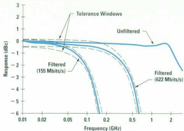
Fig. 7. Measured frequency responses of the HP 83480 digital communications analyzer with HP 83481A plug-in module.
