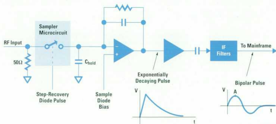
Fig. 2. Generalized sampler circuitry.
