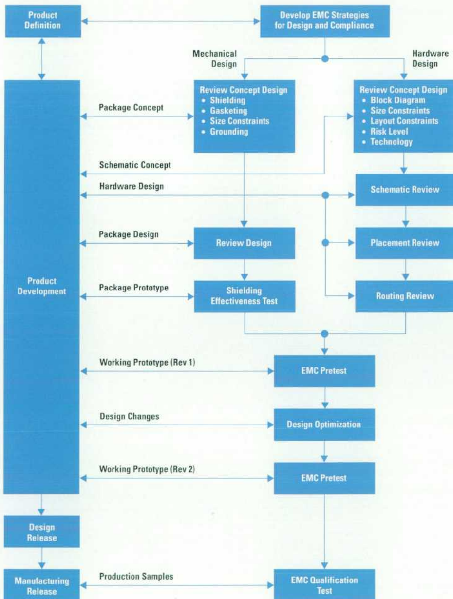
Fig. 1. EMC design process for the HP E5200A broadband service analyzer.
