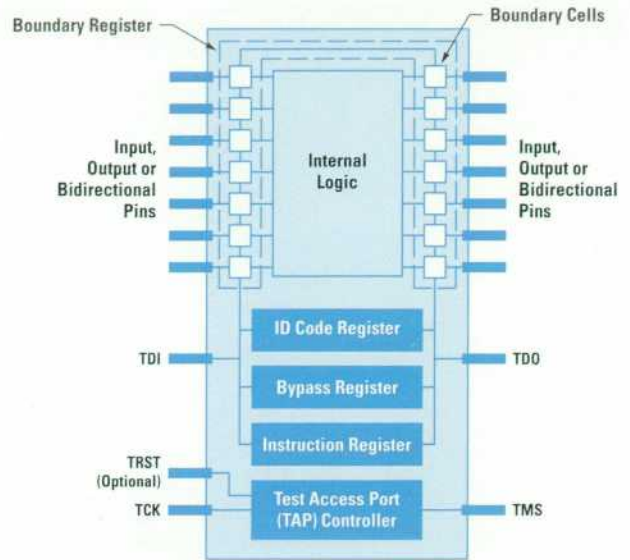
Fig. 2. Typical IEEE 1149.1-compliant device.
