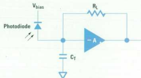
Fig. 3. Photodiode with transimpedance amplifier.
