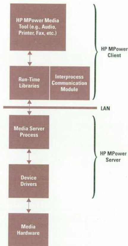
Fig. 5. The architecture for a distributed multimedia application.
