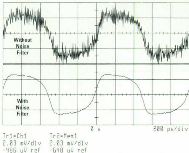
Fig. 10. Filtering the IF signal removes noise but retains the underlying wave shape.
