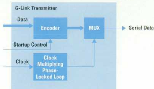
Fig. 2. Simplified transmitter chip block diagram.
