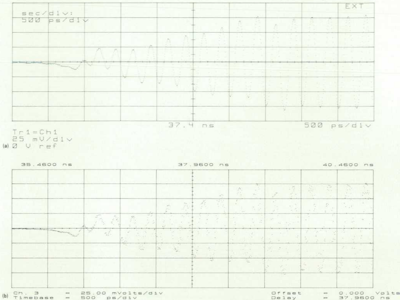
Fig. 12. Most digital signal processing algorithms require sampling the input signal at a uniform interval. (a) In the microwave transition analyzer, the sampler is driven at a synthesized rate, resulting in very precise sample timing. (b) Conventional sampling oscilloscopes rely on high-frequency trigger circuitry for timing accuracy, so the sampling interval can be considerably more uncertain.
