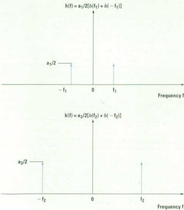
Fig. 2. Frequency-domain representation of the RF and LO signals.
