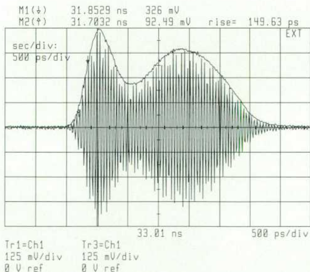
Fig. 3. The microwave transition analyzer can measure edge speeds on modulated waveforms as fast as 25 ps.
