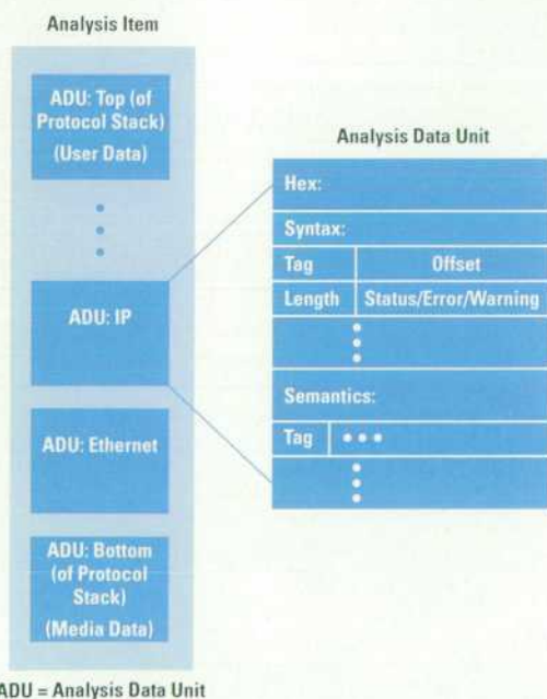
Fig. 6. An analysis item data structure.
