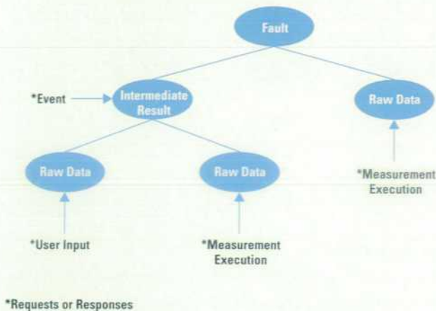
Fig. 6. Hierarchical data abstraction built by tracking requests and responses.
