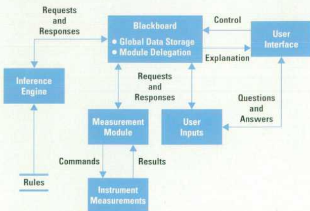
Fig. 5. The Fault Finder's architecture.
