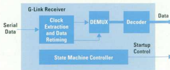
Fig. 4. Simplified receiver chip block diagram.
