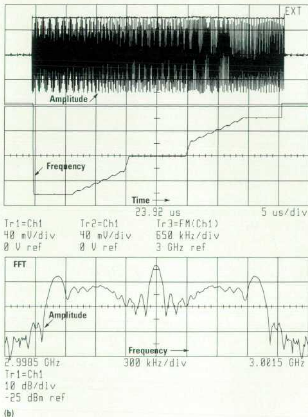
Fig. 1. Examples of complex modulation. (a) A phase coded RF pulse. The waveform and magnitude demodulation are shown in the upper half. The carrier's phase with respect to a CW reference is shown in the lower half. (b) Frequency modulation inside an RF pulse. The waveform and magnitude demodulation are shown at the top, the frequency demodulation is shown in the middle, and the magnitude spectrum of the pulse is shown at the bottom.
