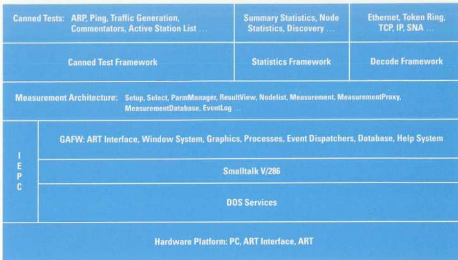
Fig. 3. The software architecture for the general-purpose environment. IEPC is the interenvironment process communication channel.
