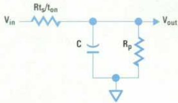
Fig. 6. Simplified sampler model.
