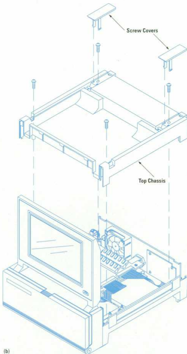
Fig. 6. (a) The bottom chassis of the Network Advisor. (b) The top chassis of the Network Advisor.
