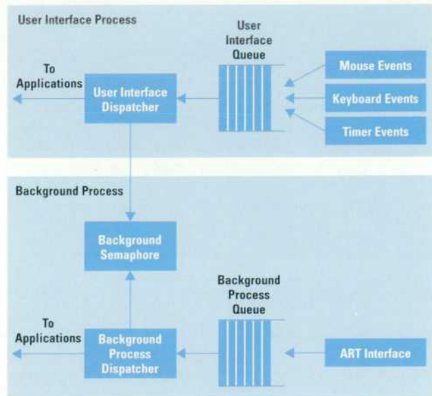
Fig. 6. Process model and dispatcher.
