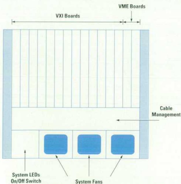
Fig. 5. HP E3560 peripheral unit cardcage organization.
