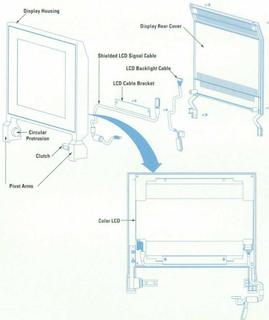
Fig. 2. Display housing and other components for the color LCD panel.
