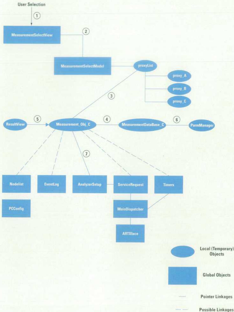
Fig. 5. Linkages and interactions when a measurement object (Measurement_Obj_C) is created to perform the measurement operations.
