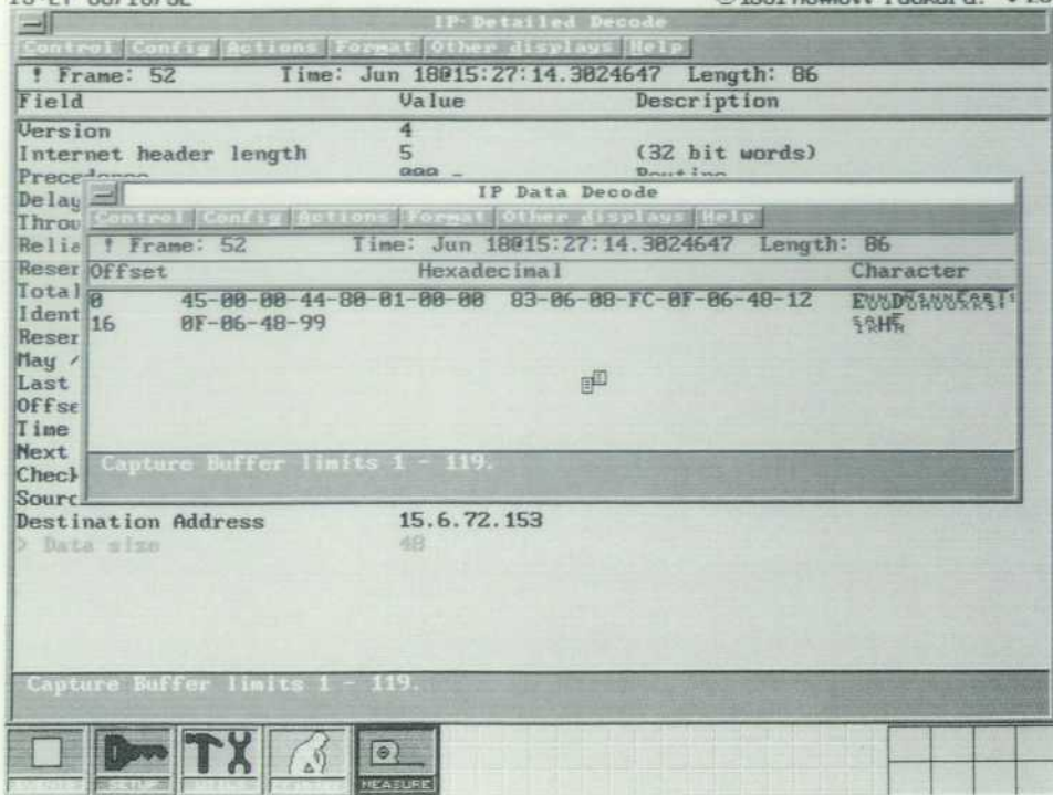
Fig. 5. Data view in hexadecimal format.
